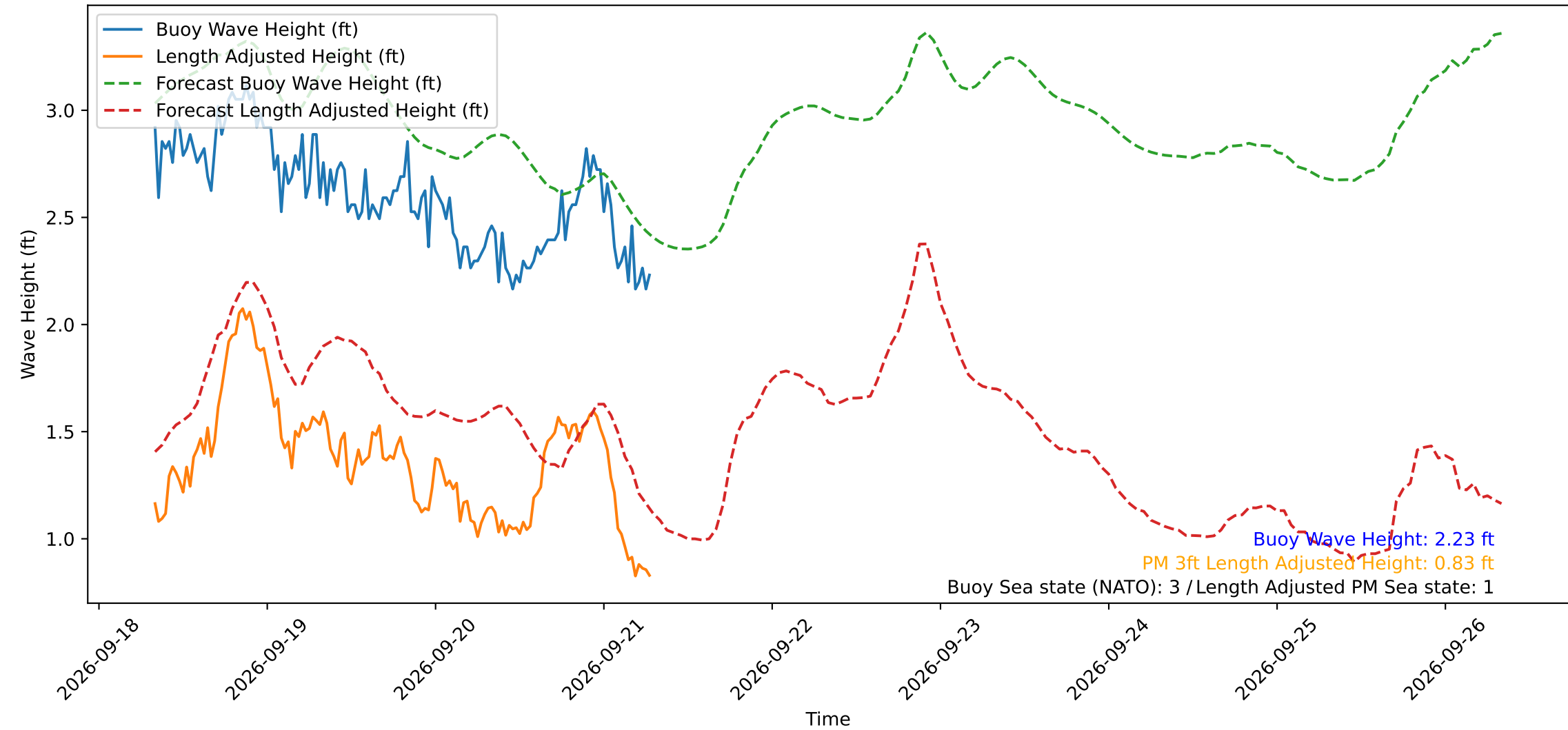
Wave Heights over Time for Green Beach at 2026-09-21 07:31:13
