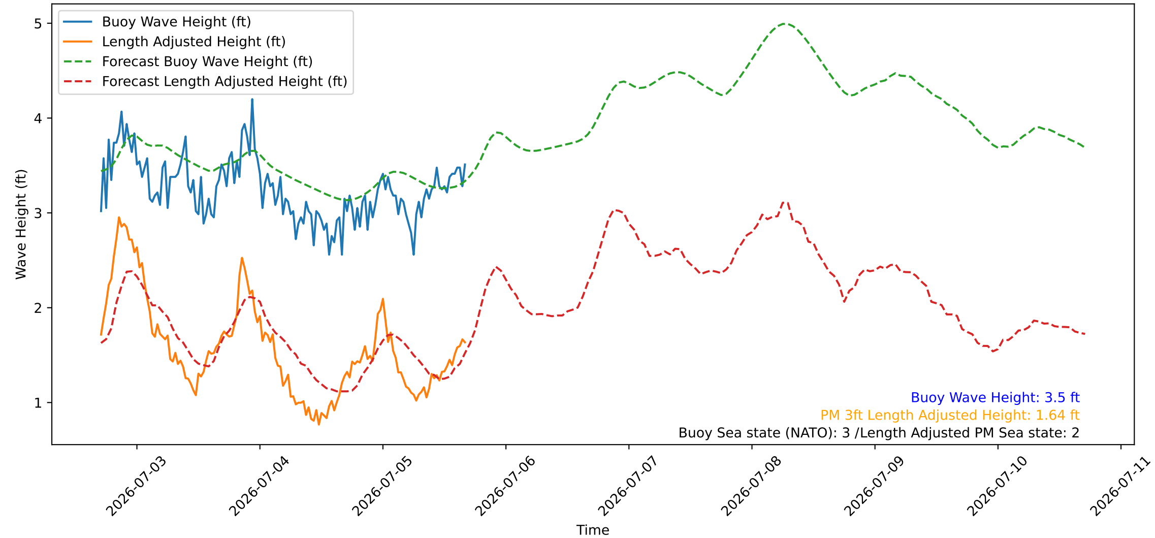
Wave Heights over Time for Green Beach at 2026-07-05 16:51:10
