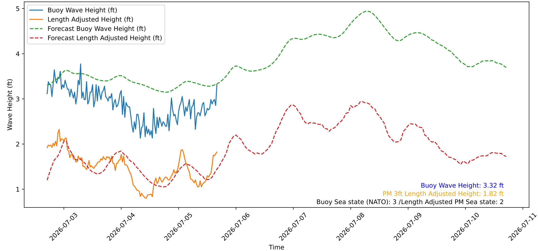
Wave Heights over Time for Oceanside Harbor at 2026-07-05 16:50:26
