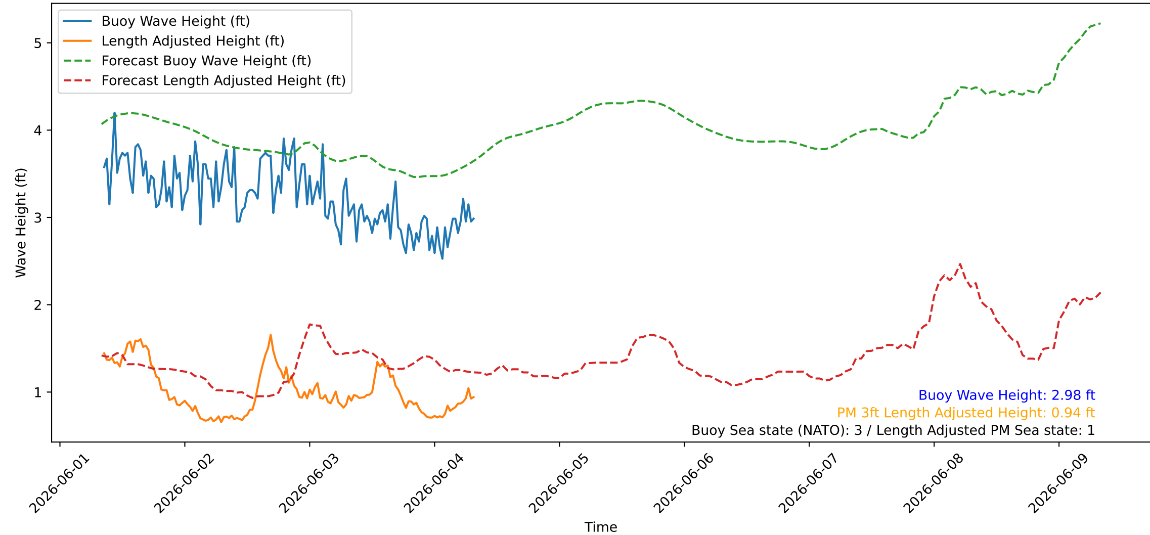
Wave Heights over Time for Red Beach at 2026-06-04 08:20:47
