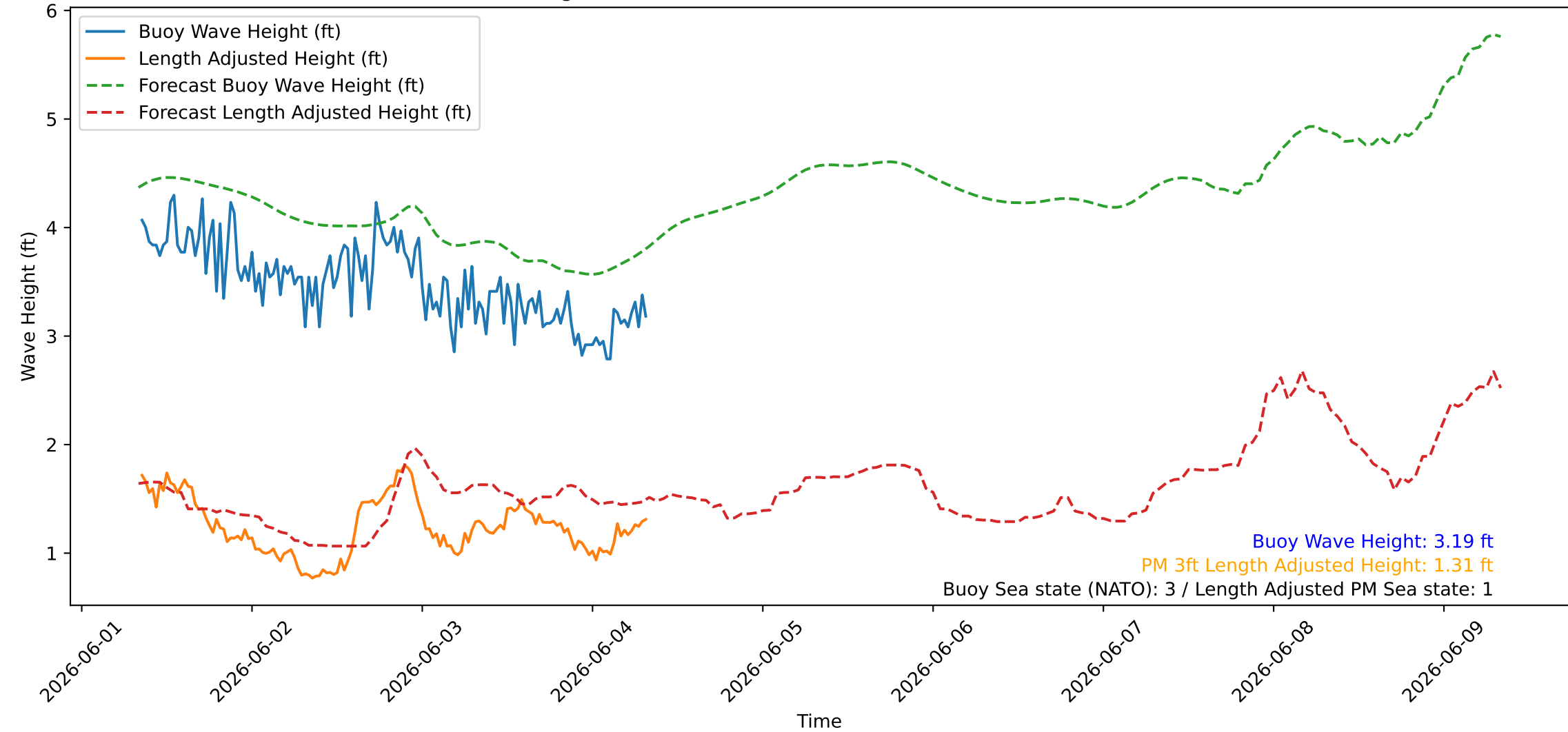
Wave Heights over Time for Green Beach at 2026-06-04 08:21:10
