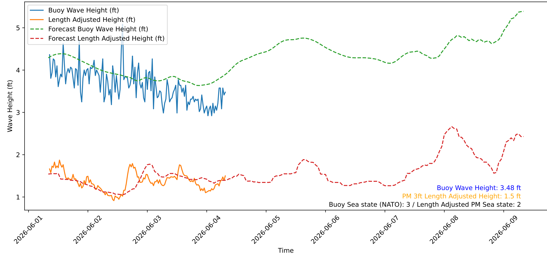
Wave Heights over Time for Oceanside Harbor at 2026-06-04 08:20:26
