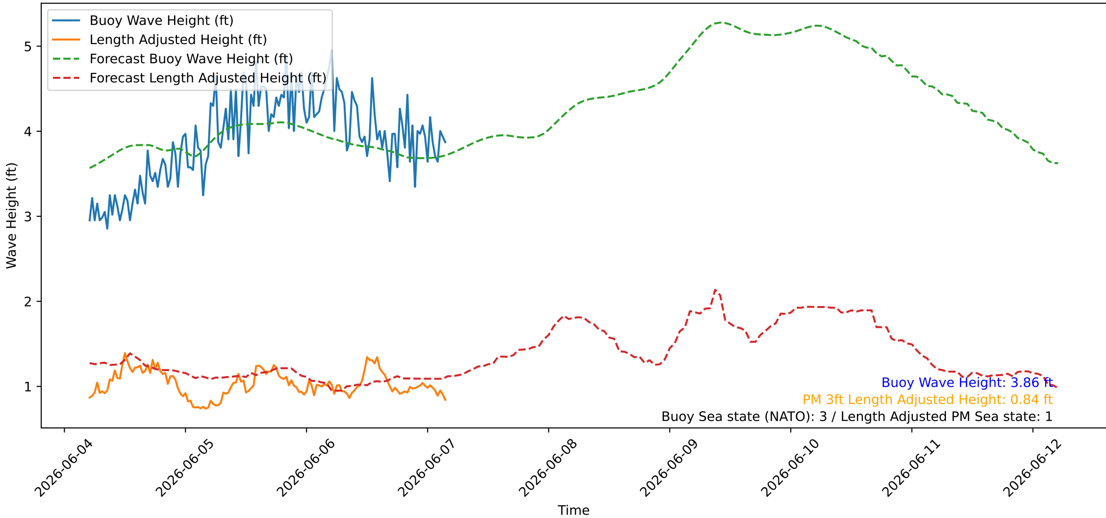
Wave Heights over Time for Red Beach at 2026-06-07 04:30:46
