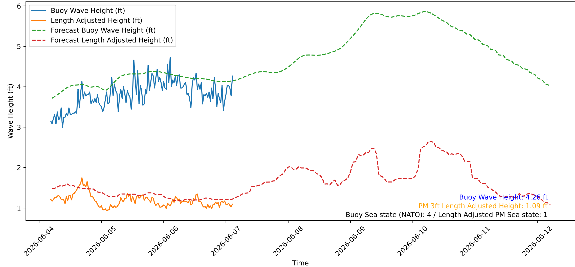
Wave Heights over Time for Green Beach at 2026-06-07 04:31:08
