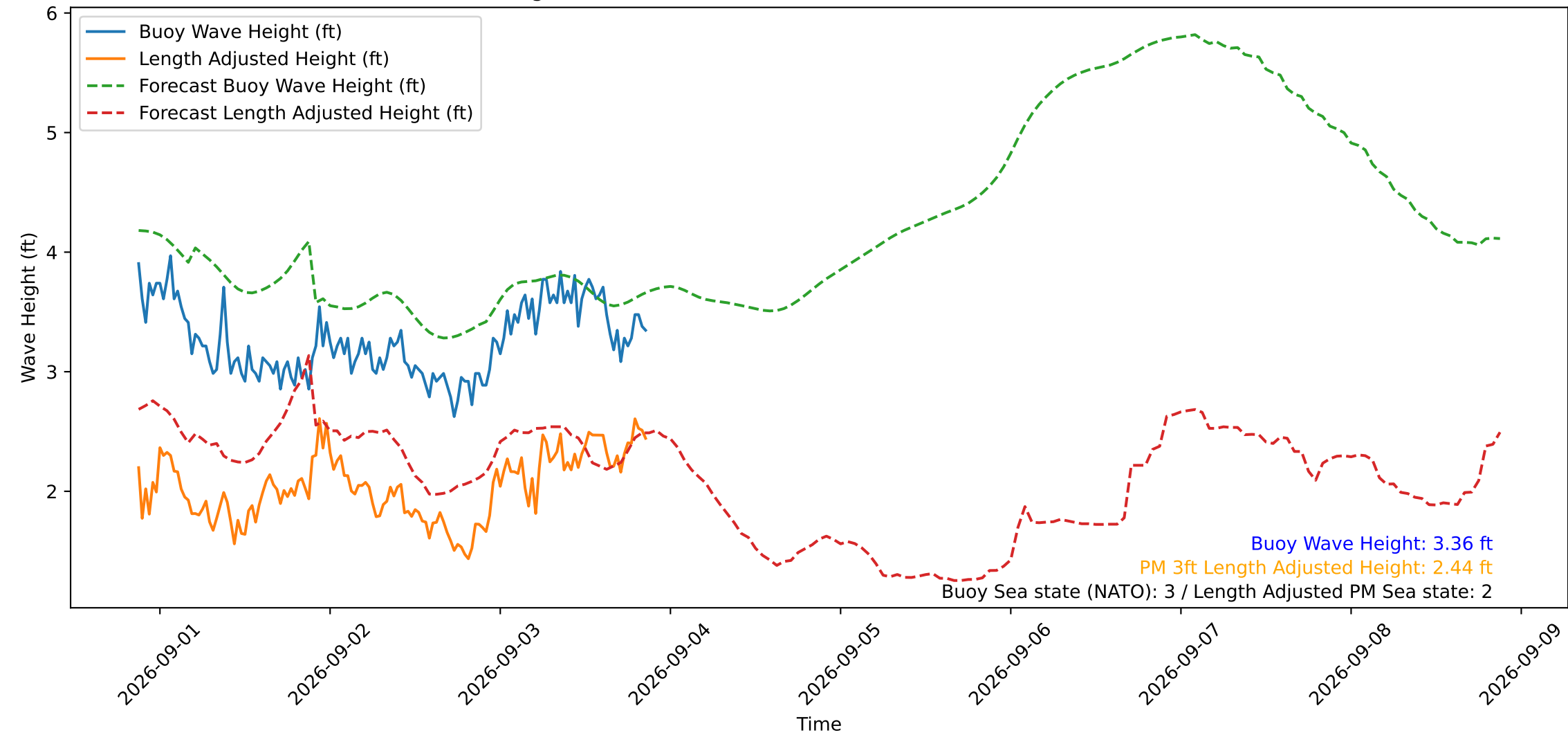
Wave Heights over Time for Oceanside Harbor at 2026-09-03 21:10:30
