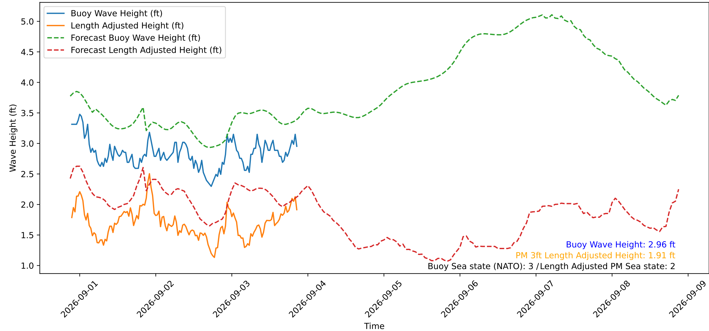
Wave Heights over Time for Red Beach at 2026-09-03 21:10:49
