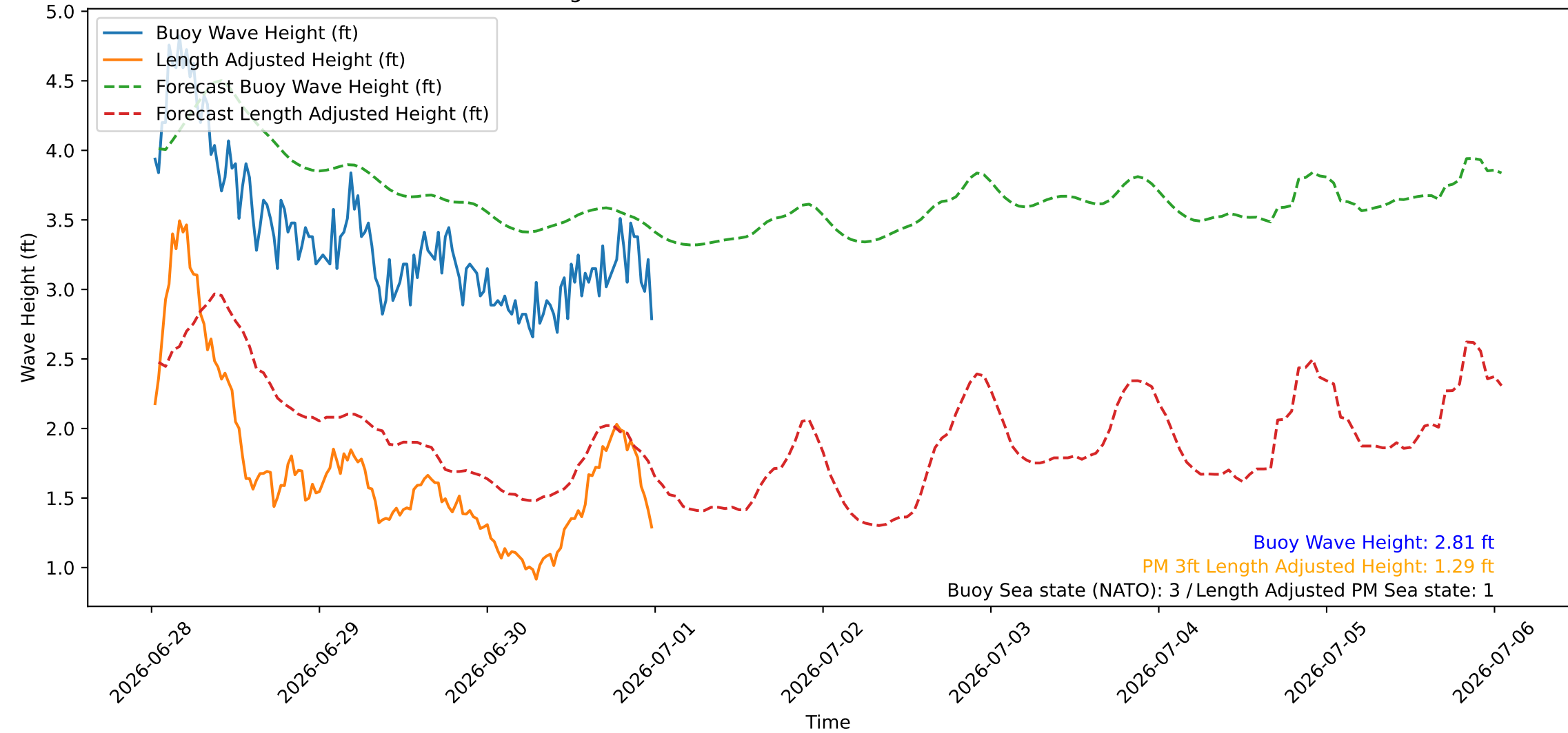
Wave Heights over Time for Green Beach at 2026-07-01 00:31:08
