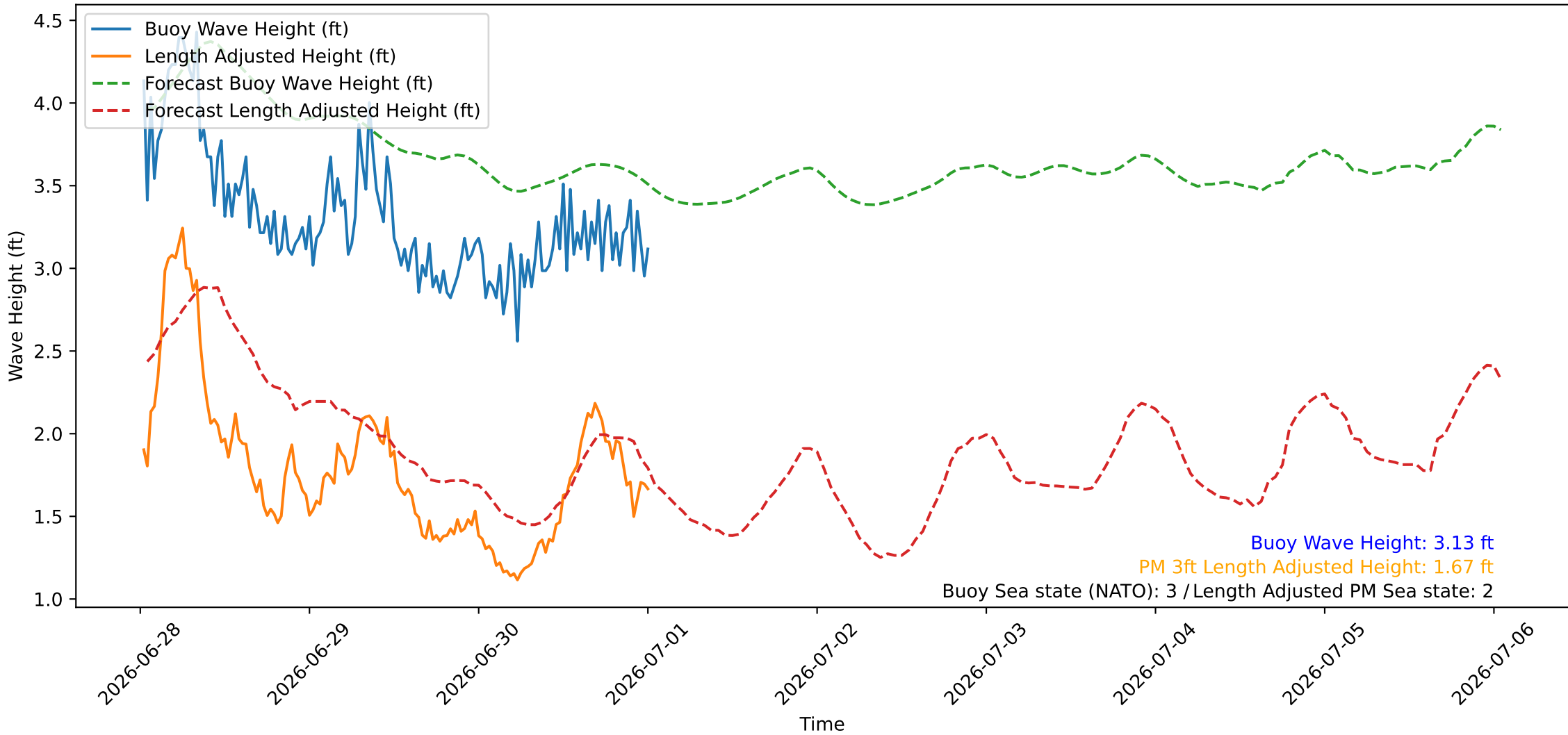
Wave Heights over Time for Oceanside Harbor at 2026-07-01 00:30:26
