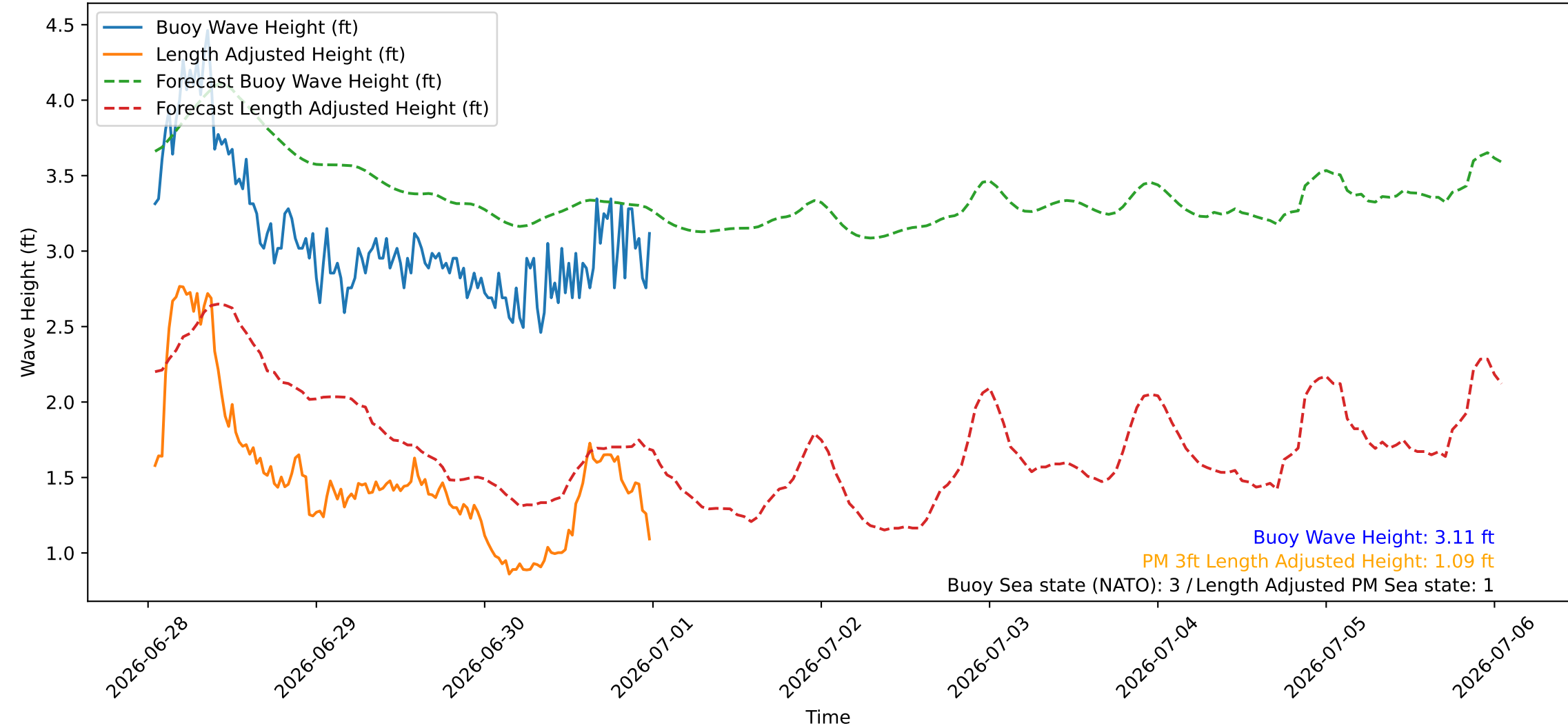
Wave Heights over Time for Red Beach at 2026-07-01 00:30:46
