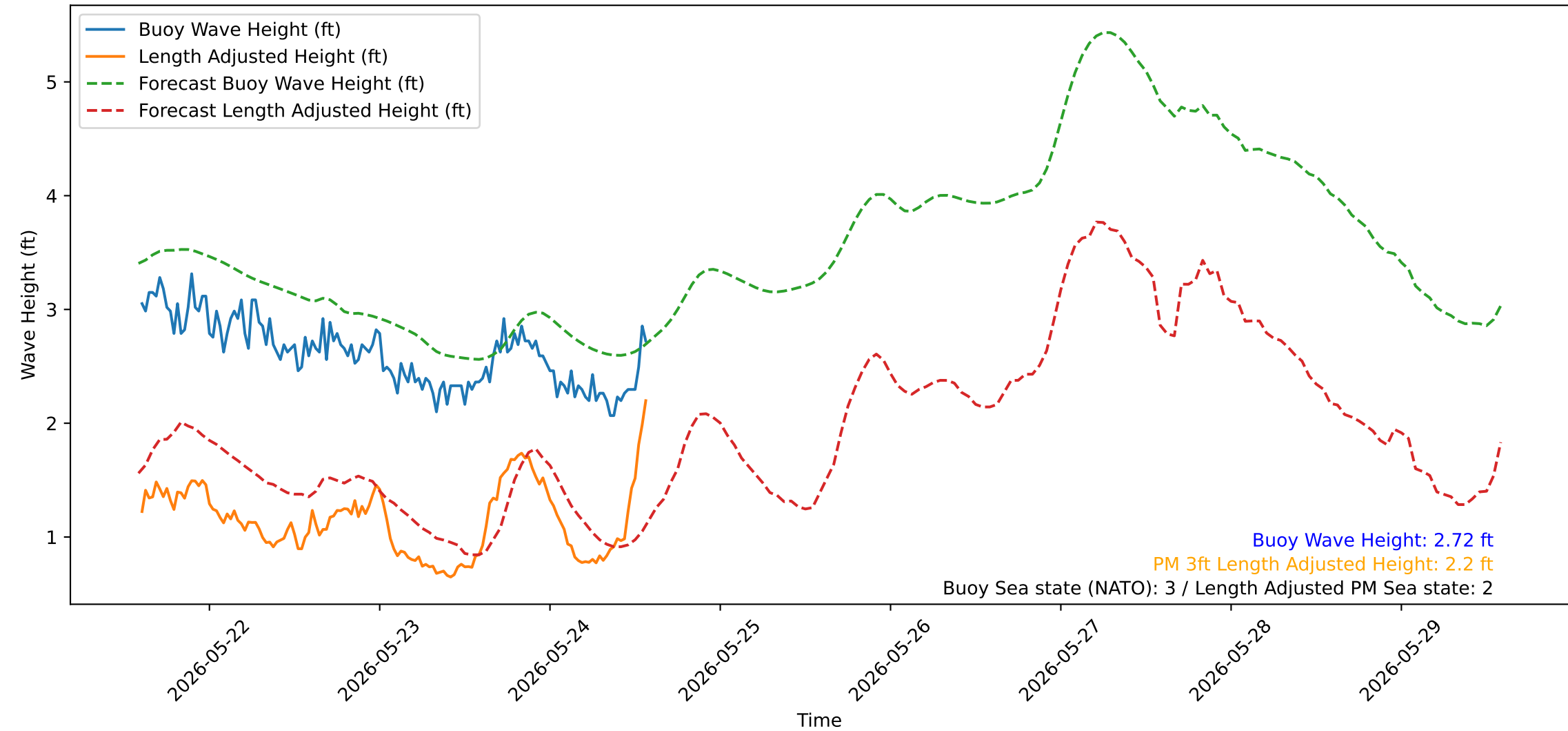
Wave Heights over Time for Green Beach at 2026-05-24 14:21:16
