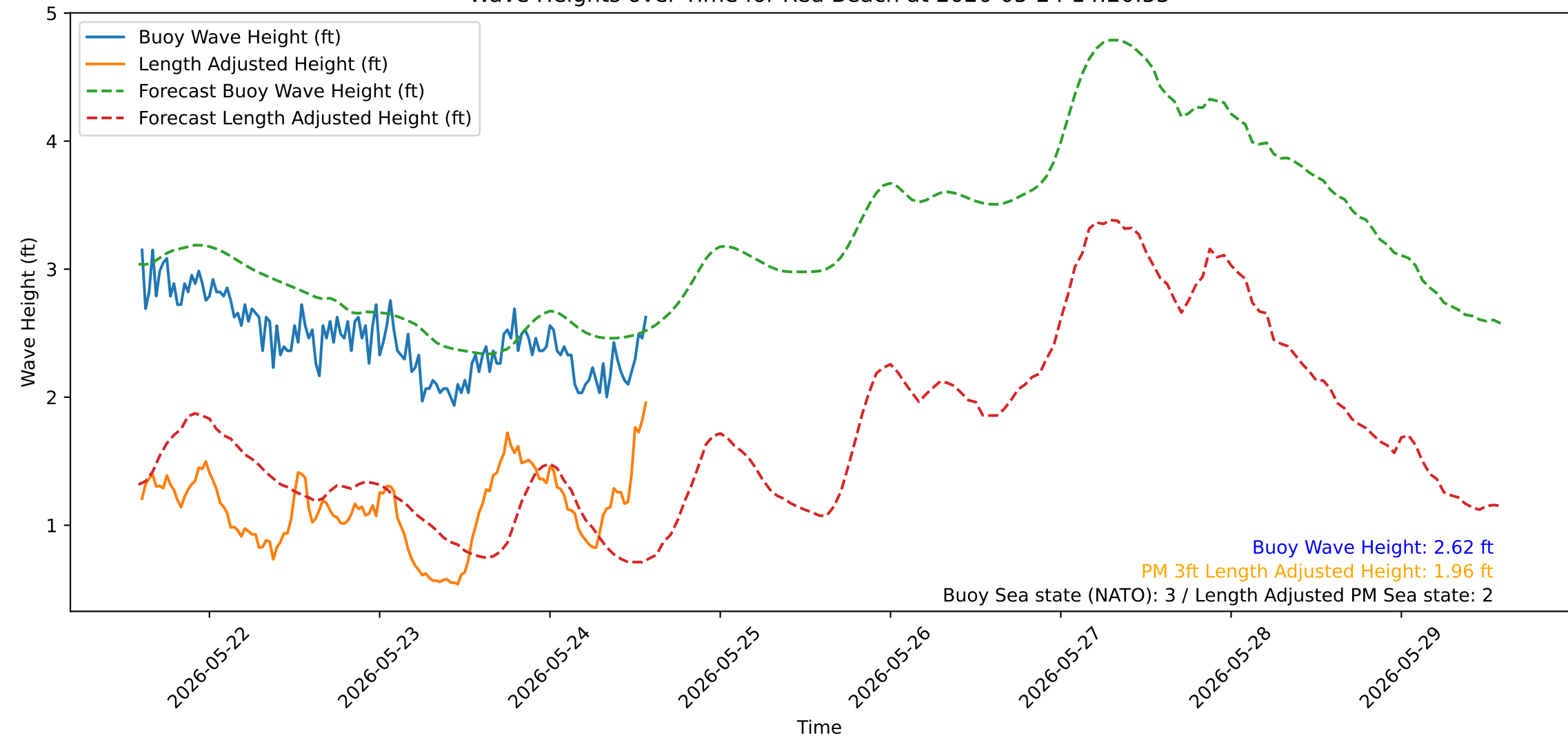
Wave Heights over Time for Red Beach at 2026-05-24 14:20:53
