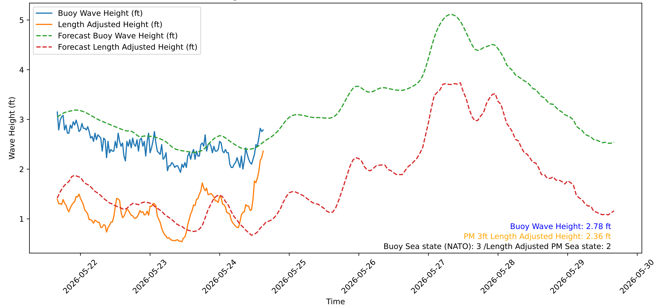
Wave Heights over Time for Red Beach at 2026-05-24 15:40:51
