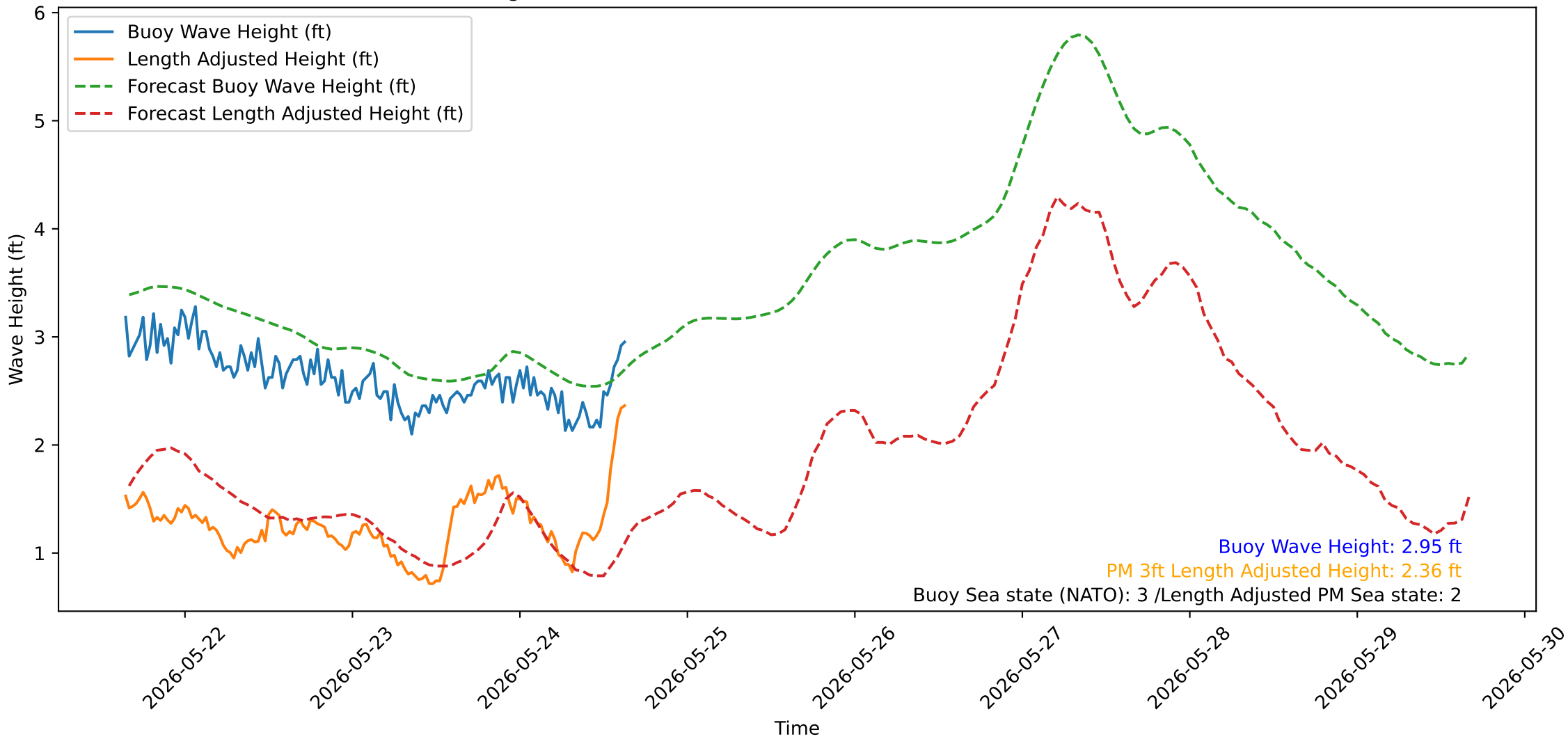
Wave Heights over Time for Oceanside Harbor at 2026-05-24 15:40:31
