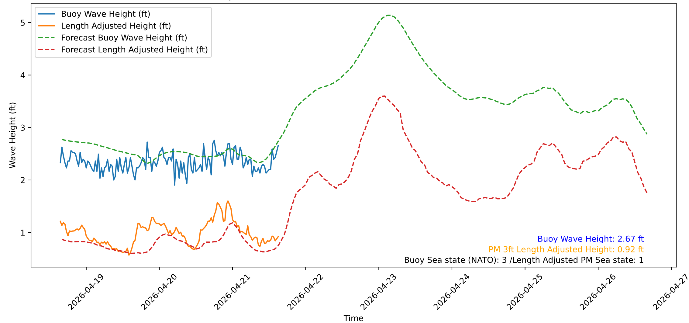
Wave Heights over Time for Oceanside Harbor at 2026-04-21 15:40:32
