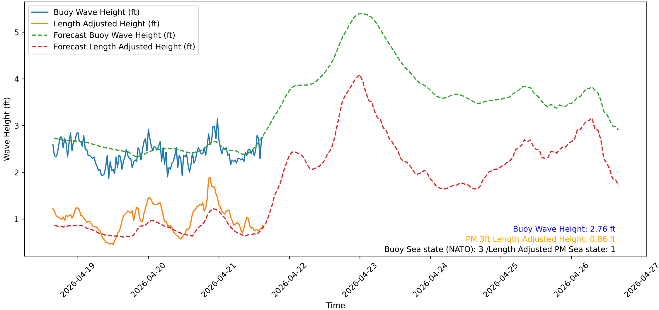
Wave Heights over Time for Green Beach at 2026-04-21 15:41:14
