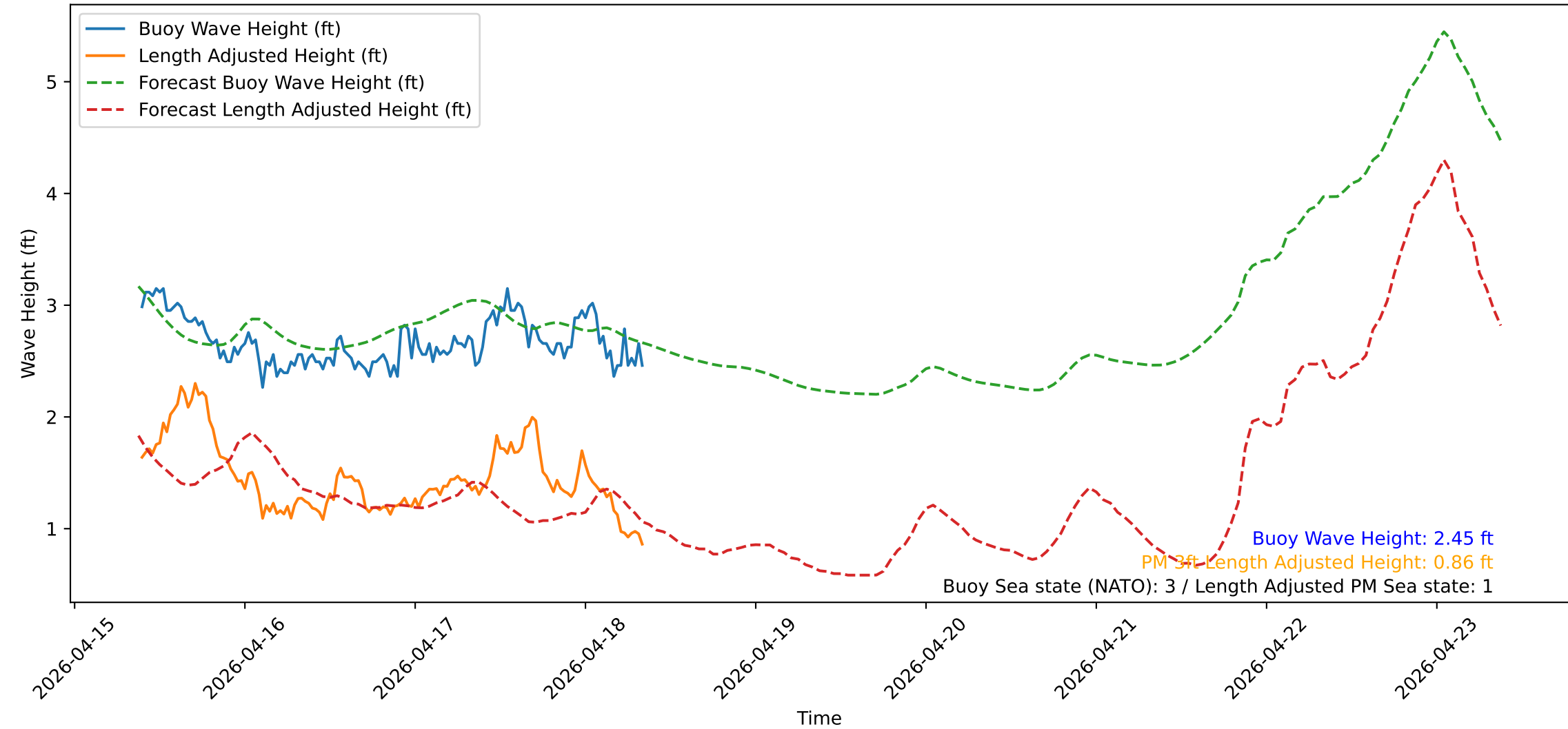
Wave Heights over Time for Red Beach at 2026-04-18 09:00:50
