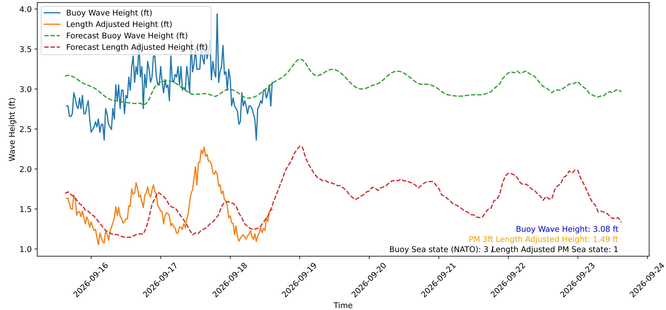
Wave Heights over Time for Oceanside Harbor at 2026-09-18 15:20:31
