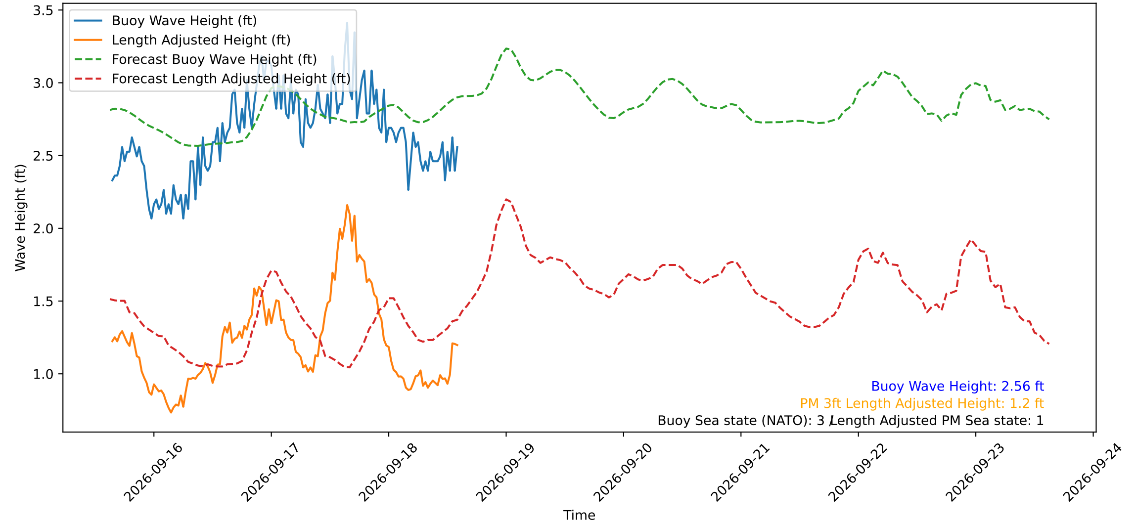
Wave Heights over Time for Red Beach at 2026-09-18 15:20:53
