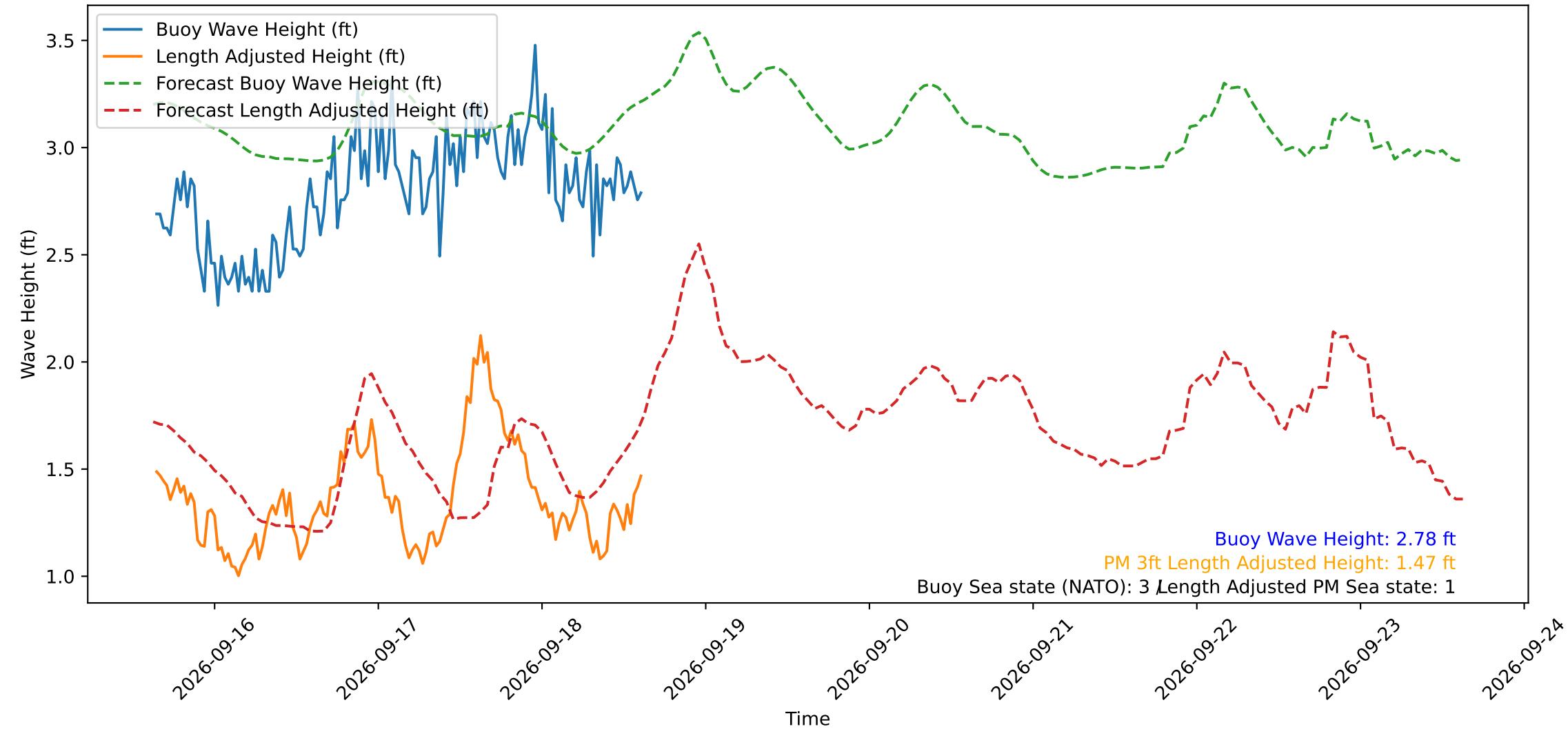
Wave Heights over Time for Green Beach at 2026-09-18 15:21:18
