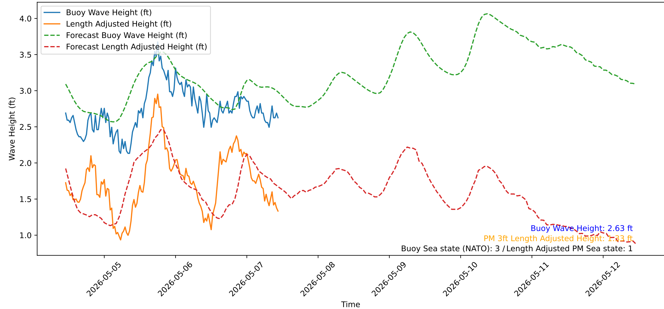
Wave Heights over Time for Green Beach at 2026-05-07 11:11:12
