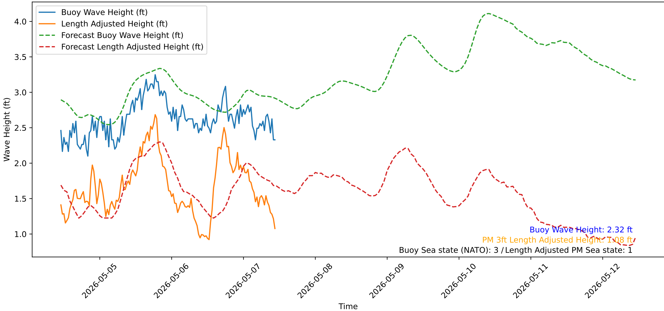
Wave Heights over Time for Oceanside Harbor at 2026-05-07 11:10:31
