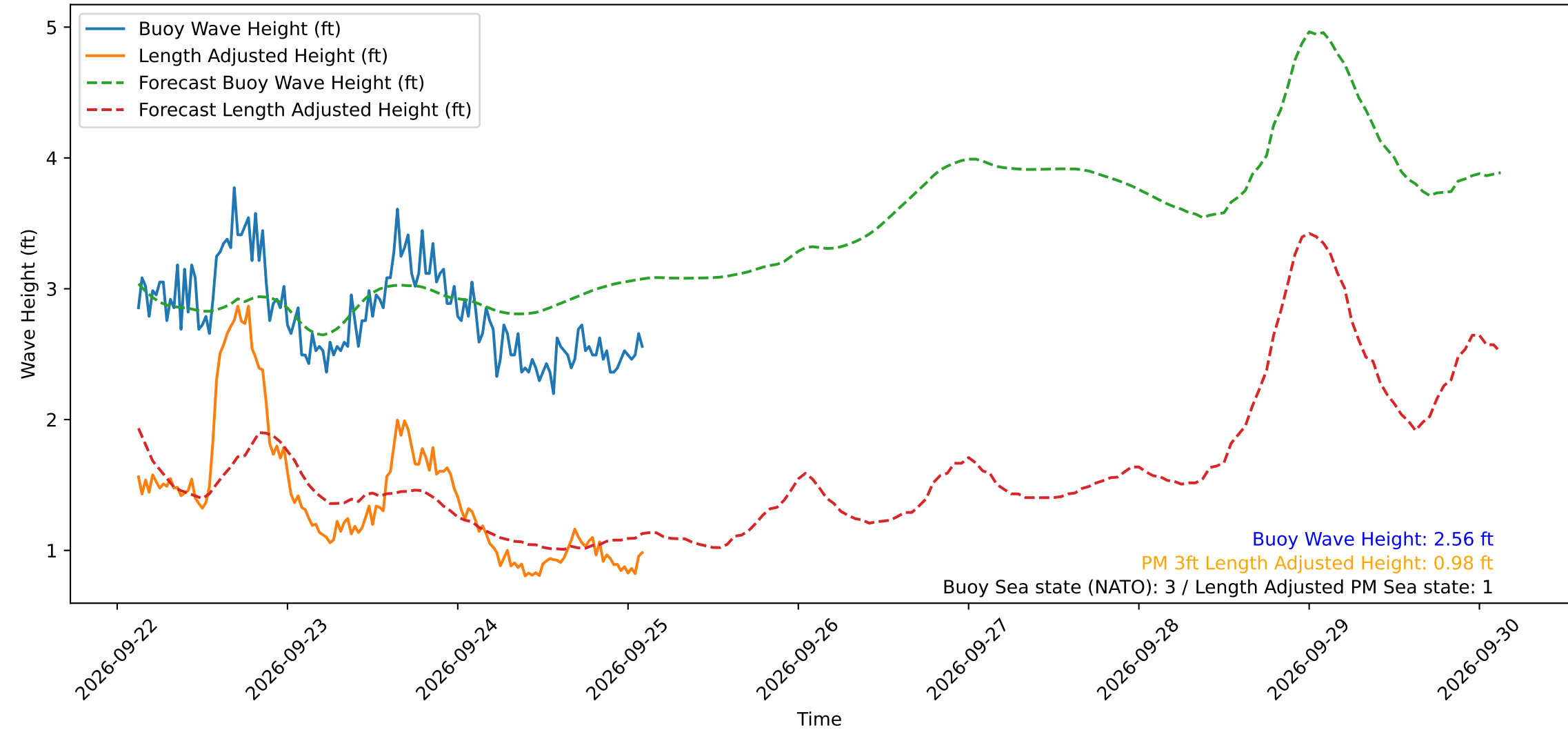
Wave Heights over Time for Oceanside Harbor at 2026-09-25 02:50:30
