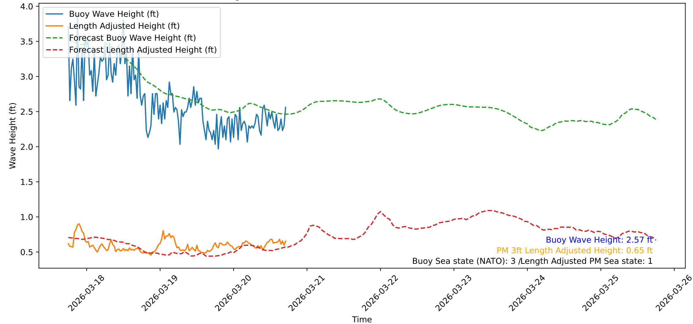
Wave Heights over Time for Oceanside Harbor at 2026-03-20 17:50:31
