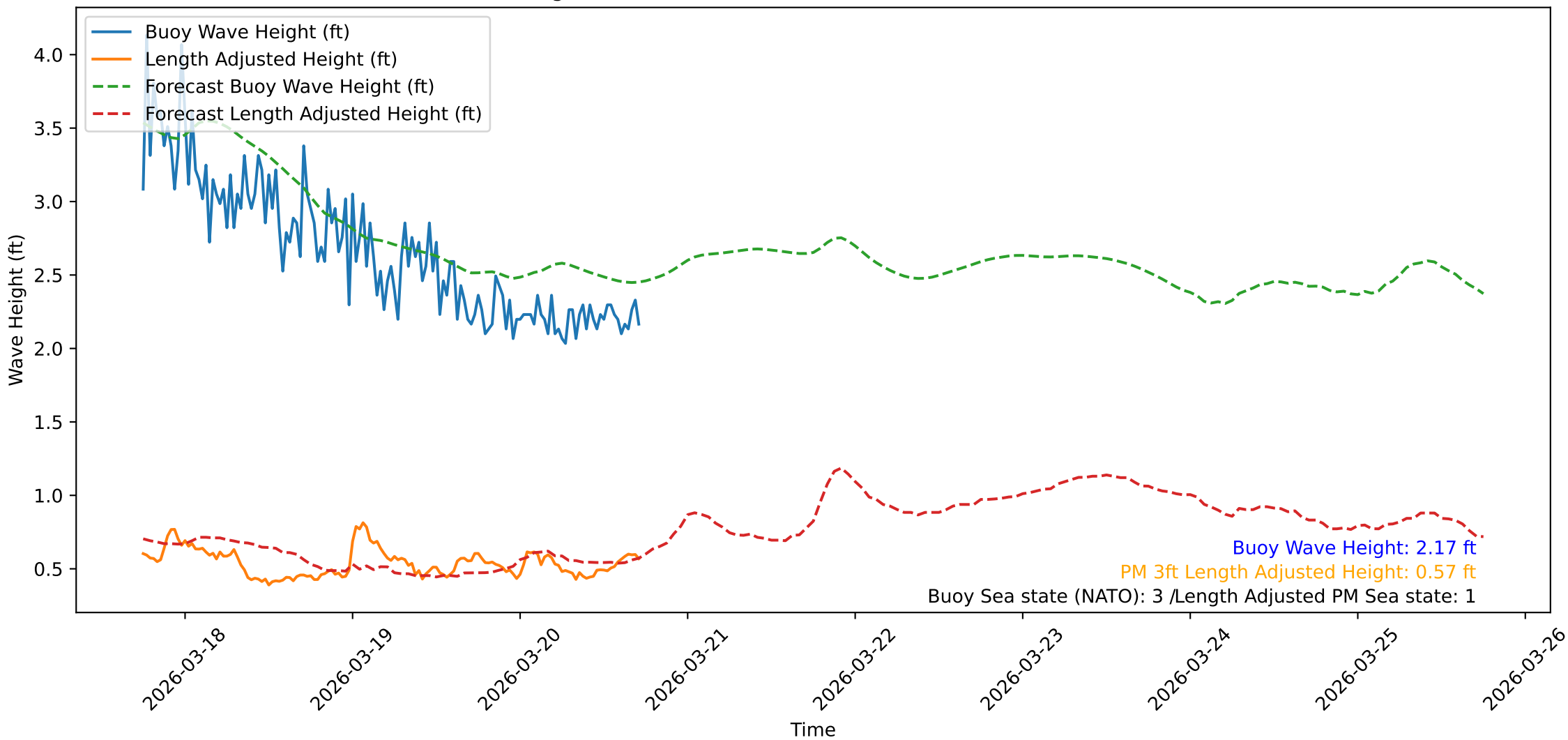
Wave Heights over Time for Green Beach at 2026-03-20 17:51:09
