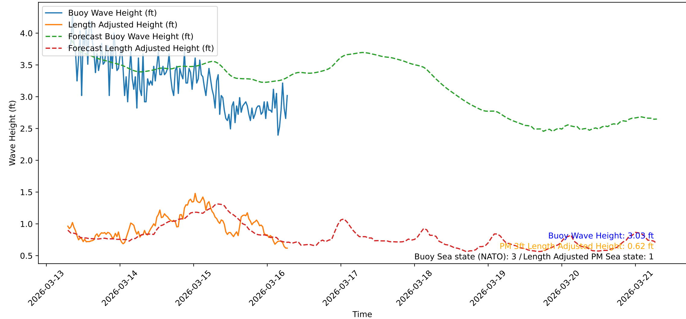
Wave Heights over Time for Oceanside Harbor at 2026-03-16 07:10:42
