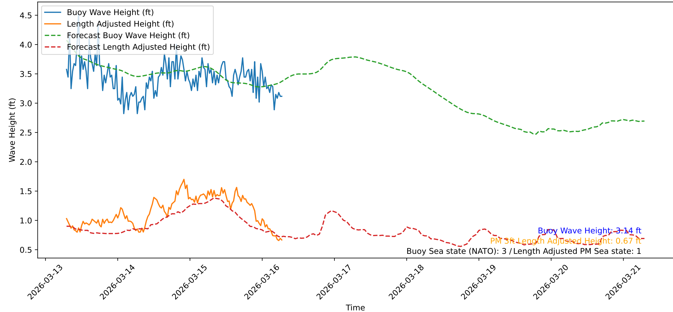
Wave Heights over Time for Green Beach at 2026-03-16 07:11:37
