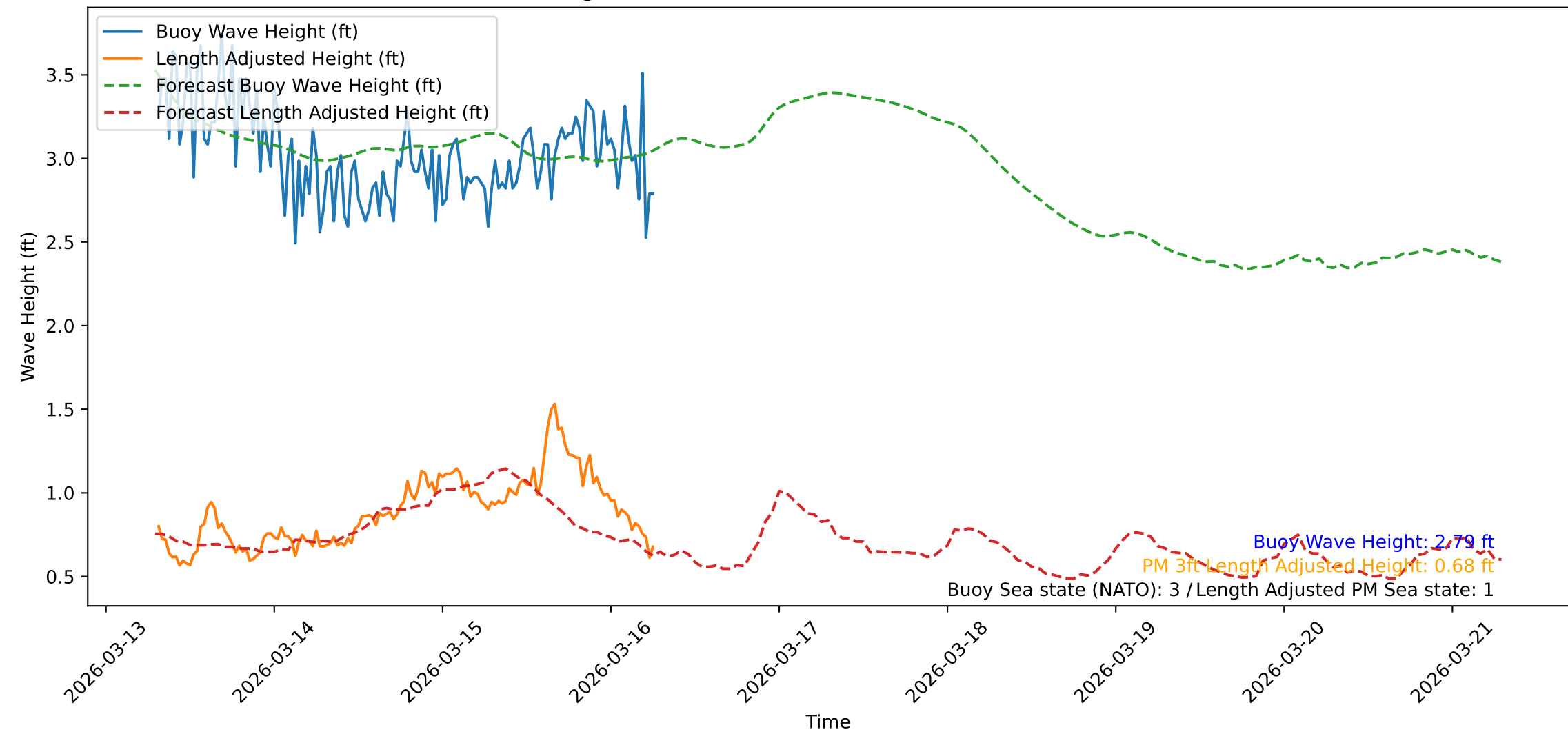
Wave Heights over Time for Red Beach at 2026-03-16 07:11:02
