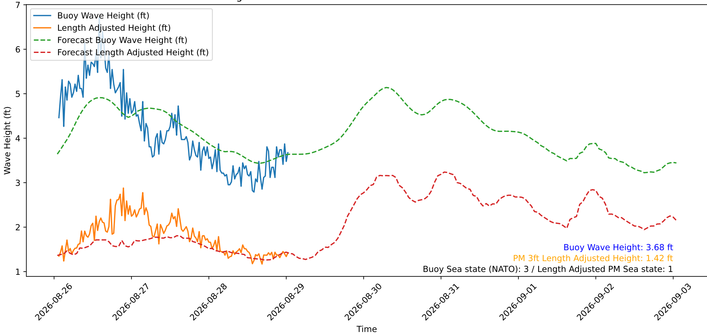
Wave Heights over Time for Oceanside Harbor at 2026-08-29 01:20:29
