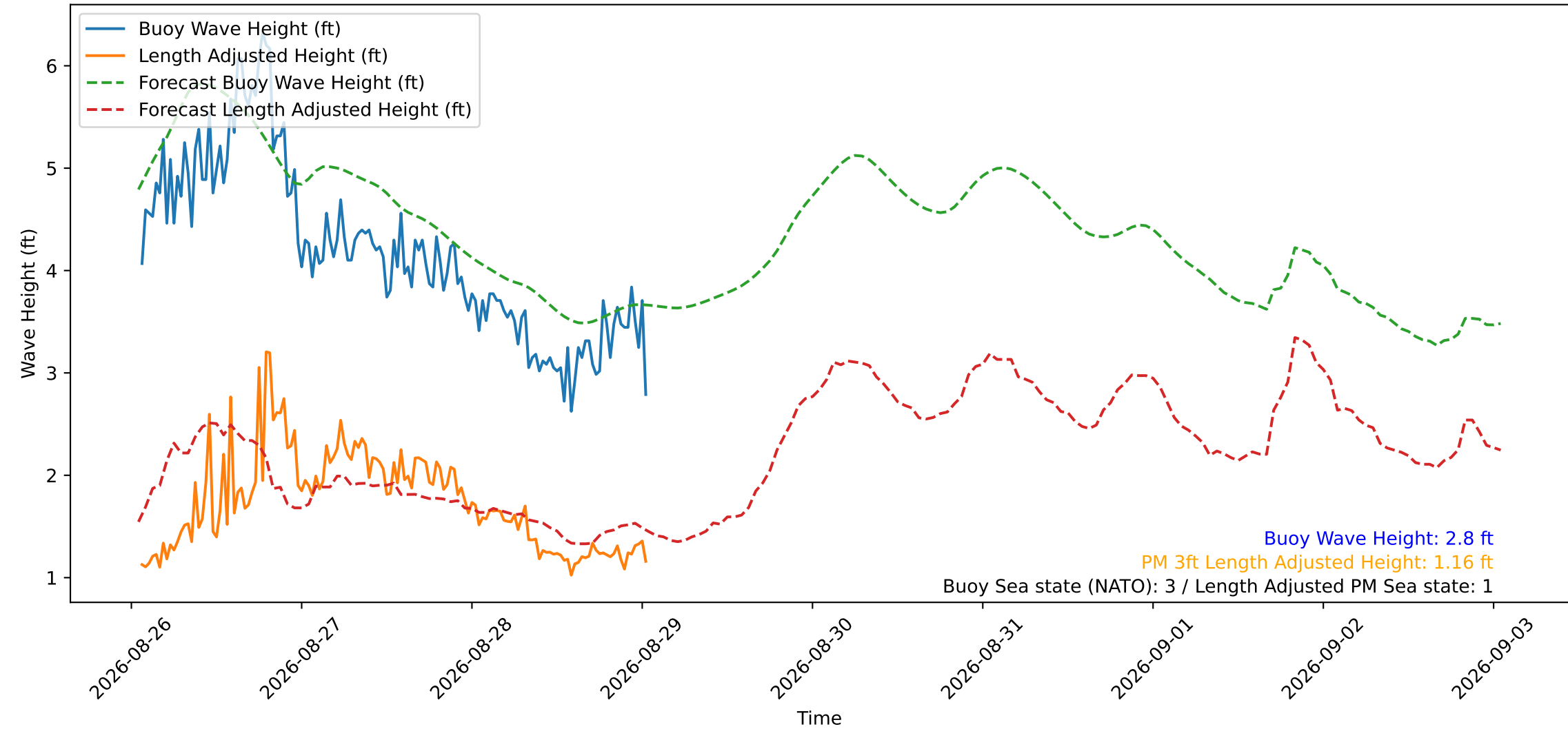
Wave Heights over Time for Green Beach at 2026-08-29 01:21:14
