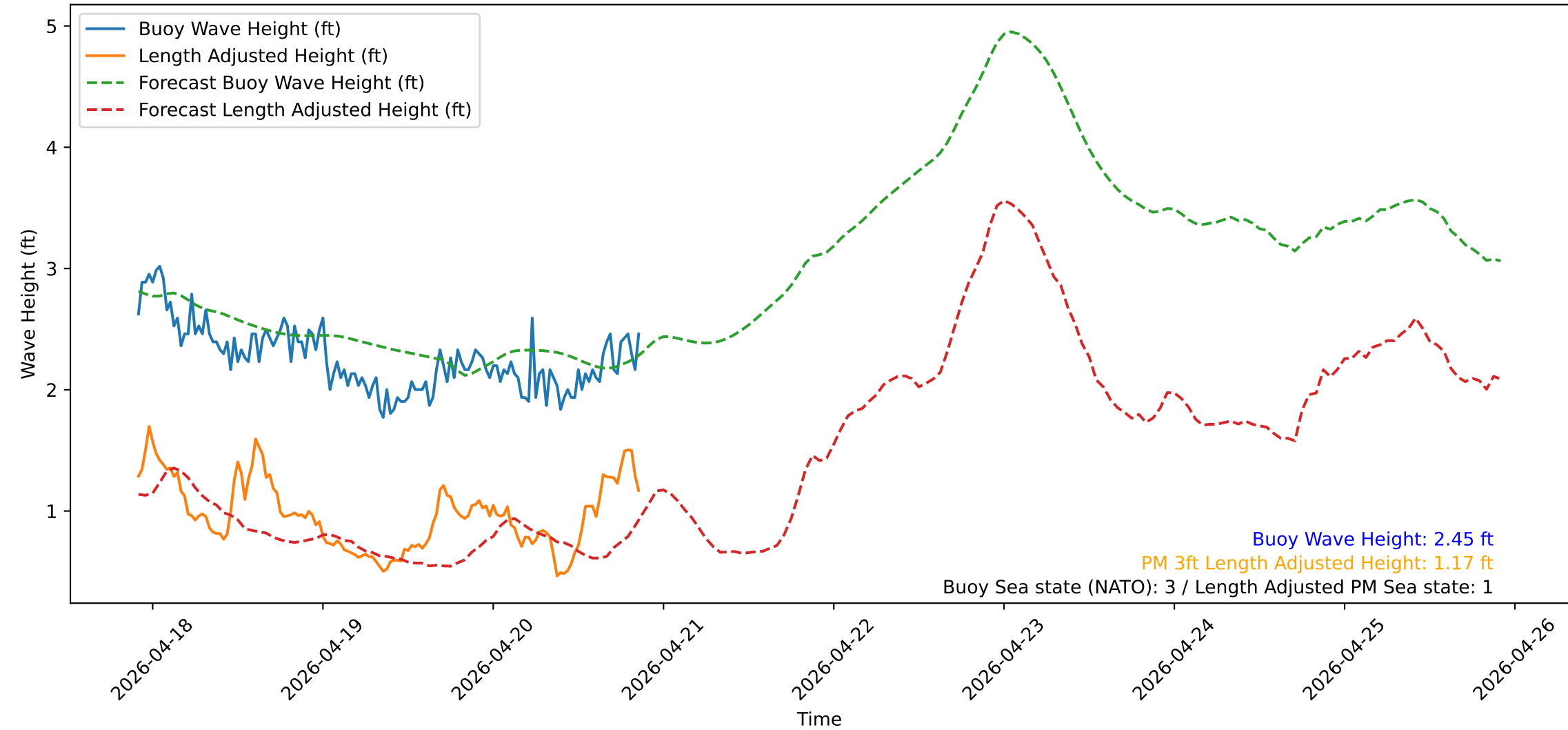
Wave Heights over Time for Red Beach at 2026-04-20 21:30:51
