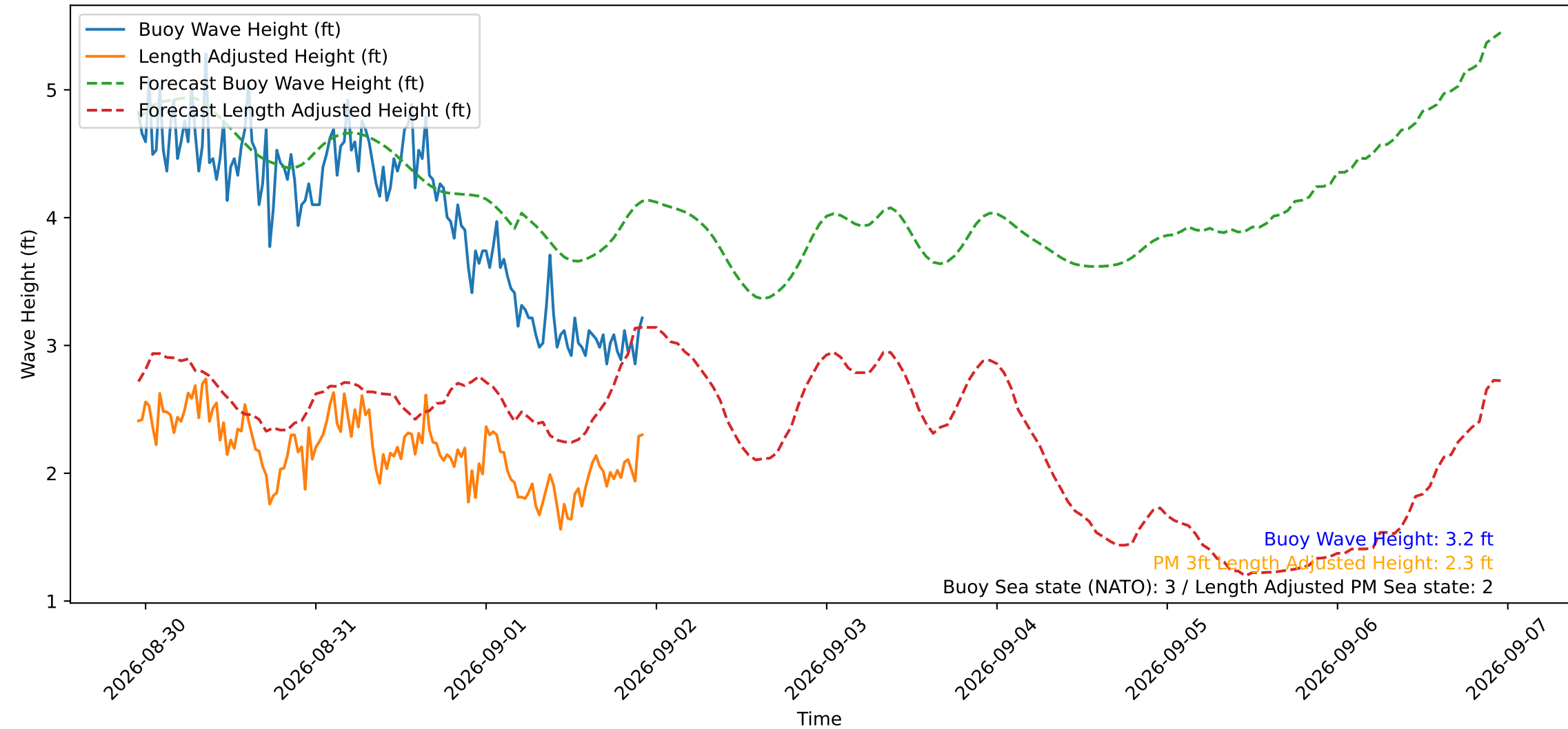
Wave Heights over Time for Oceanside Harbor at 2026-09-01 22:50:30
