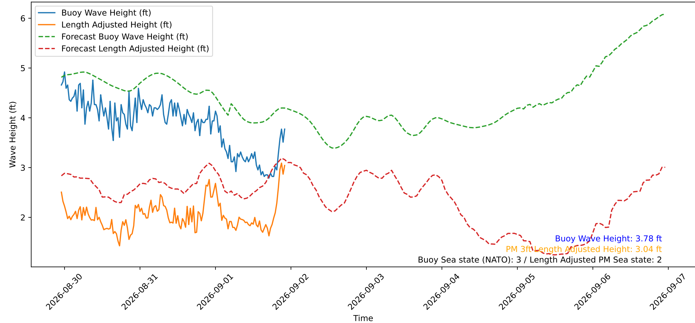
Wave Heights over Time for Green Beach at 2026-09-01 22:51:14
