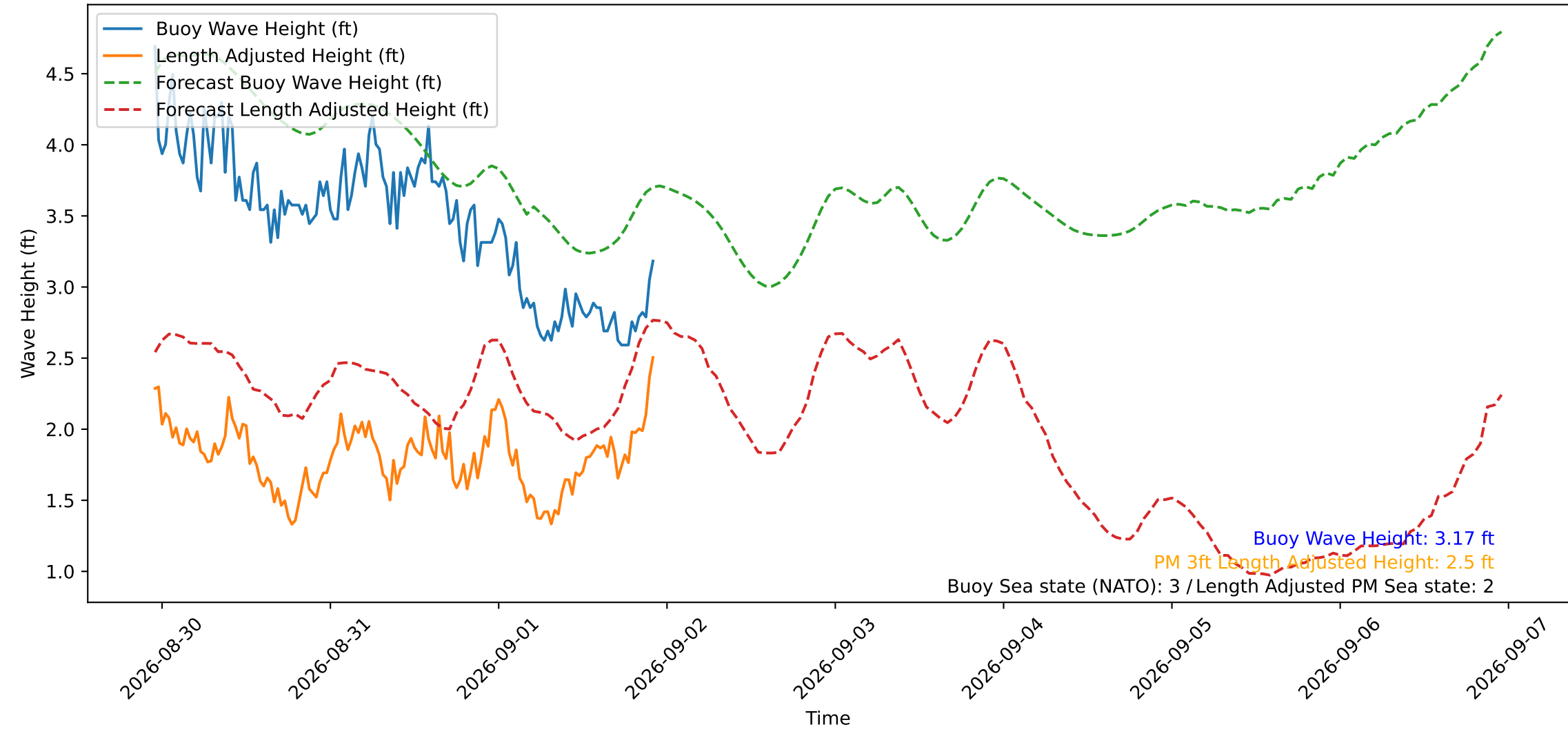
Wave Heights over Time for Red Beach at 2026-09-01 22:50:50
