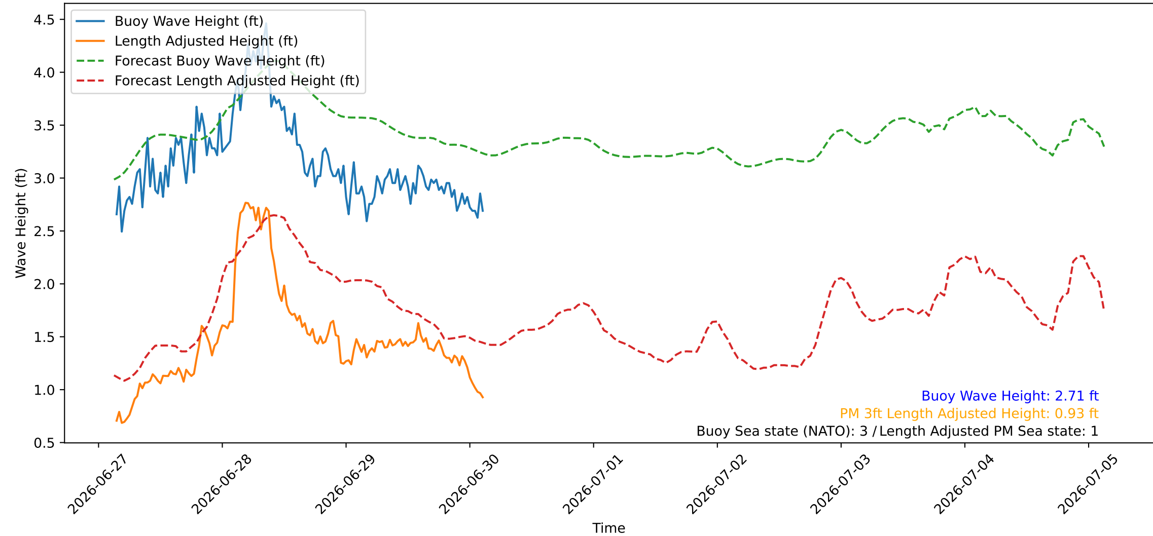
Wave Heights over Time for Red Beach at 2026-06-30 03:10:45
