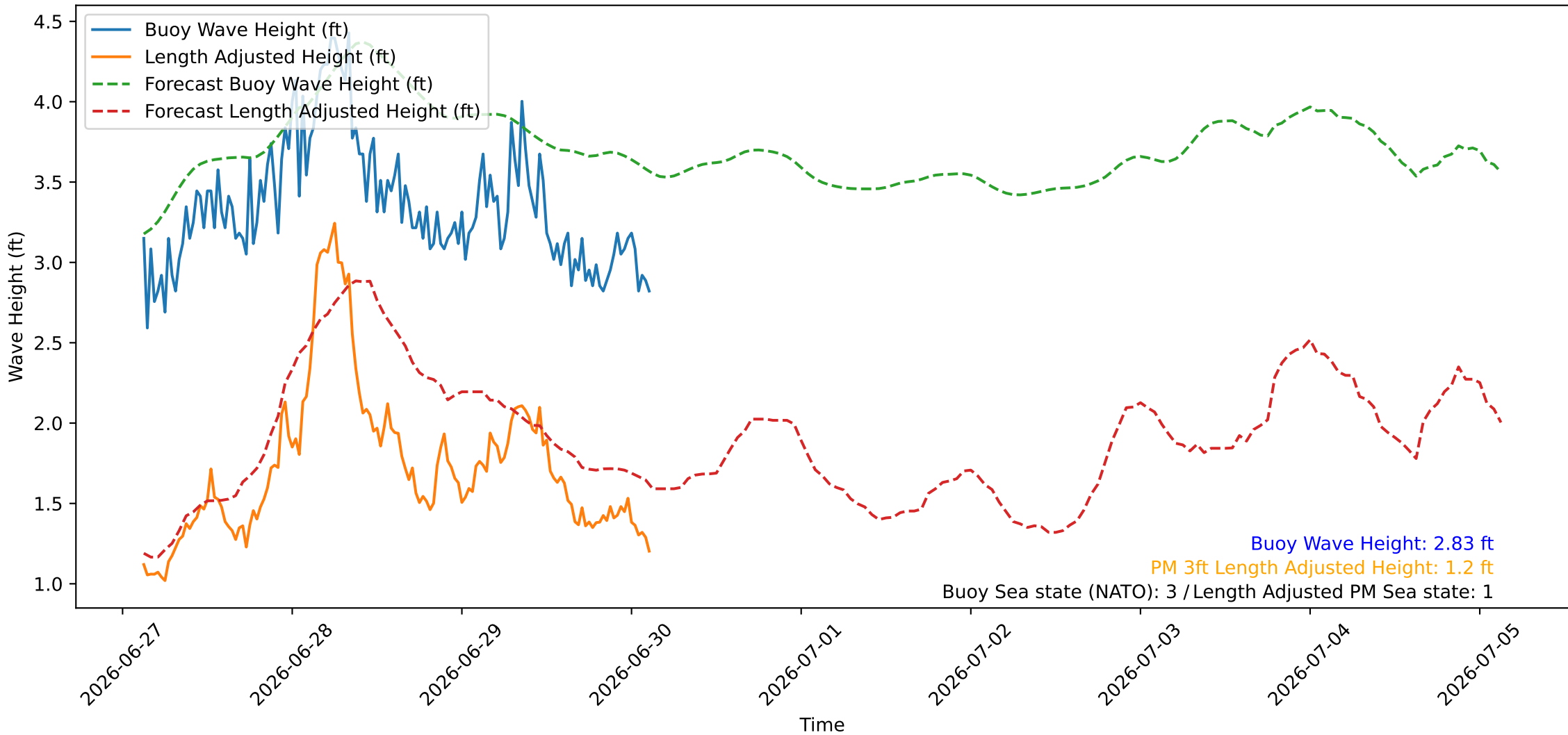
Wave Heights over Time for Oceanside Harbor at 2026-06-30 03:10:26
