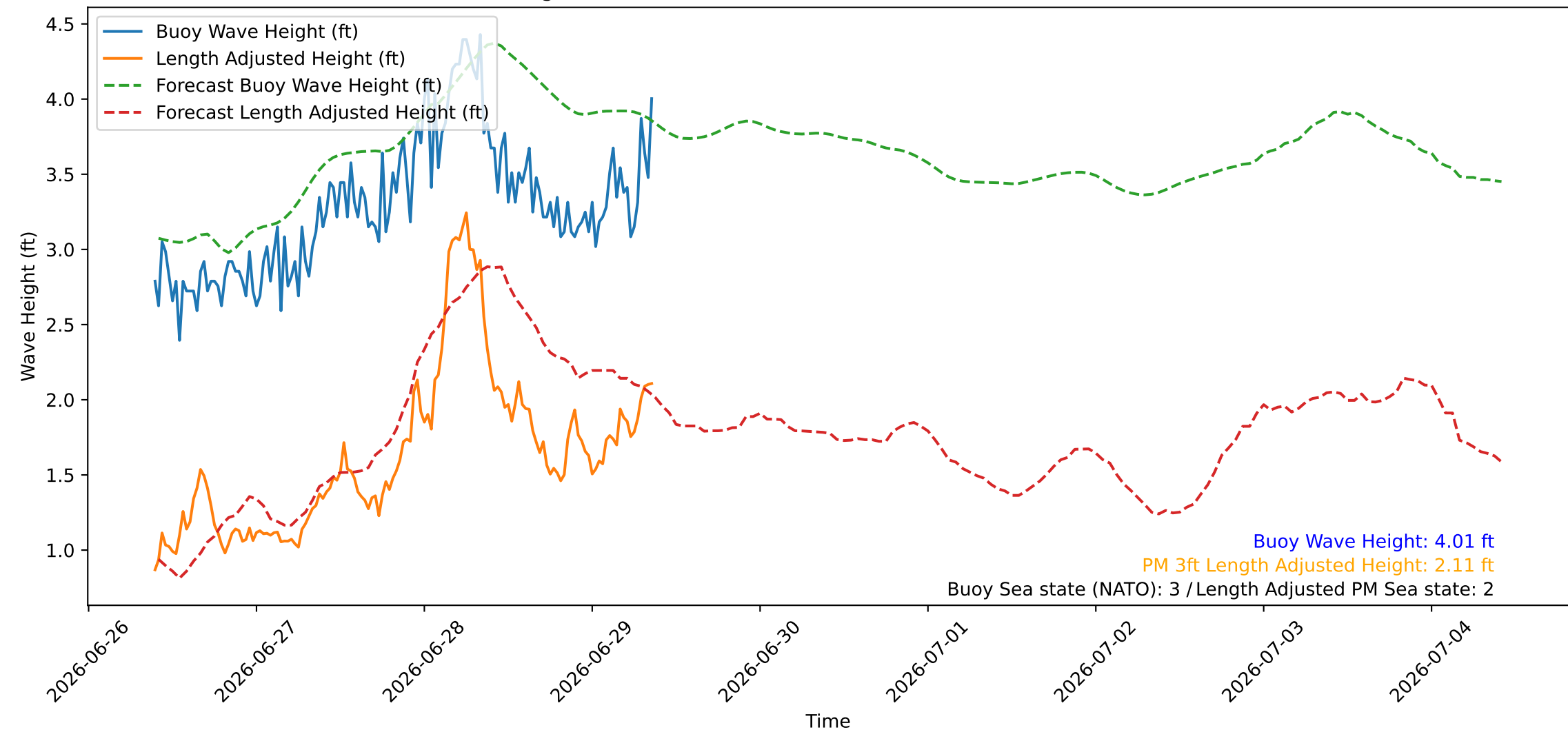
Wave Heights over Time for Oceanside Harbor at 2026-06-29 09:30:26
