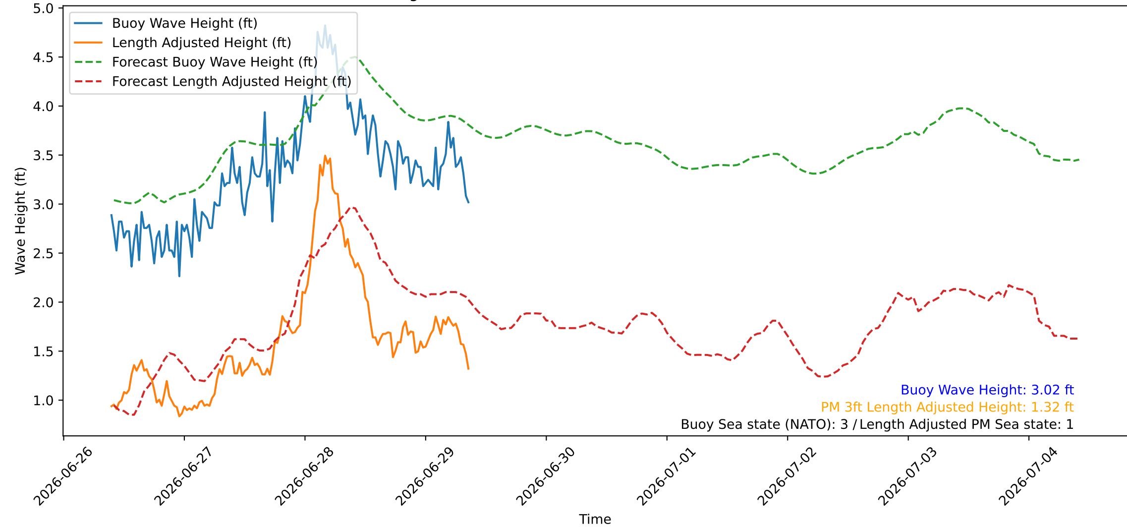
Wave Heights over Time for Green Beach at 2026-06-29 09:31:08
