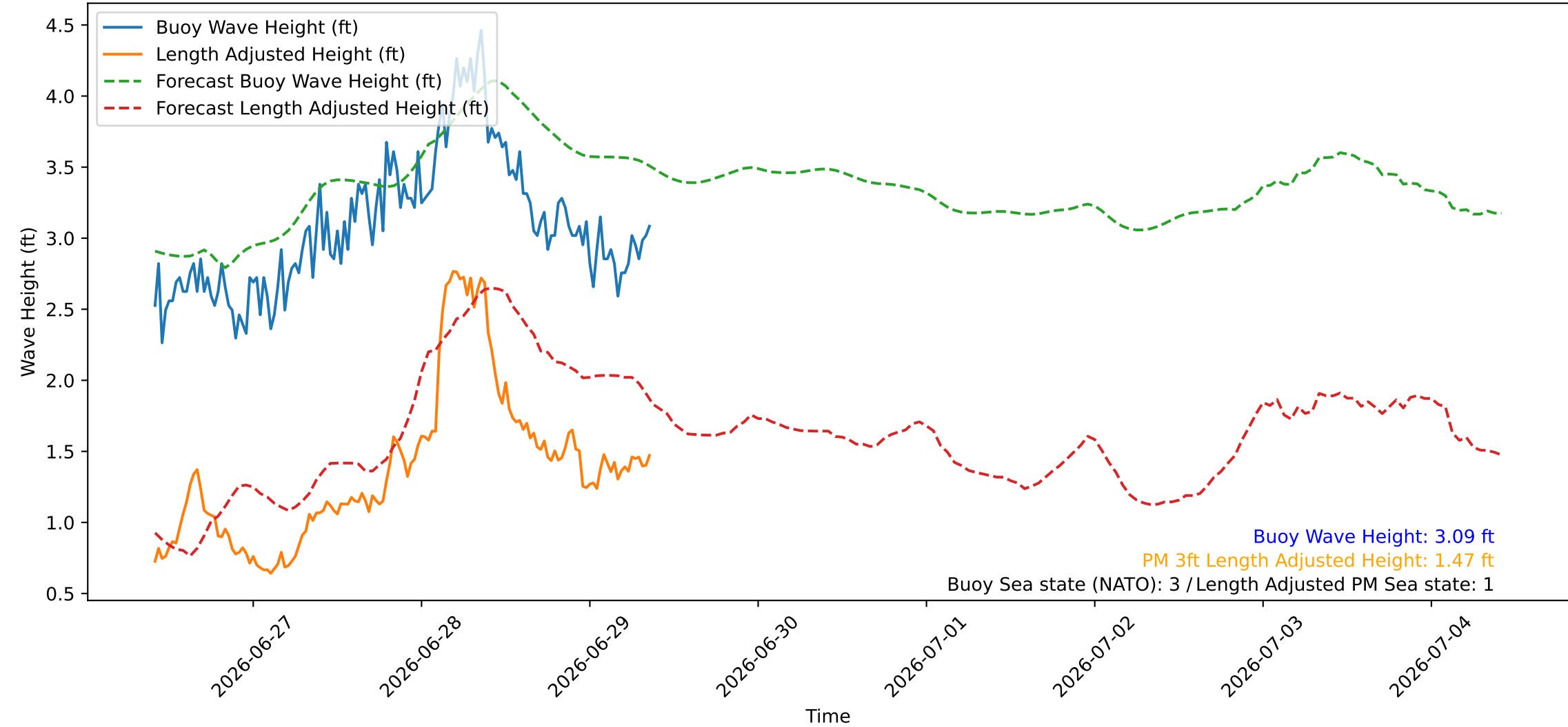
Wave Heights over Time for Red Beach at 2026-06-29 09:30:46
