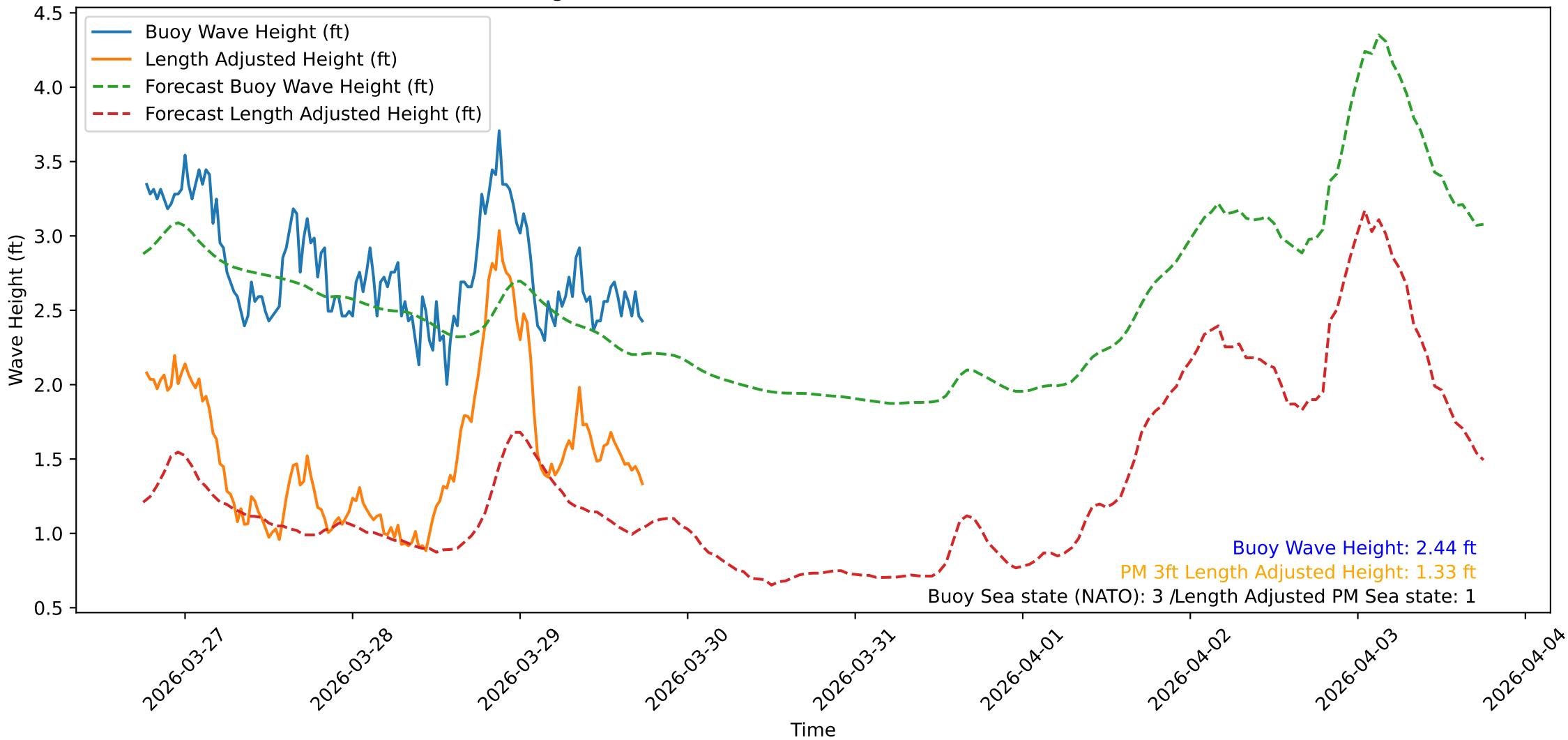
Wave Heights over Time for Green Beach at 2026-03-29 18:21:10
