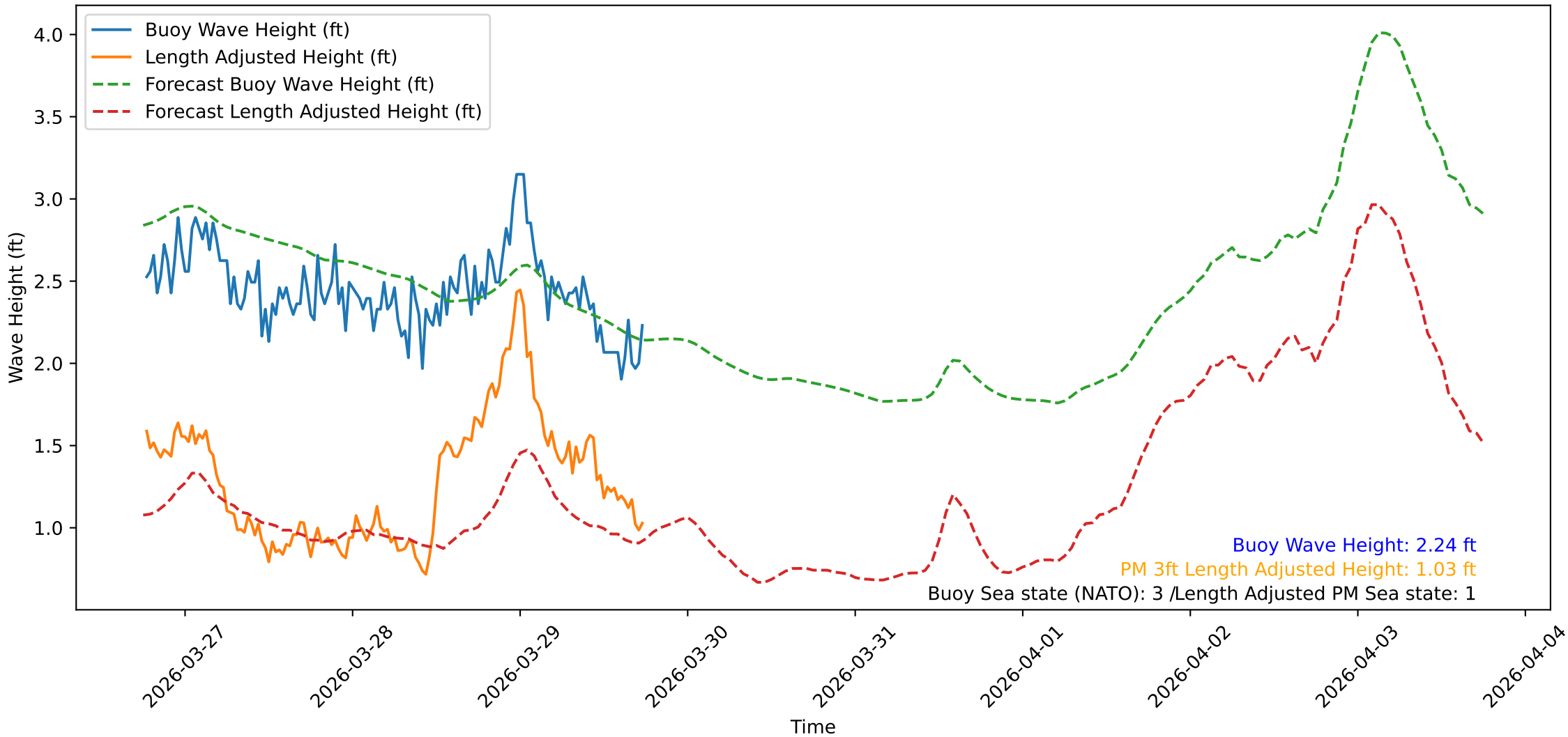
Wave Heights over Time for Oceanside Harbor at 2026-03-29 18:20:32
