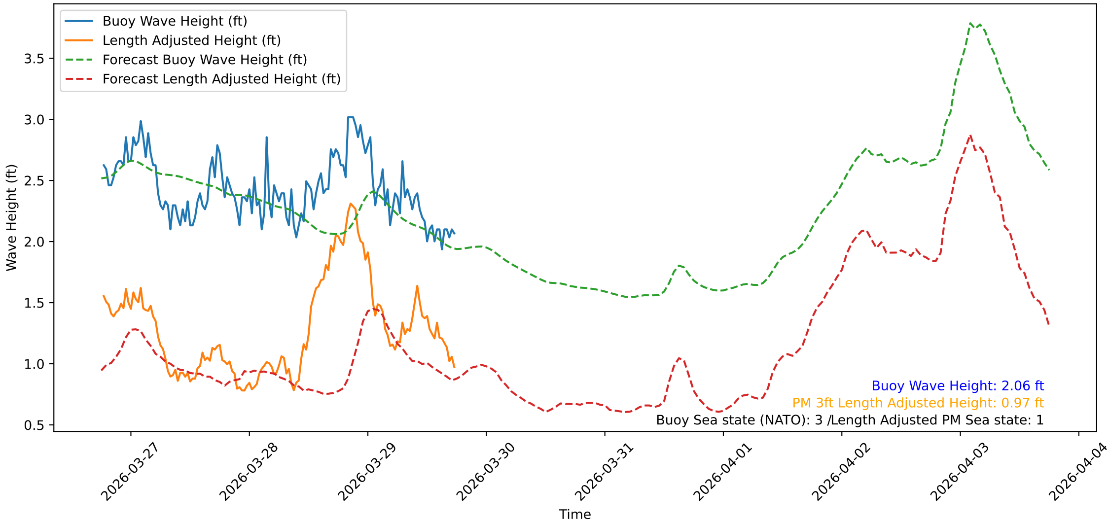
Wave Heights over Time for Red Beach at 2026-03-29 18:20:48
