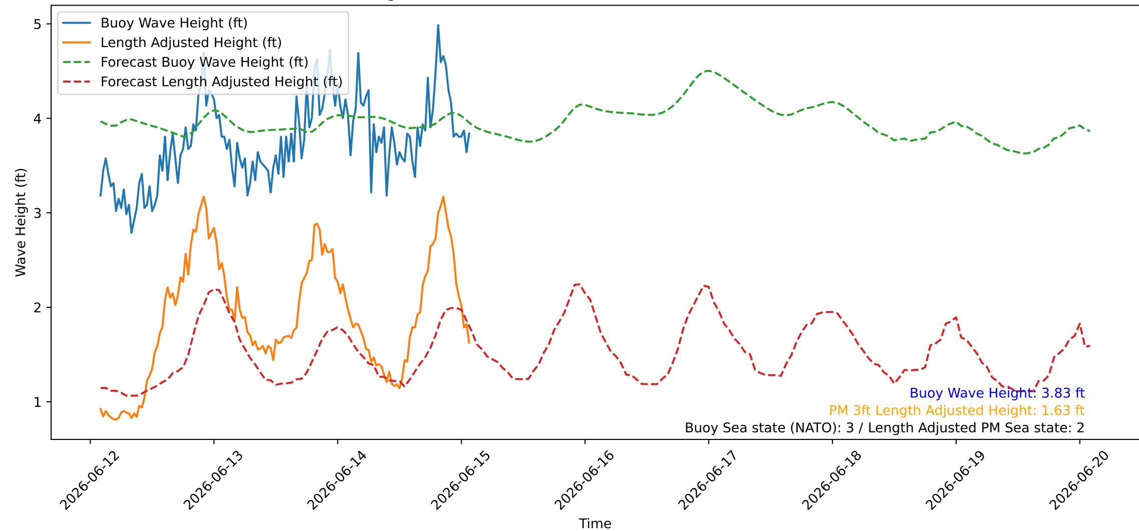
Wave Heights over Time for Oceanside Harbor at 2026-06-15 02:10:26
