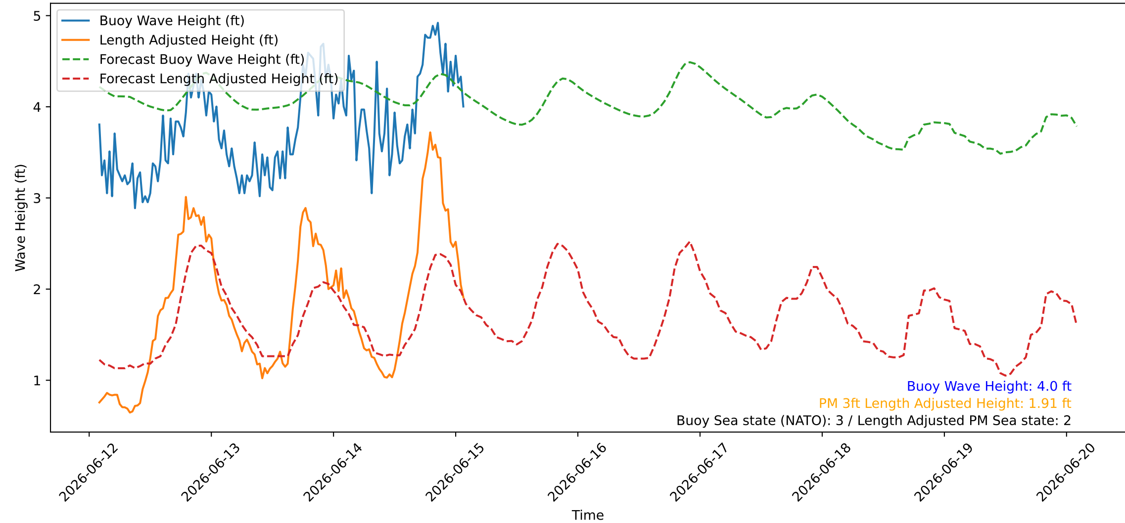
Wave Heights over Time for Green Beach at 2026-06-15 02:11:08
