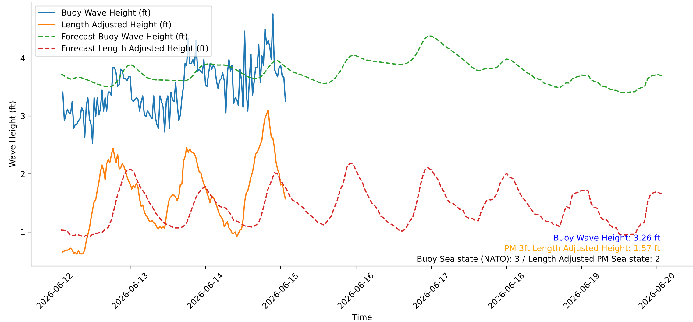
Wave Heights over Time for Red Beach at 2026-06-15 02:10:45
