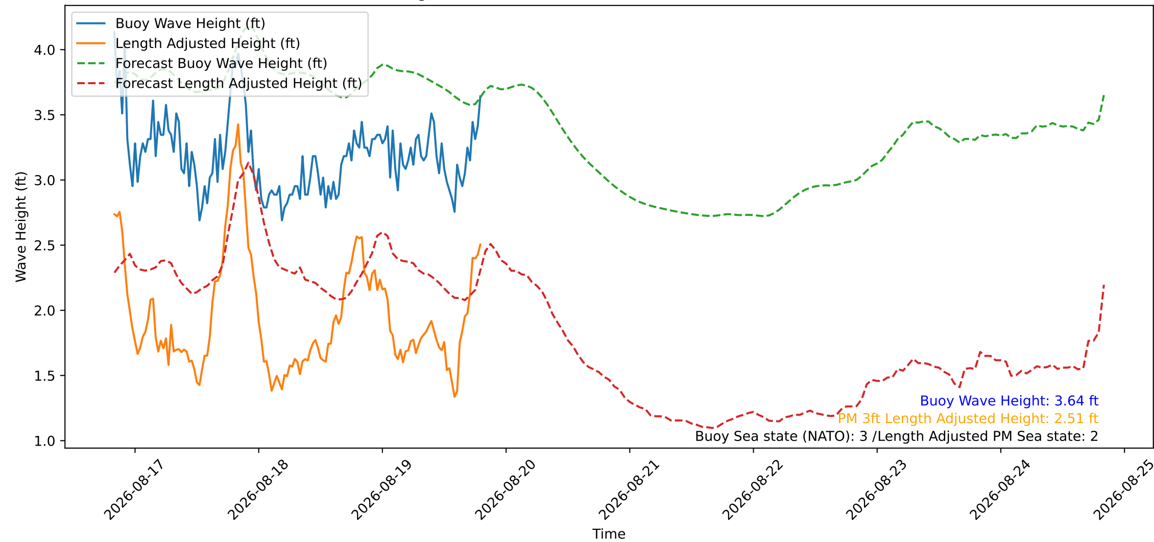
Wave Heights over Time for Green Beach at 2026-08-19 19:41:11
