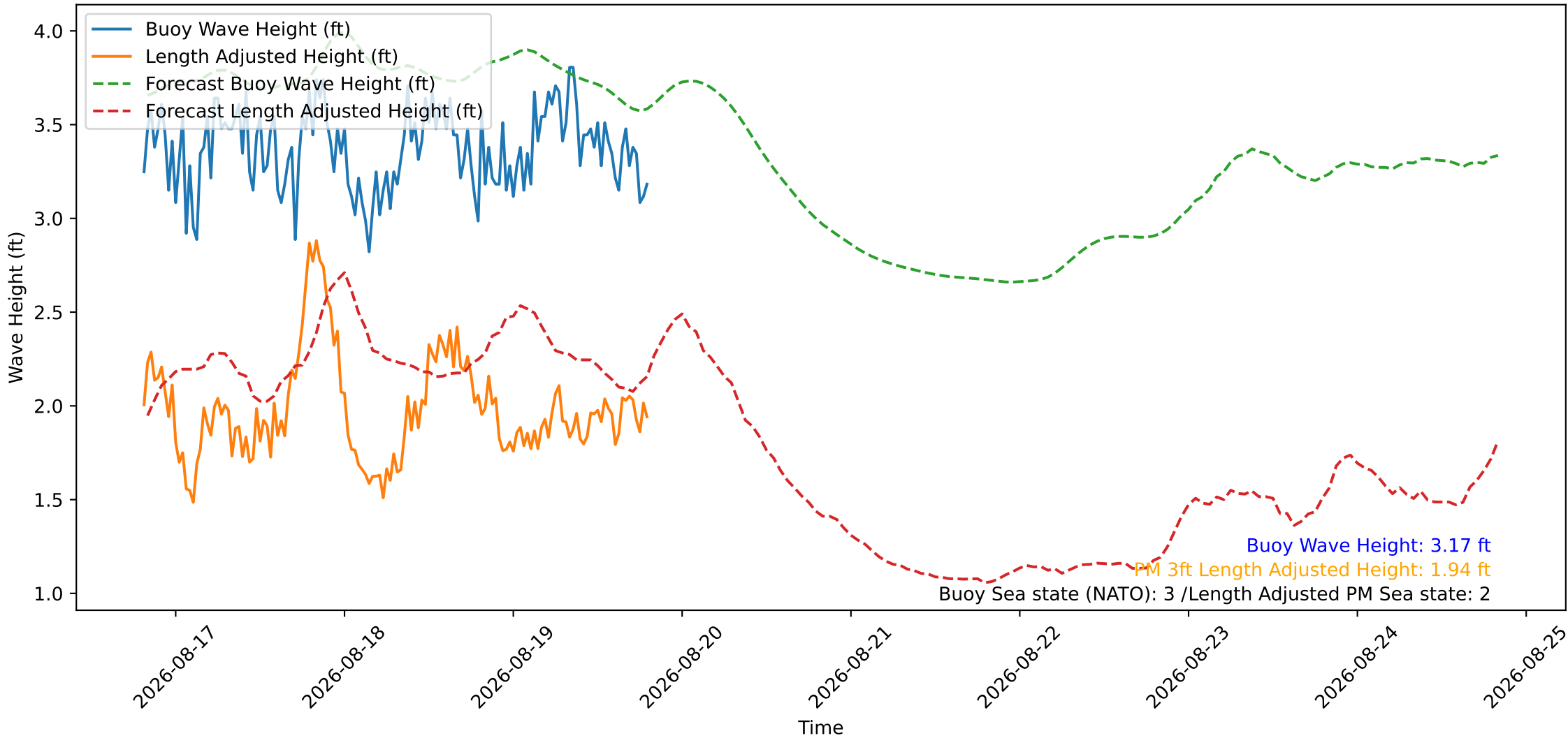
Wave Heights over Time for Oceanside Harbor at 2026-08-19 19:40:27
