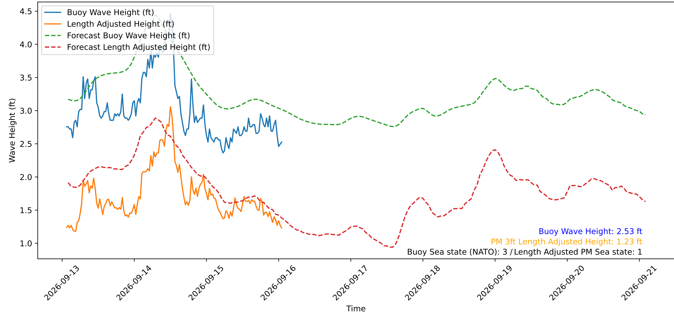
Wave Heights over Time for Oceanside Harbor at 2026-09-16 01:40:30
