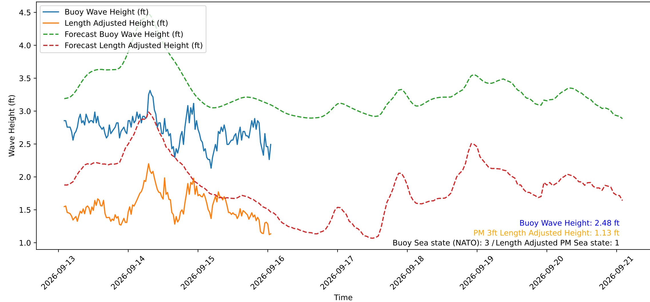
Wave Heights over Time for Green Beach at 2026-09-16 01:41:12
