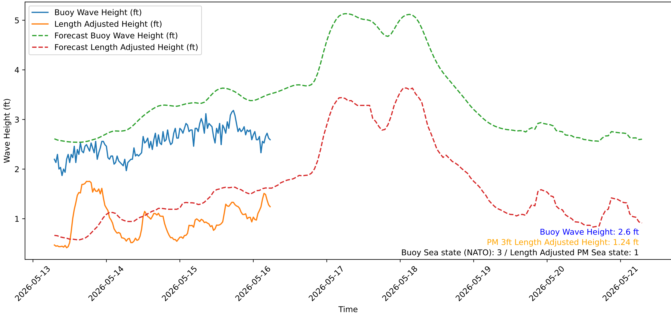
Wave Heights over Time for Red Beach at 2026-05-16 06:30:51
