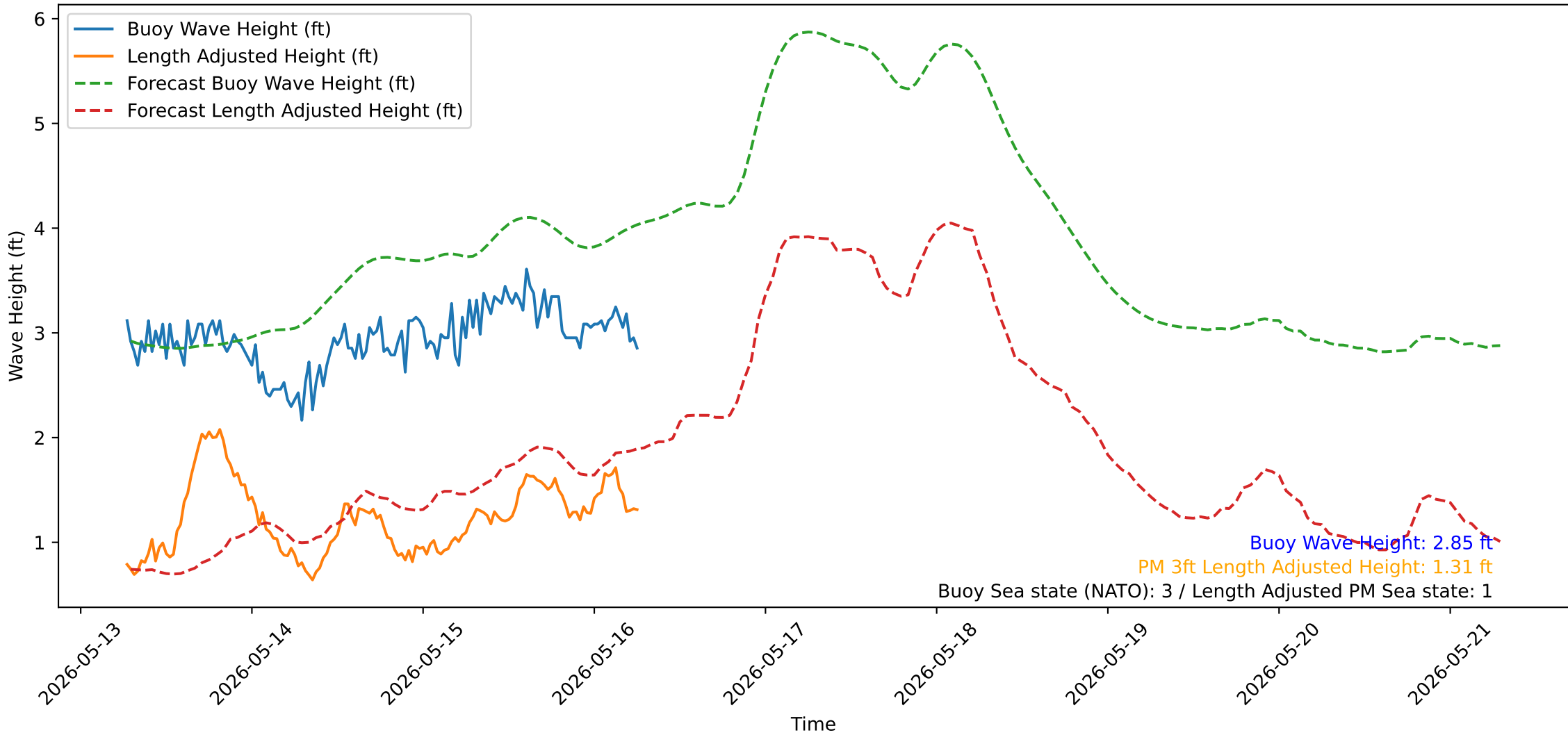
Wave Heights over Time for Oceanside Harbor at 2026-05-16 06:30:32
