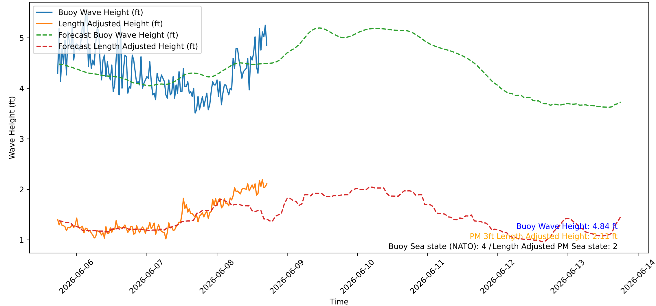
Wave Heights over Time for Oceanside Harbor at 2026-06-08 17:40:26
