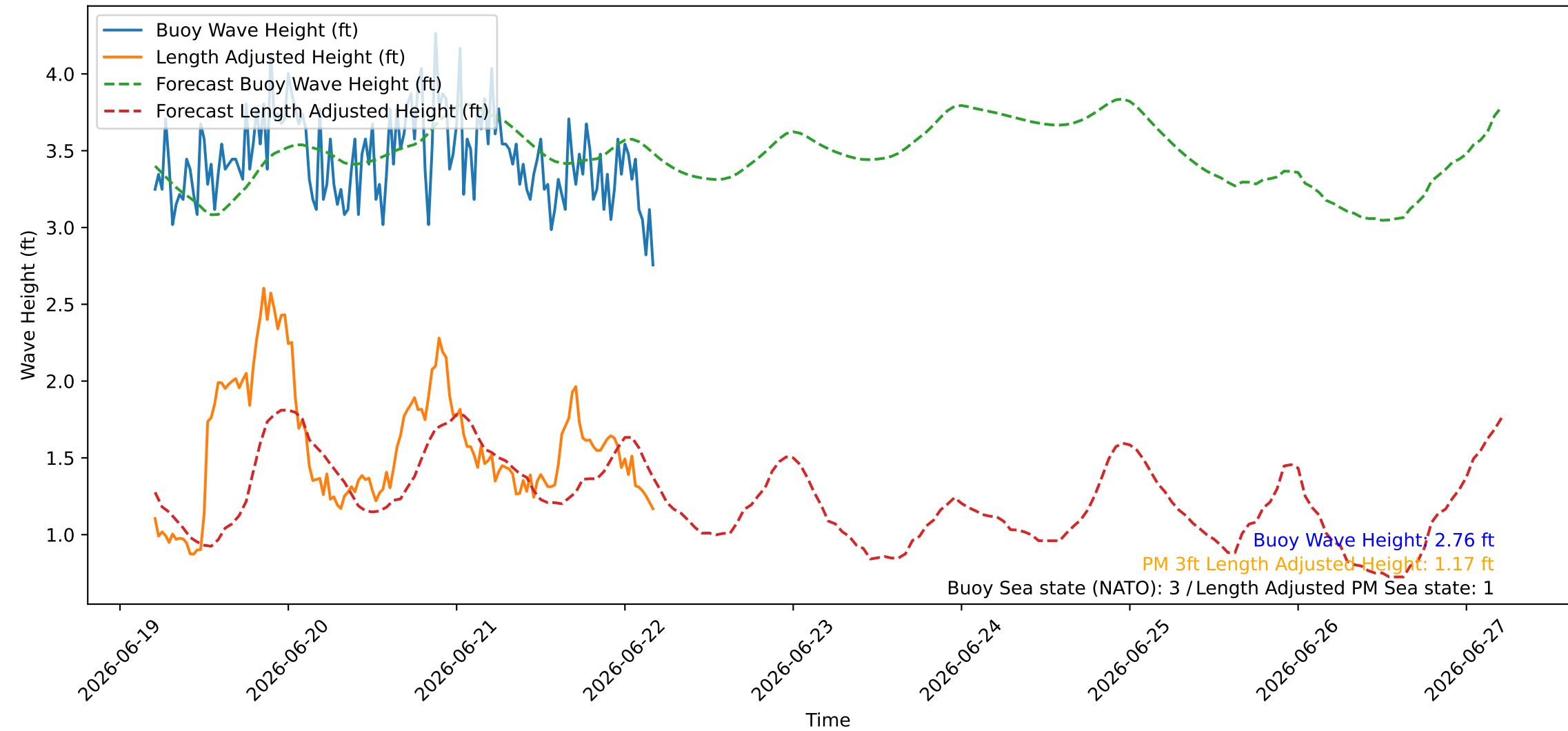
Wave Heights over Time for Oceanside Harbor at 2026-06-22 04:50:26
