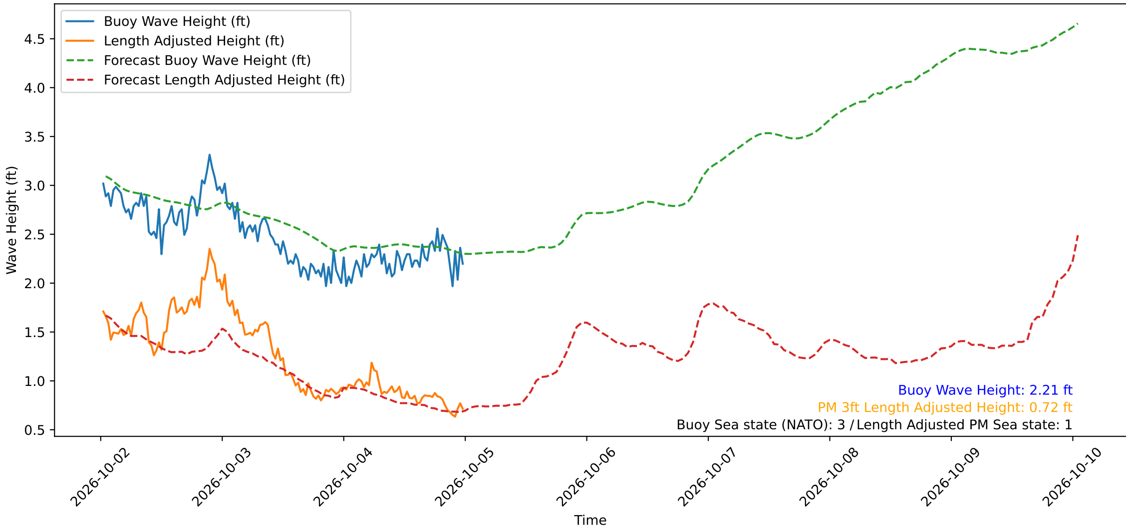
Wave Heights over Time for Oceanside Harbor at 2026-10-05 00:30:30
