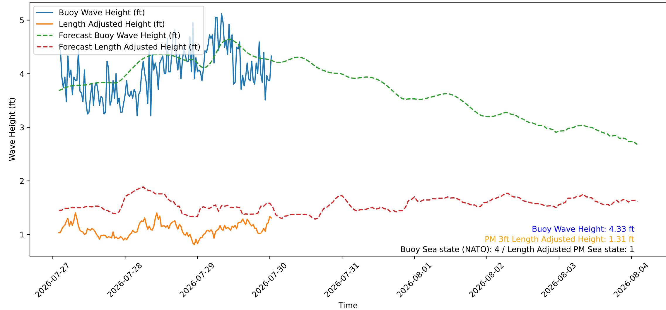
Wave Heights over Time for Red Beach at 2026-07-30 01:30:46
