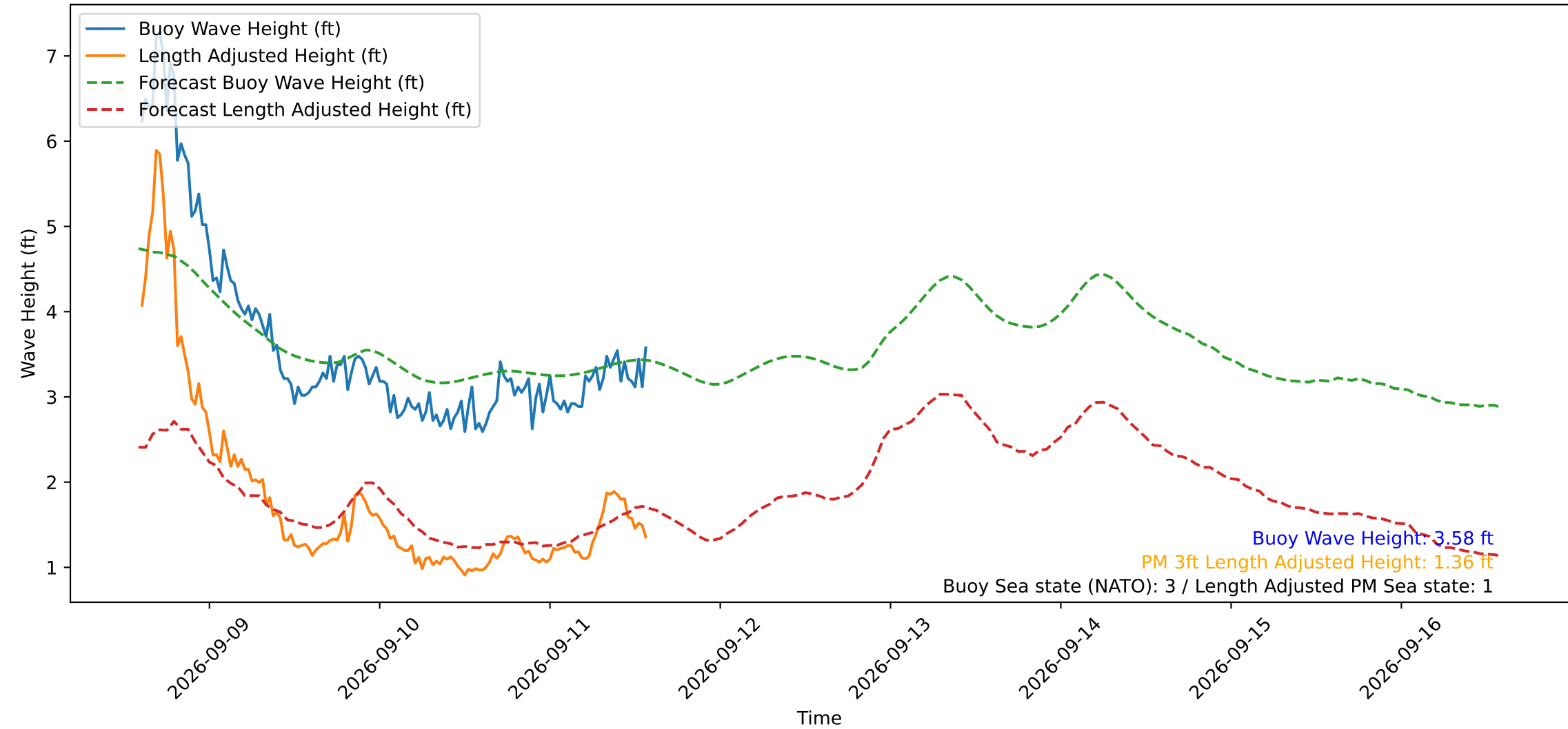
Wave Heights over Time for Green Beach at 2026-09-11 14:21:15
