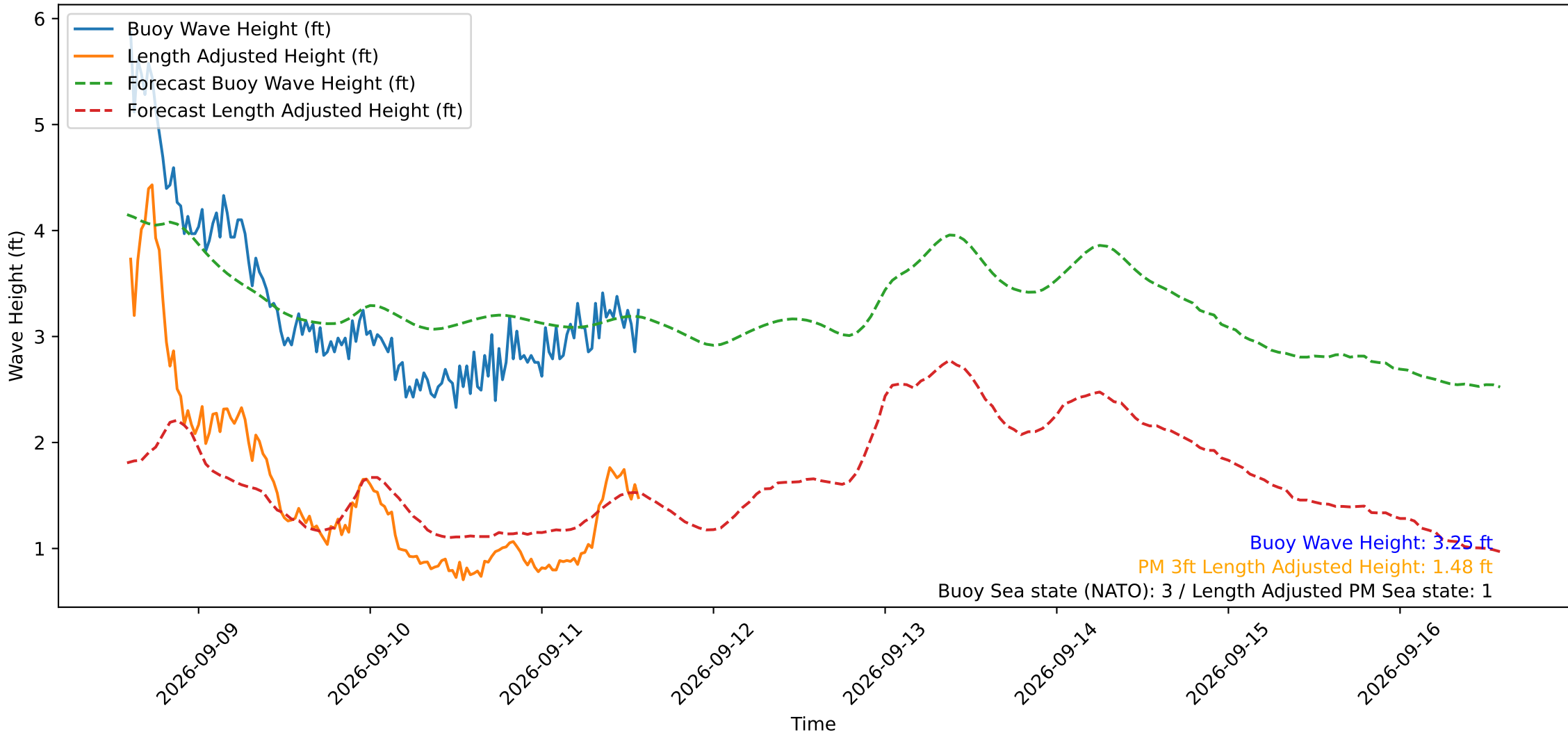
Wave Heights over Time for Red Beach at 2026-09-11 14:20:51
