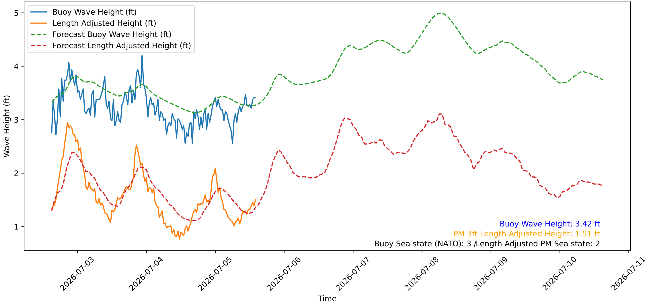
Wave Heights over Time for Green Beach at 2026-07-05 15:01:08
