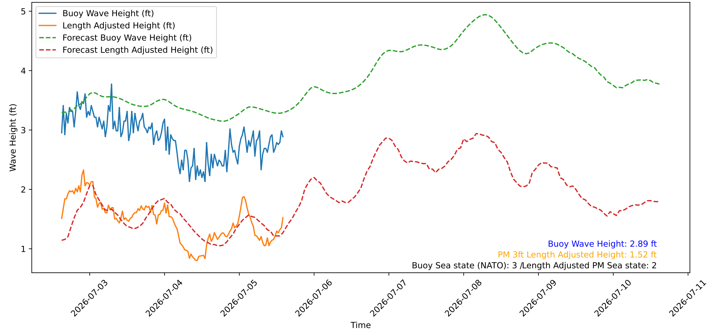
Wave Heights over Time for Oceanside Harbor at 2026-07-05 15:00:27
