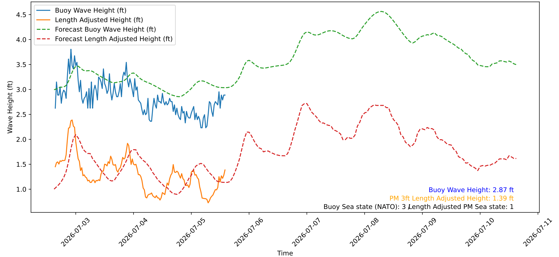
Wave Heights over Time for Red Beach at 2026-07-05 15:00:46
