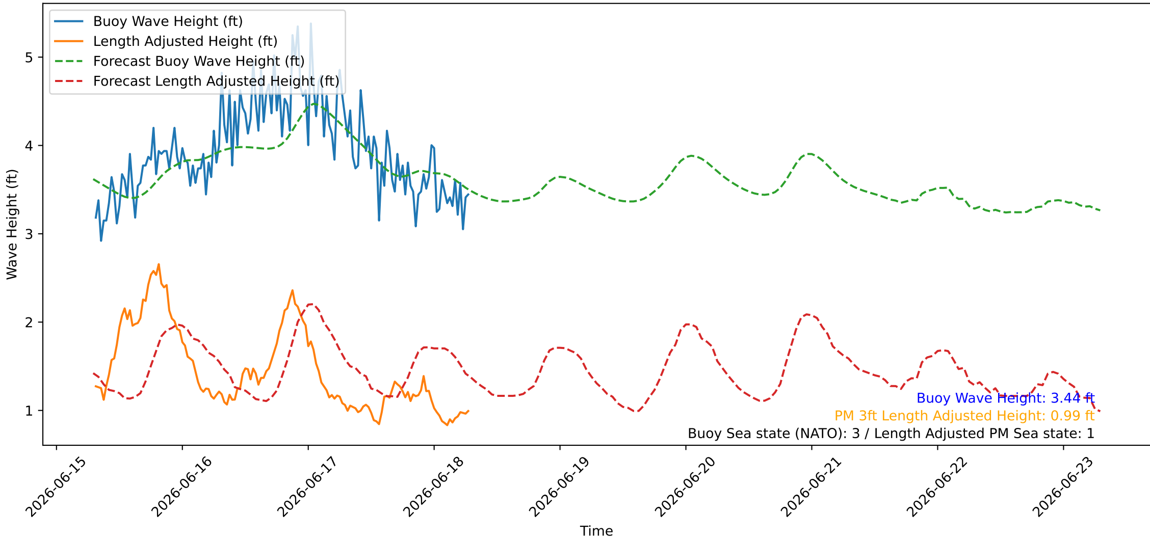
Wave Heights over Time for Red Beach at 2026-06-18 07:20:47
