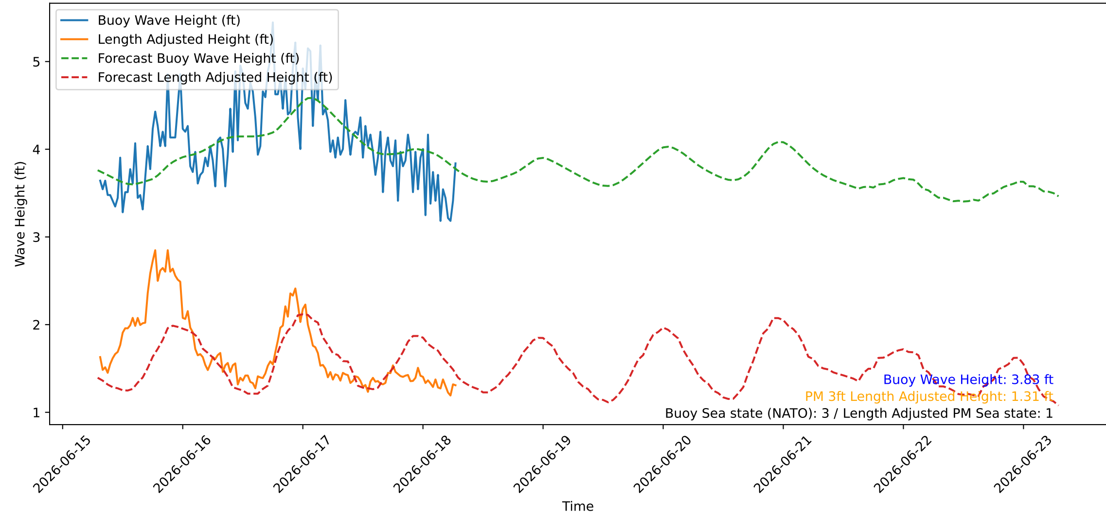
Wave Heights over Time for Oceanside Harbor at 2026-06-18 07:20:26
