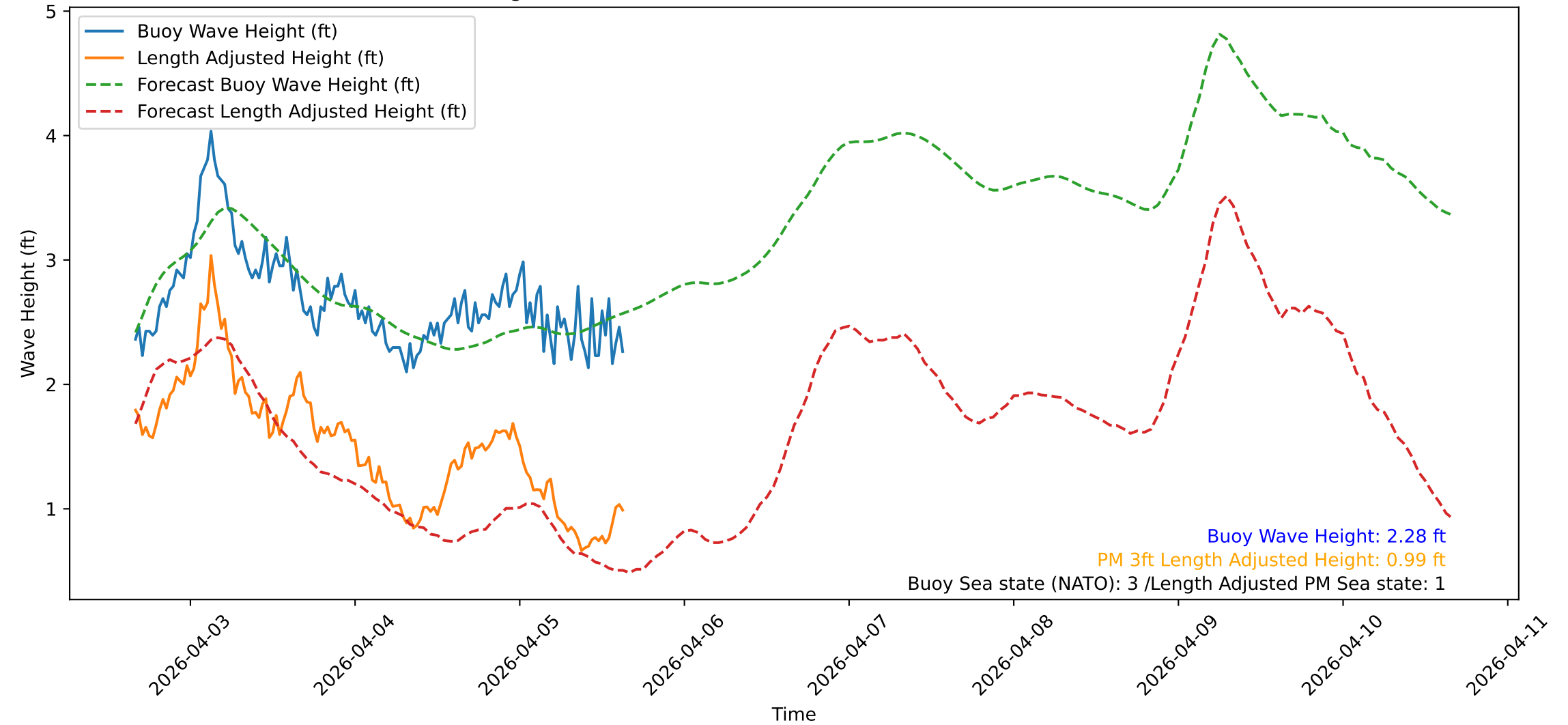
Wave Heights over Time for Oceanside Harbor at 2026-04-05 16:00:32
