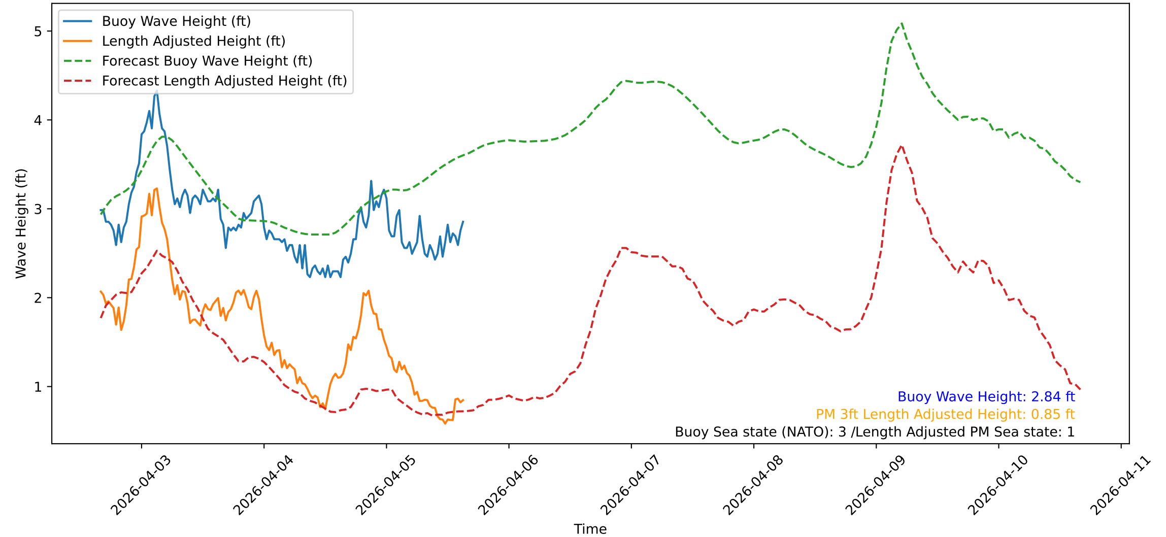
Wave Heights over Time for Green Beach at 2026-04-05 16:01:13
