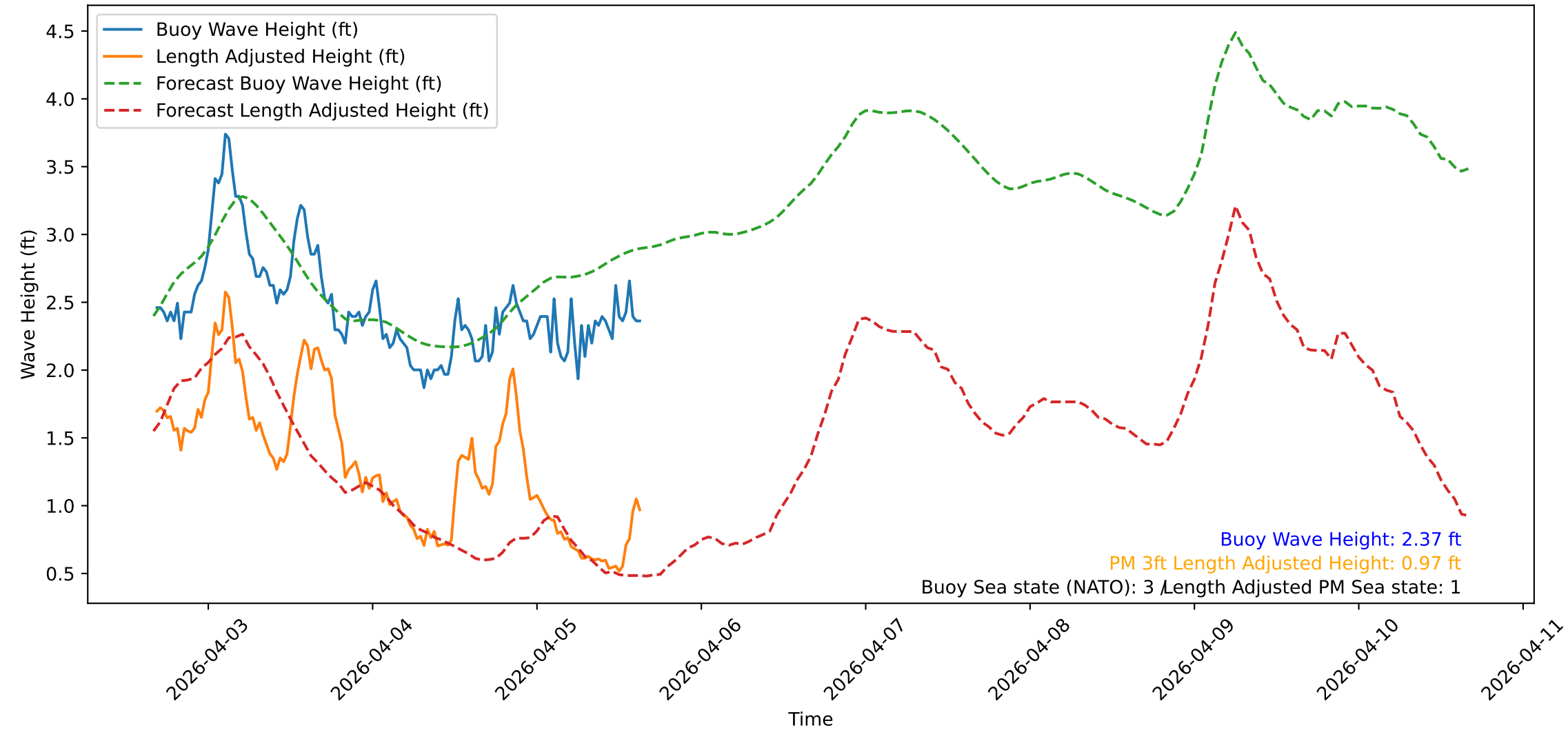
Wave Heights over Time for Red Beach at 2026-04-05 16:00:49
