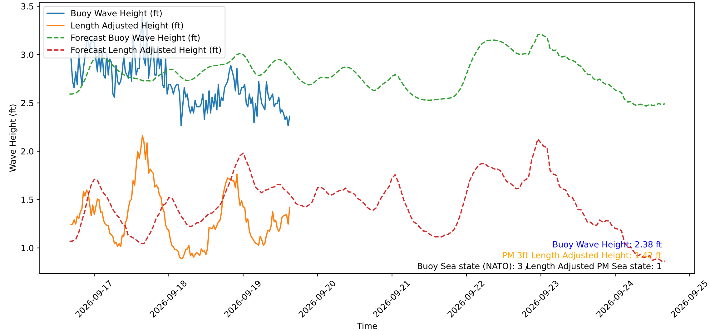
Wave Heights over Time for Red Beach at 2026-09-19 16:00:49
