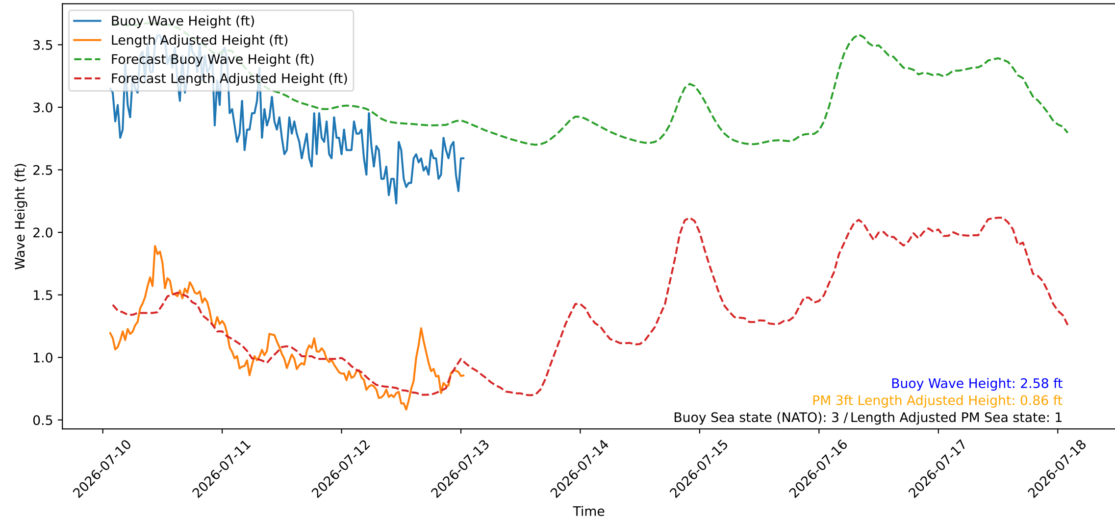
Wave Heights over Time for Green Beach at 2026-07-13 01:31:08
