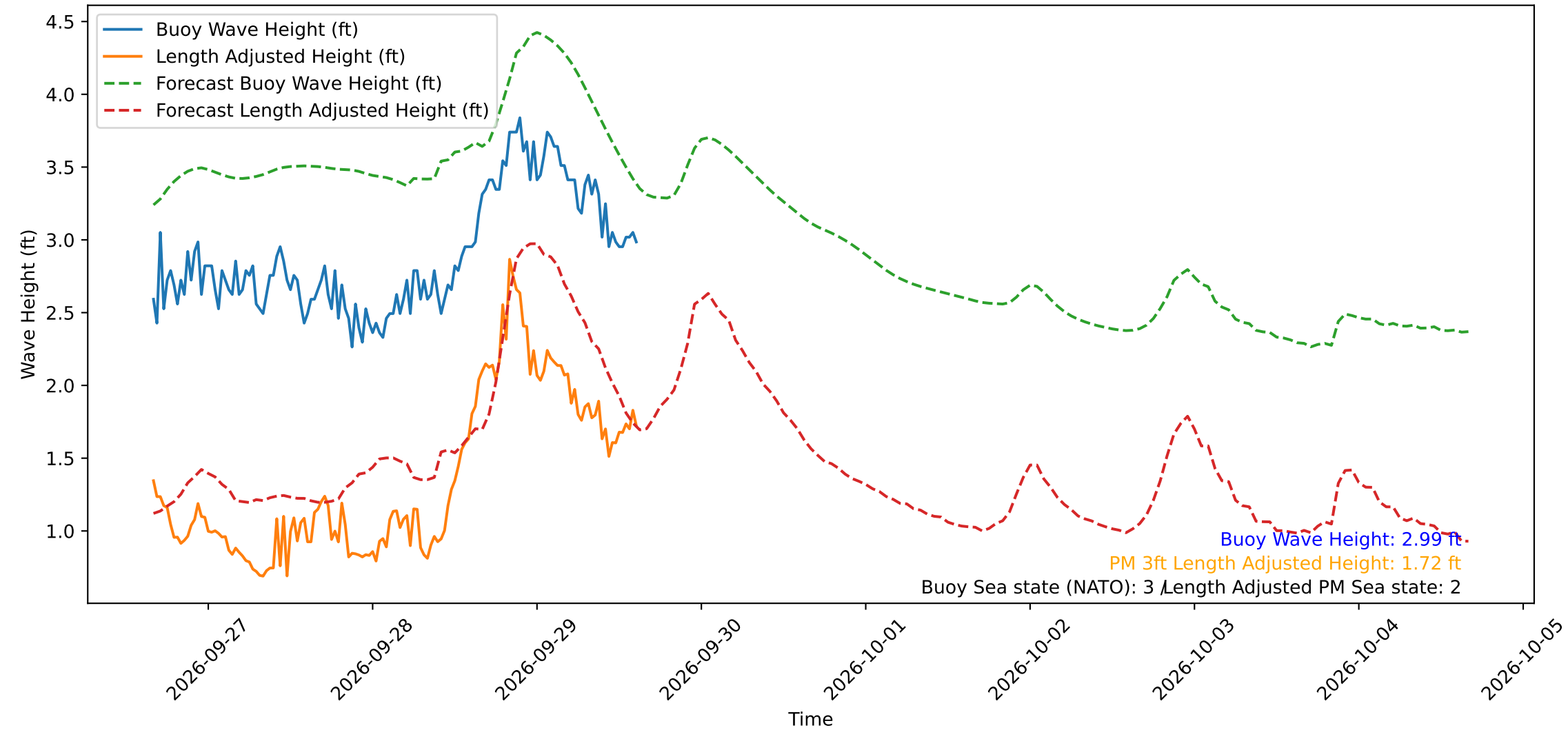
Wave Heights over Time for Red Beach at 2026-09-29 15:30:50
