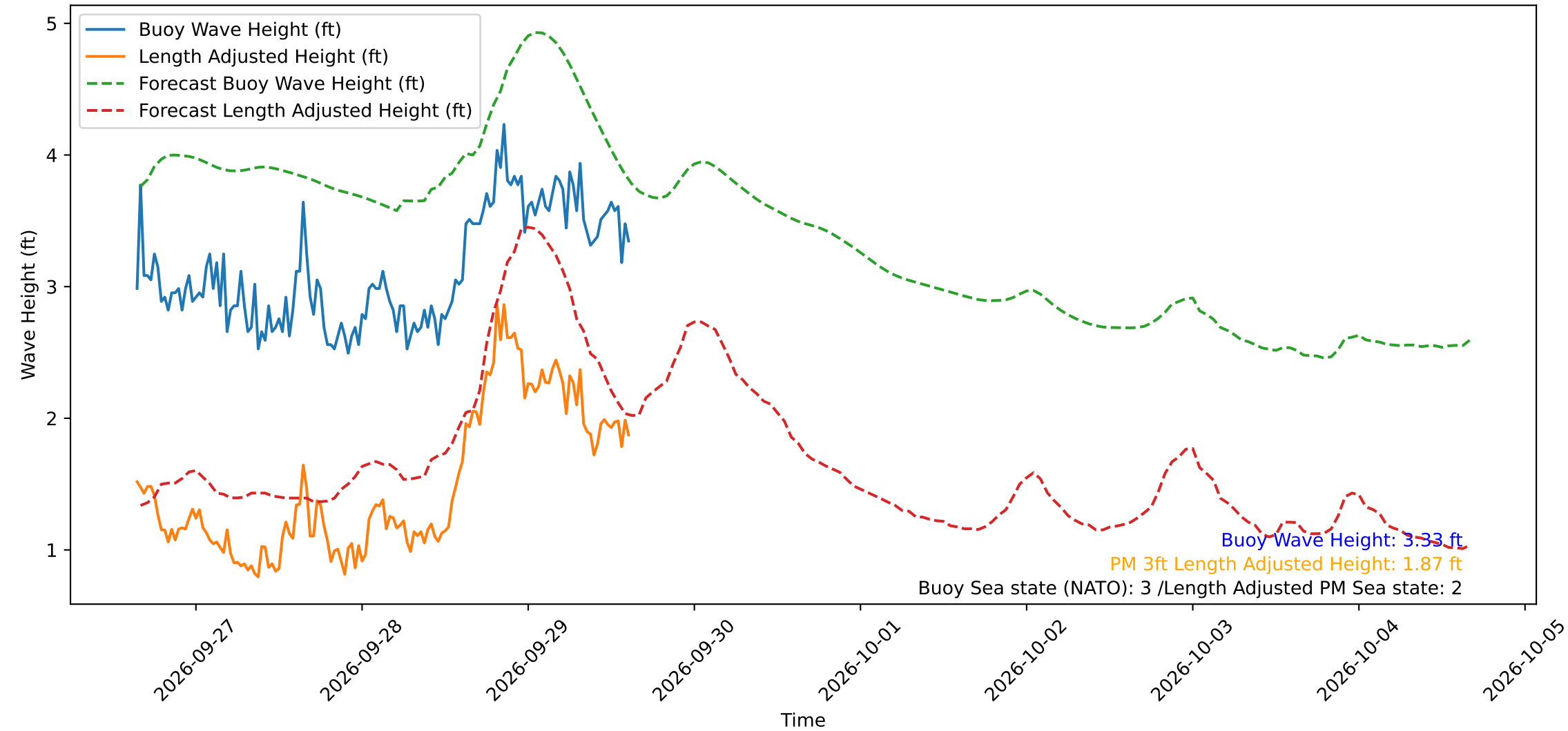
Wave Heights over Time for Oceanside Harbor at 2026-09-29 15:30:30
