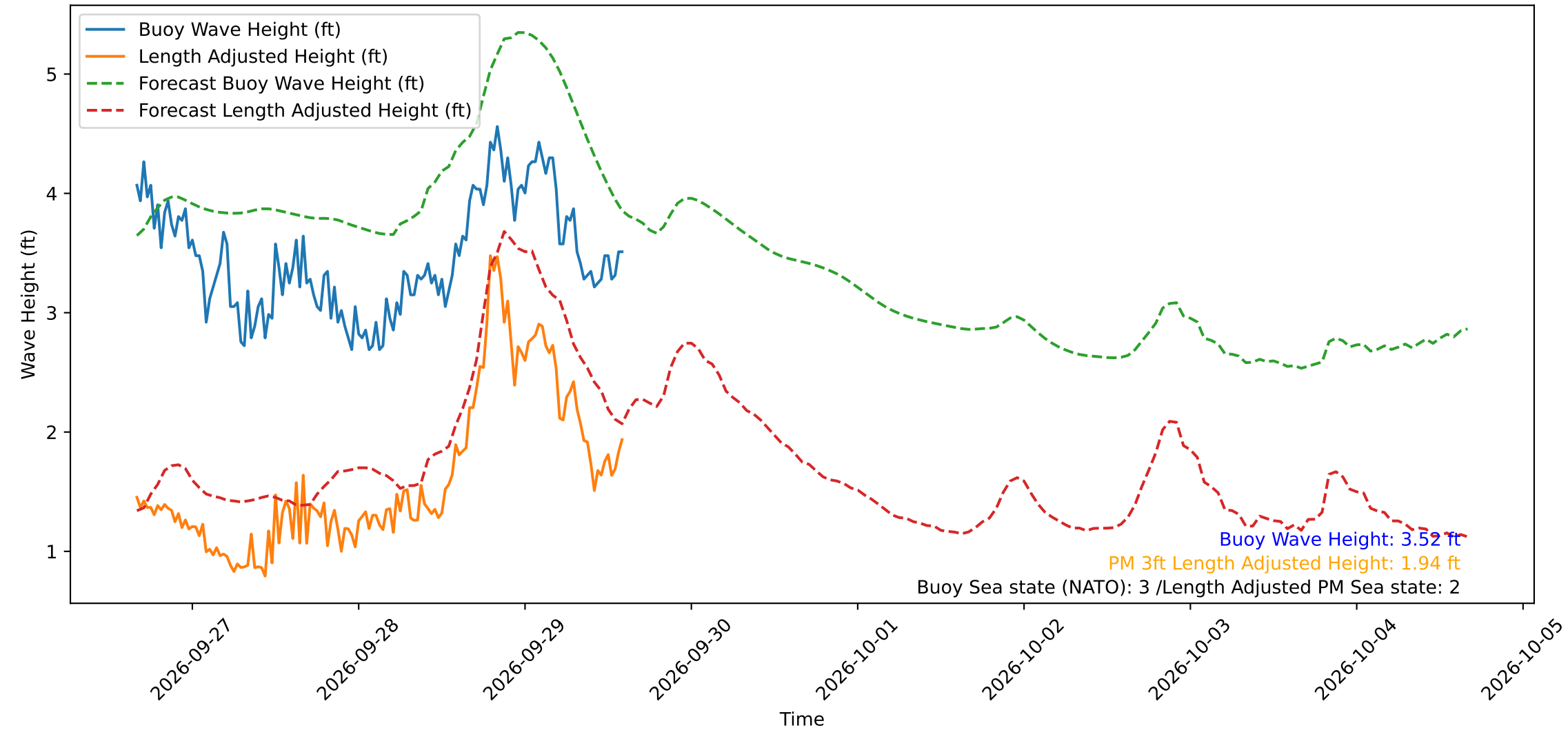
Wave Heights over Time for Green Beach at 2026-09-29 15:31:14
