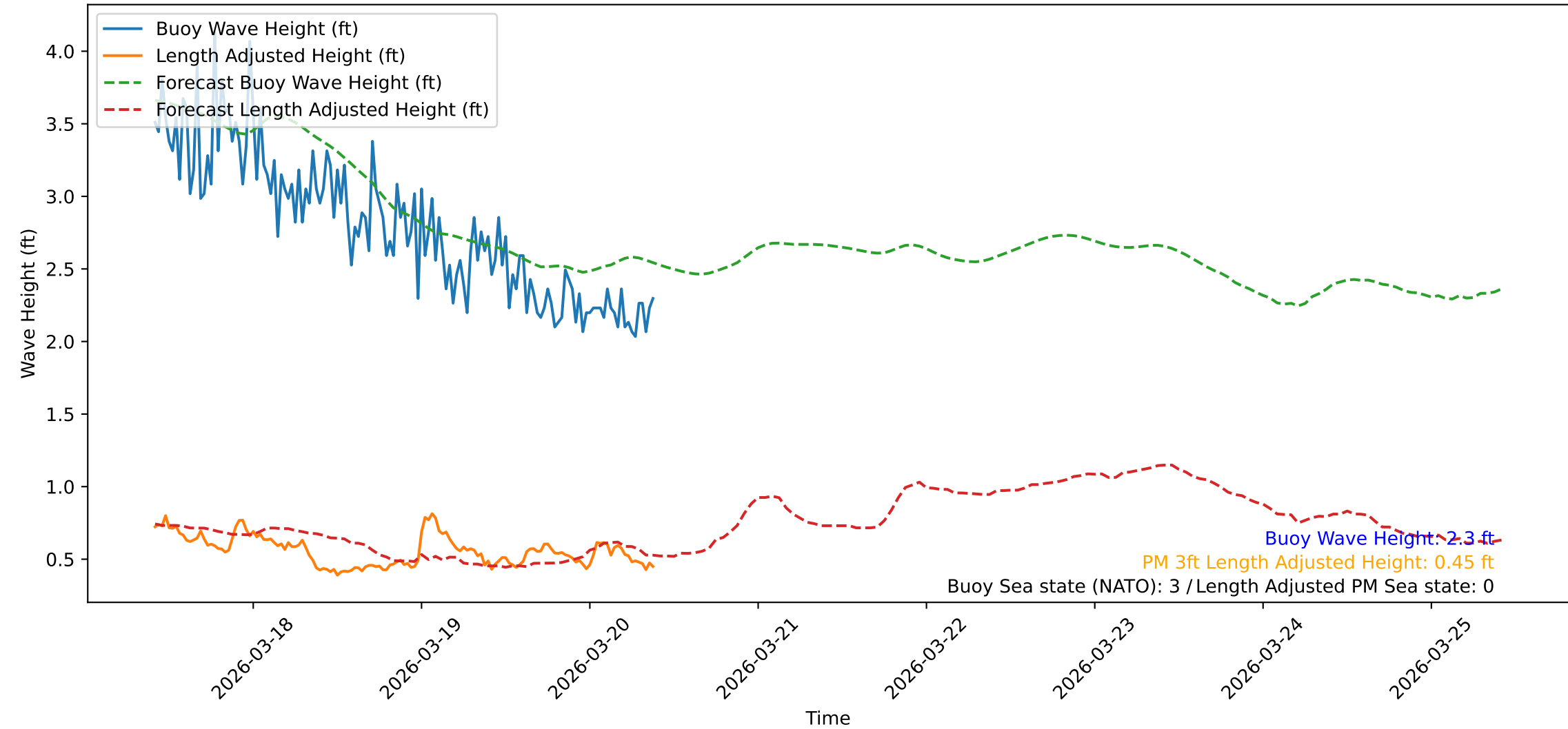
Wave Heights over Time for Green Beach at 2026-03-20 10:01:09
