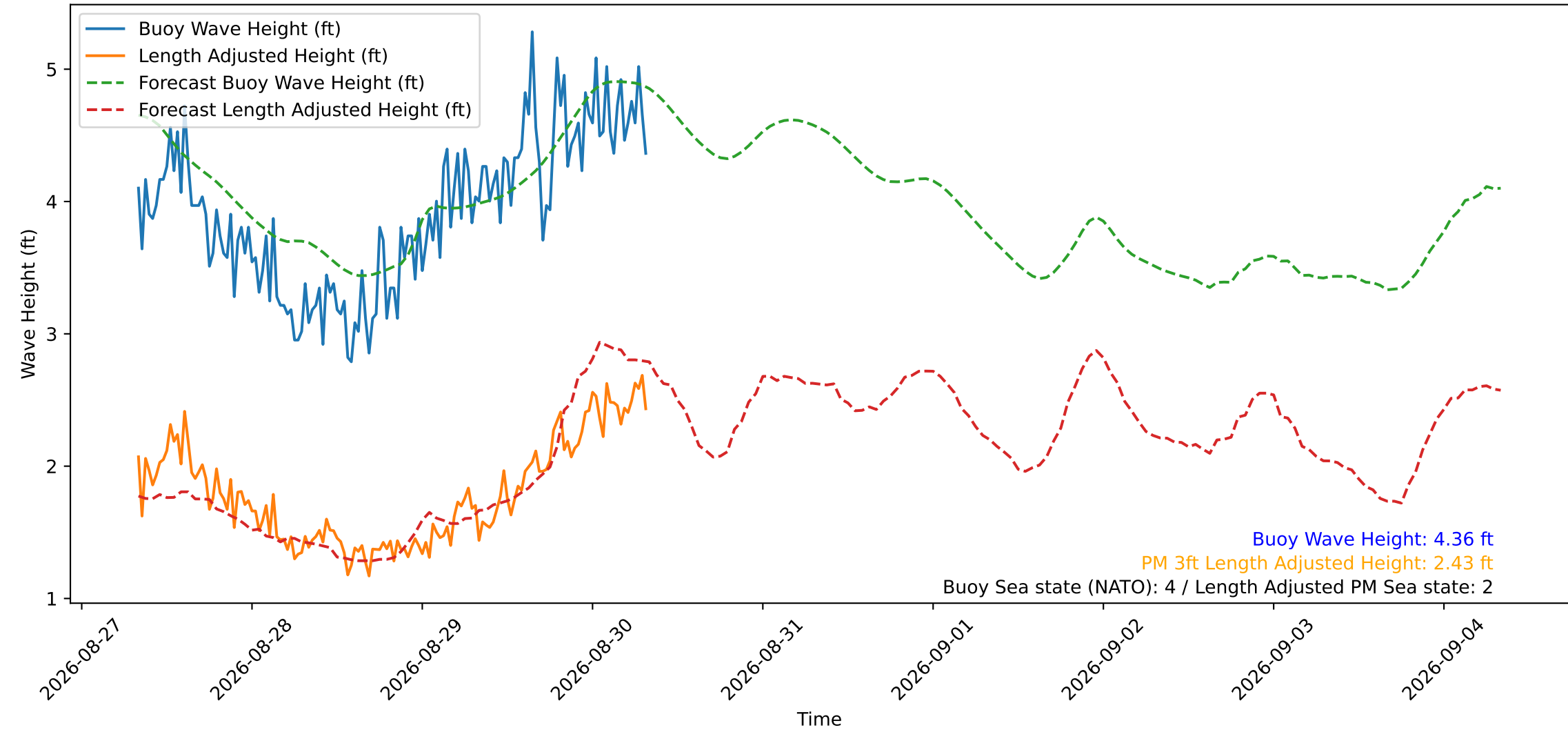
Wave Heights over Time for Oceanside Harbor at 2026-08-30 08:10:29
