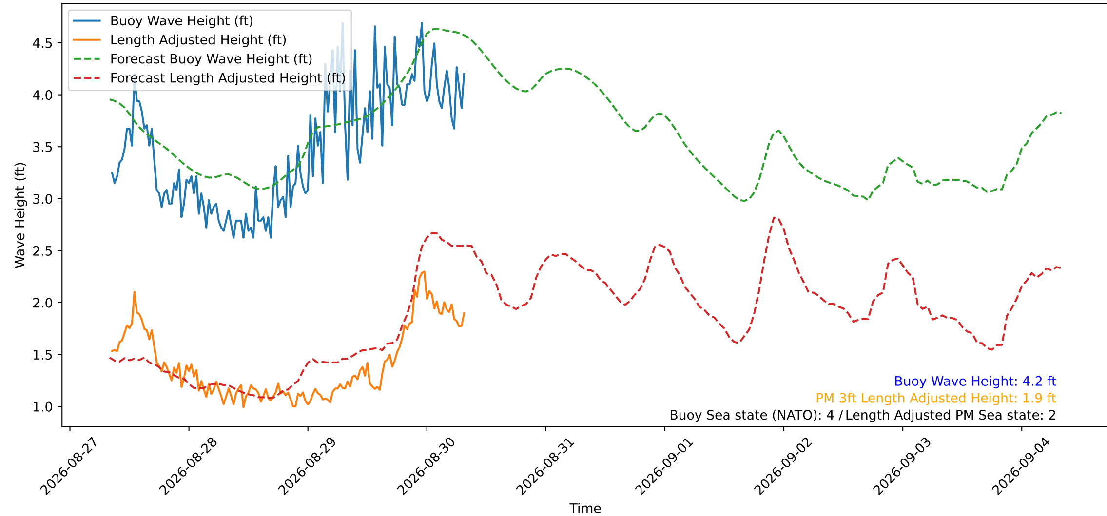
Wave Heights over Time for Red Beach at 2026-08-30 08:10:49
