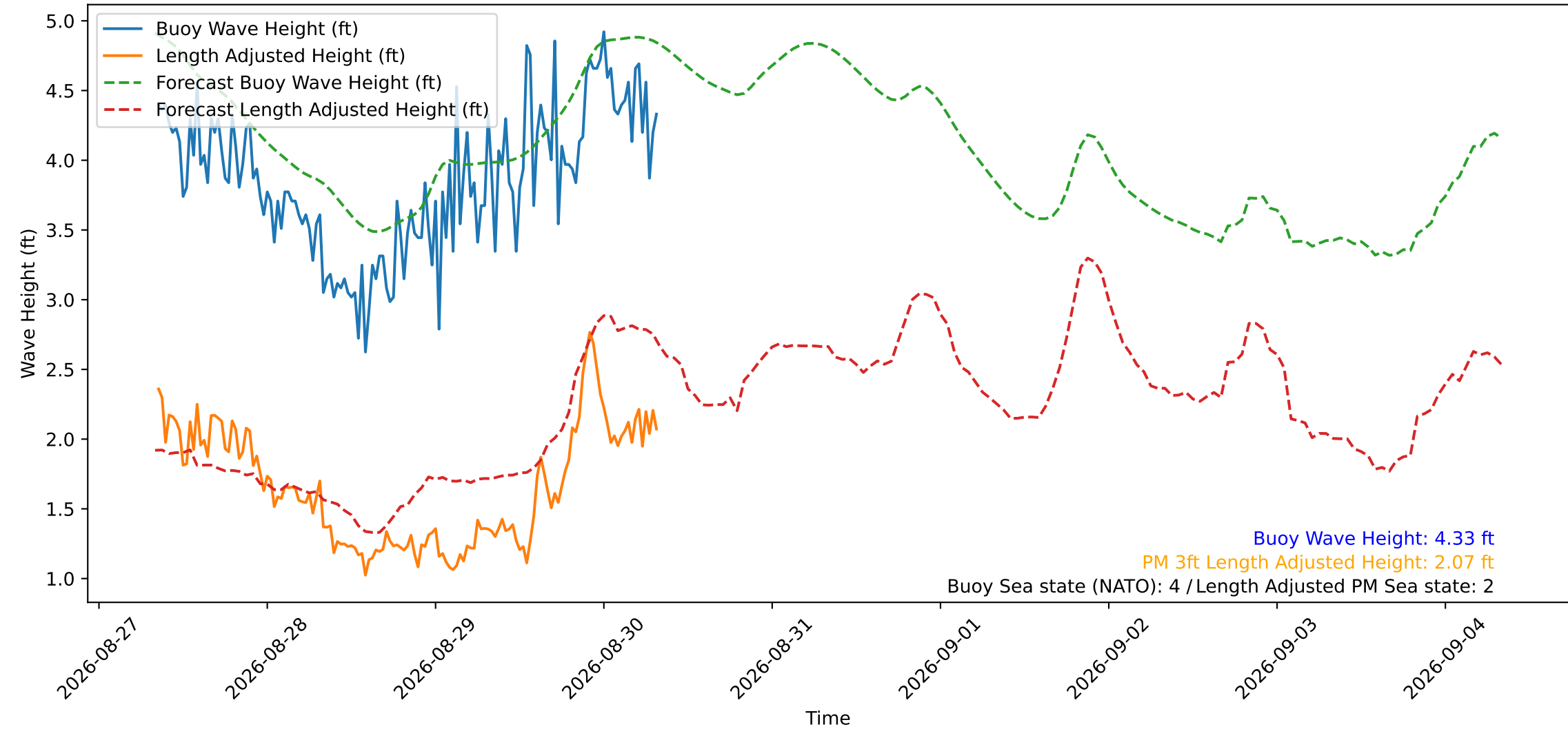
Wave Heights over Time for Green Beach at 2026-08-30 08:11:11
