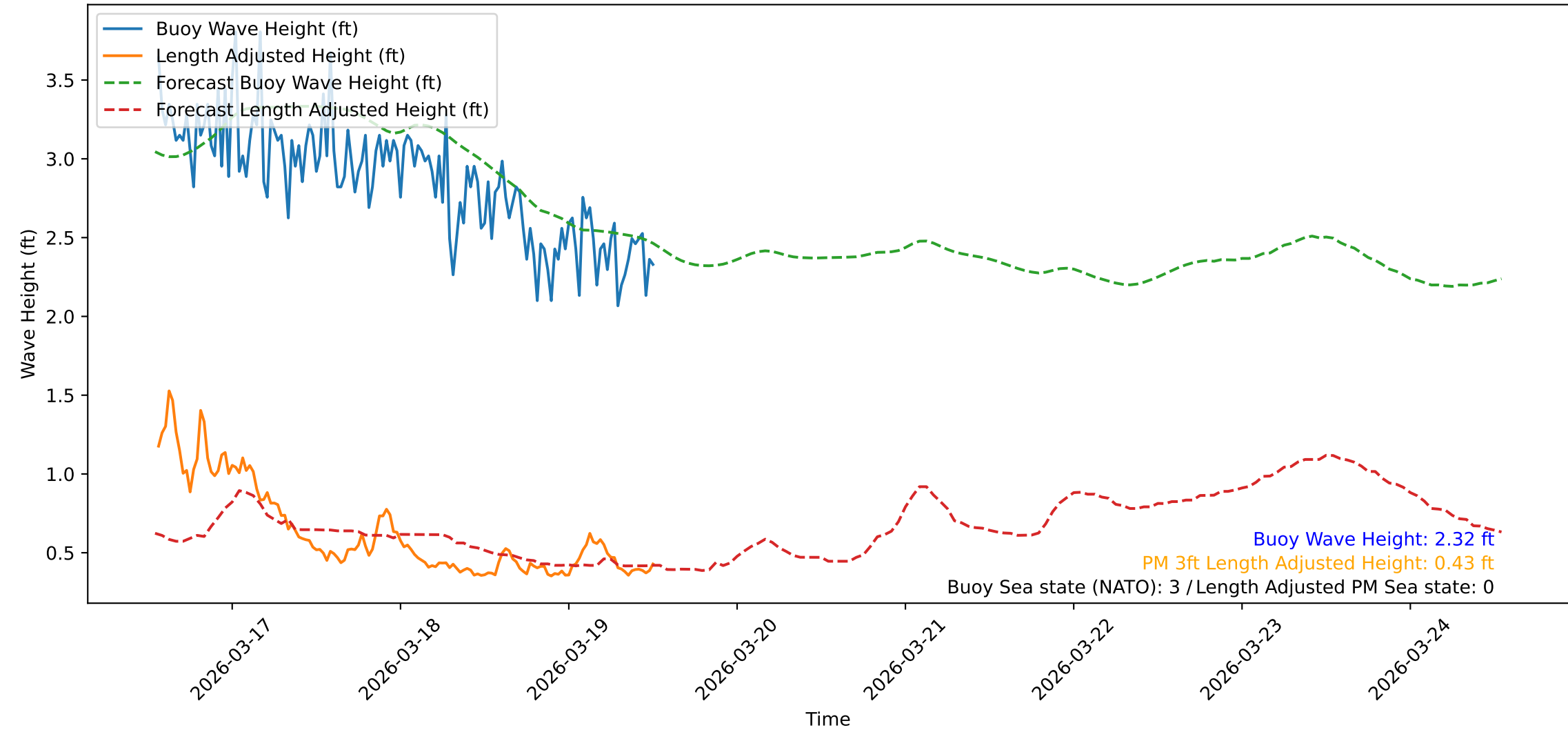
Wave Heights over Time for Red Beach at 2026-03-19 13:00:48
