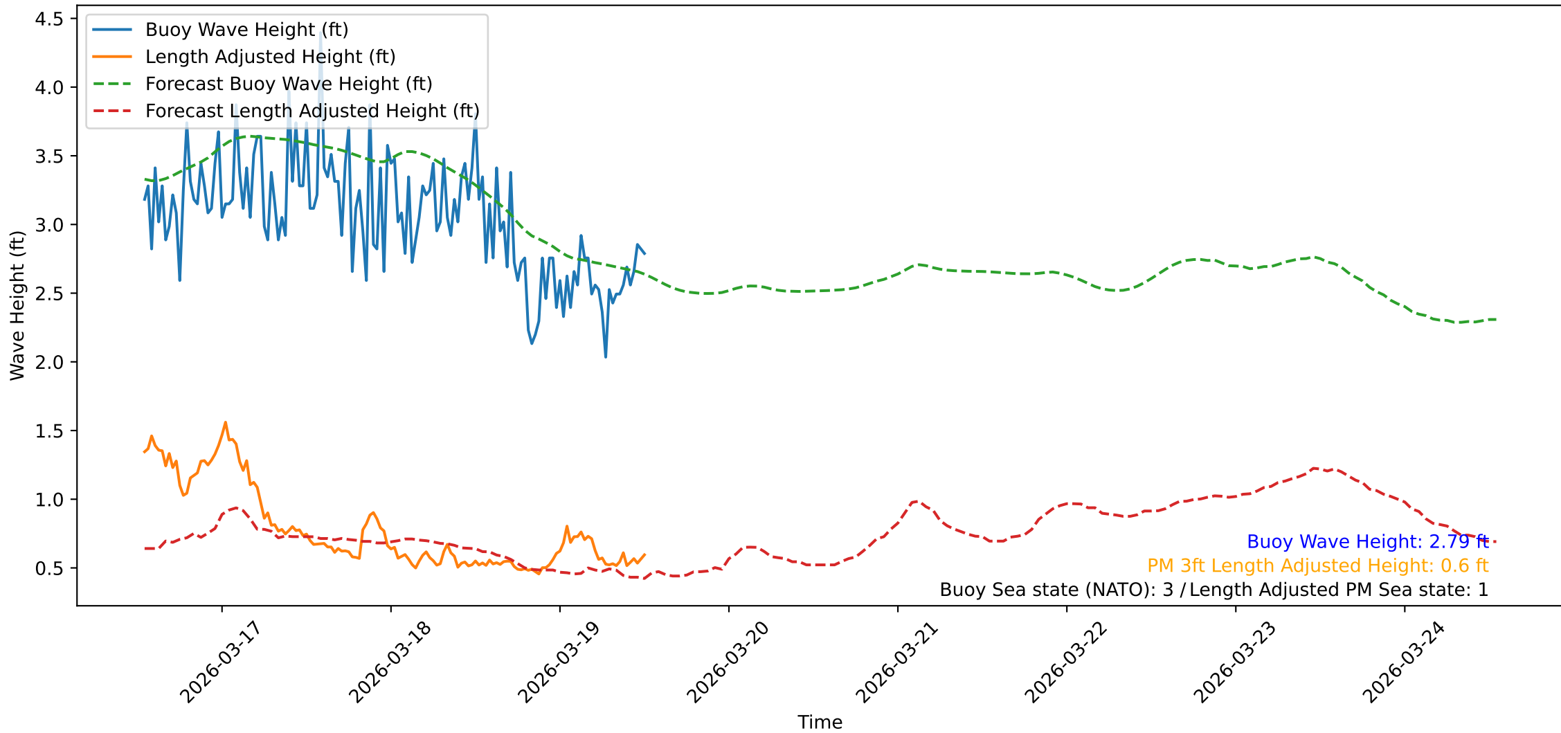
Wave Heights over Time for Oceanside Harbor at 2026-03-19 13:00:32
