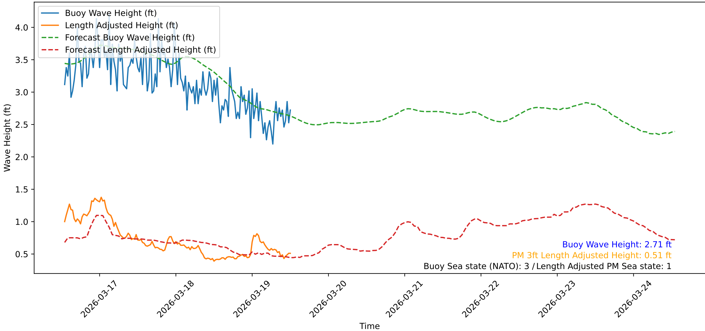
Wave Heights over Time for Green Beach at 2026-03-19 13:01:10
