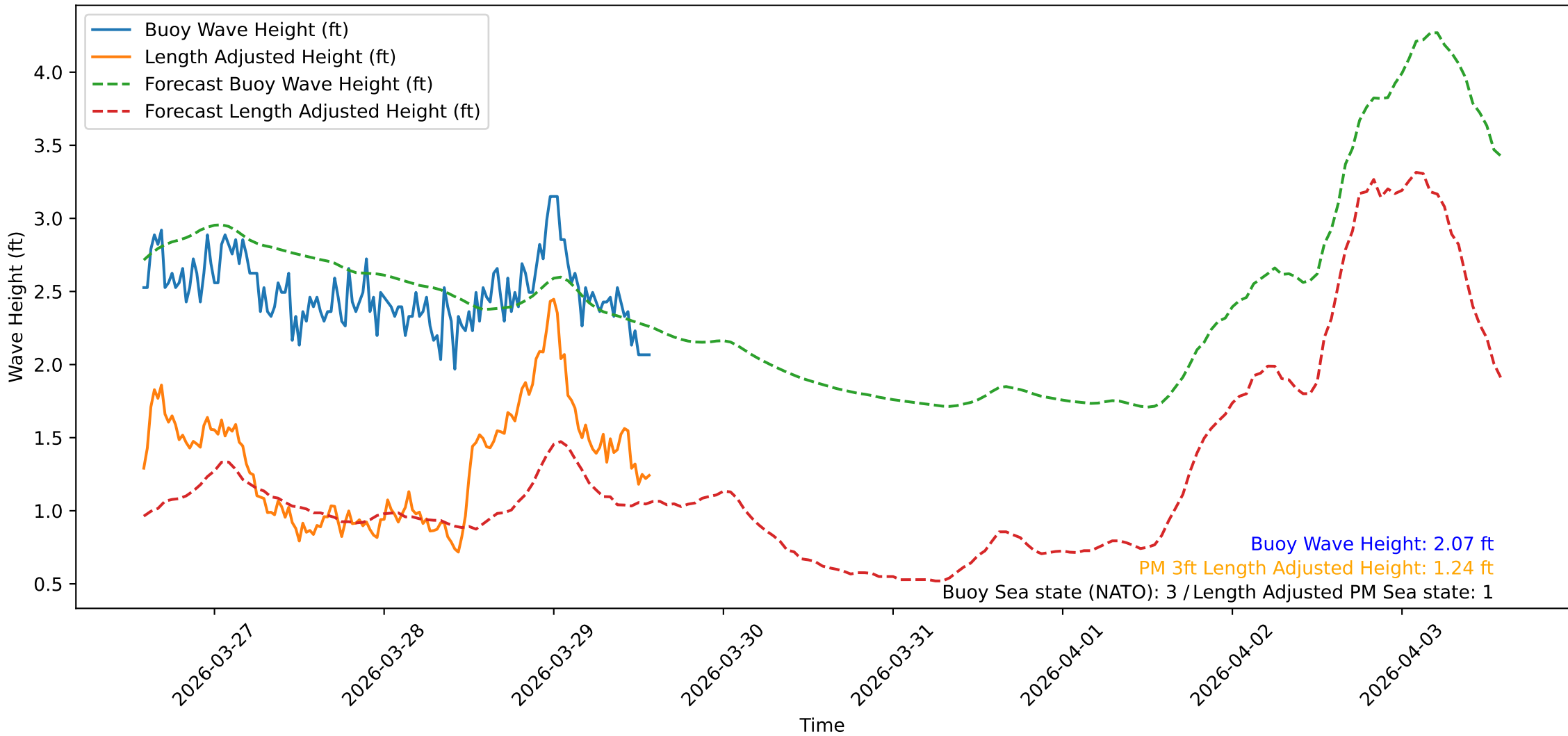
Wave Heights over Time for Oceanside Harbor at 2026-03-29 14:00:30
