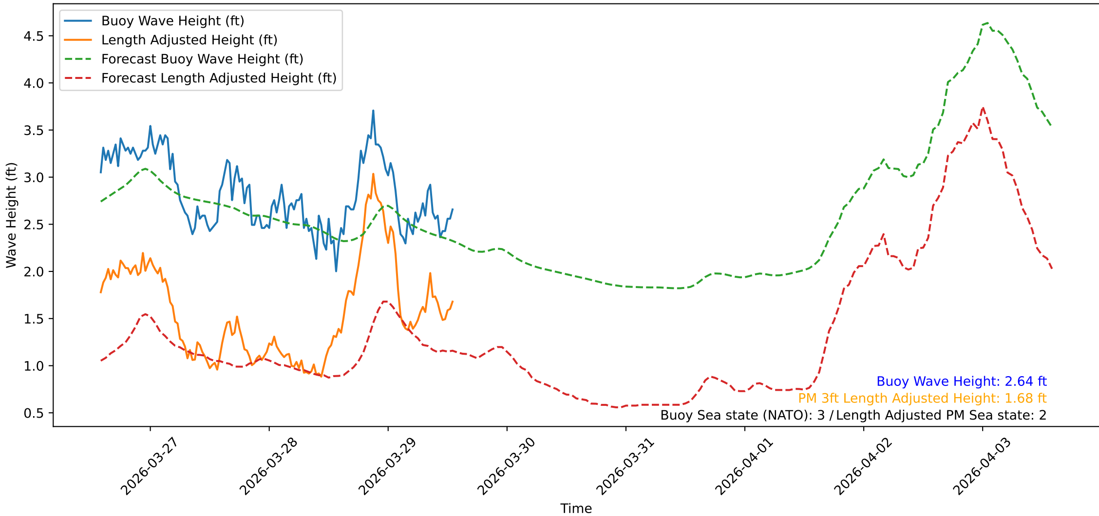
Wave Heights over Time for Green Beach at 2026-03-29 14:01:09
