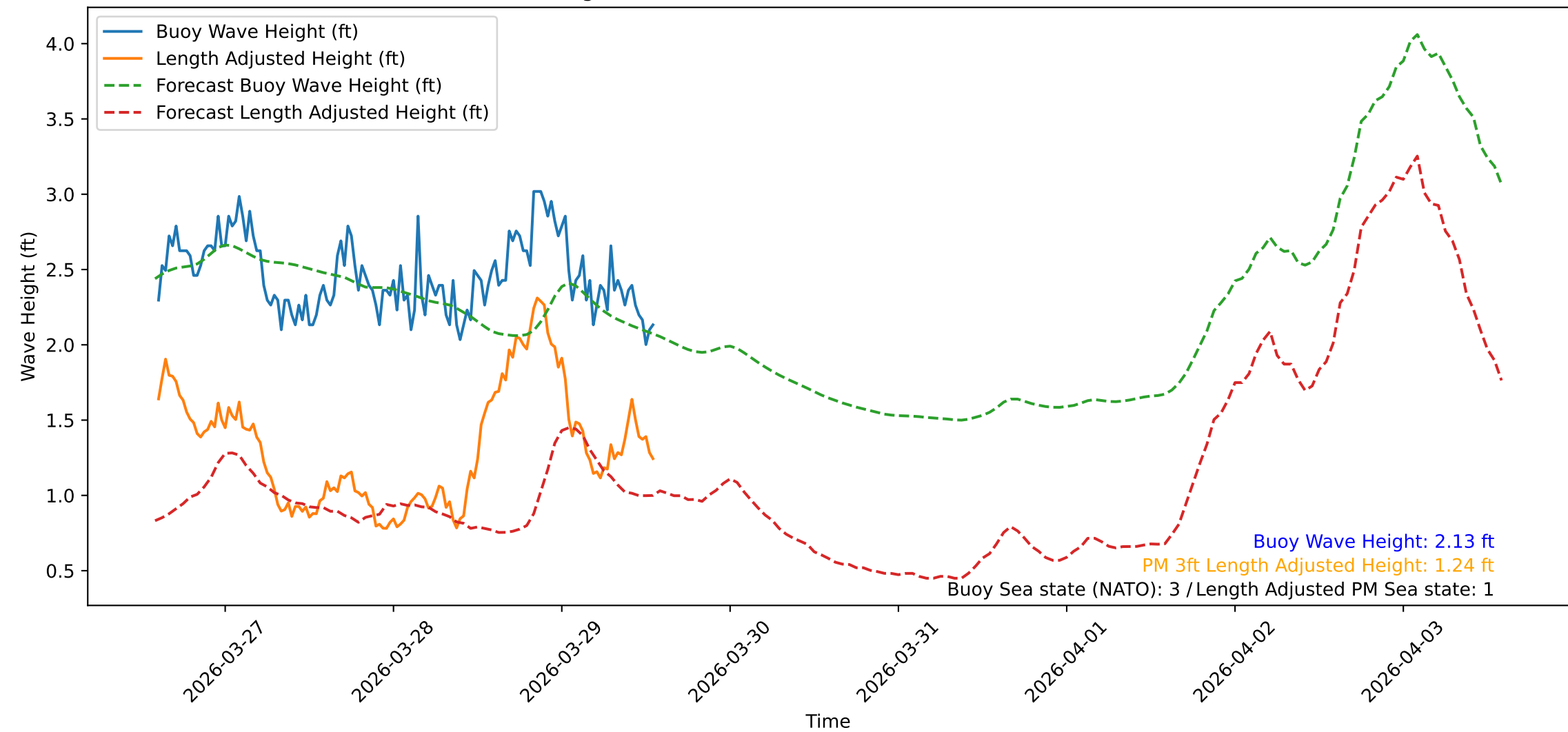
Wave Heights over Time for Red Beach at 2026-03-29 14:00:46
