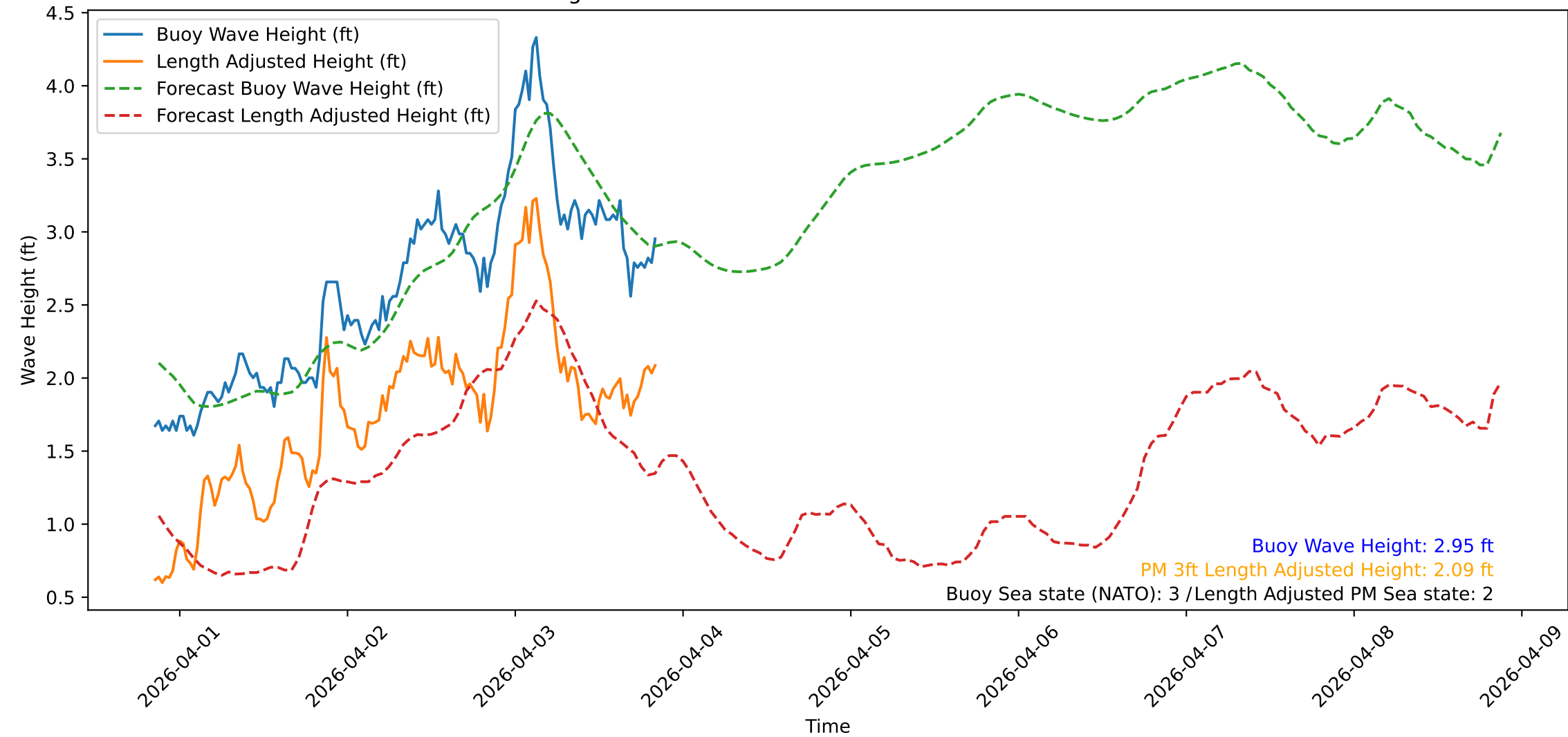
Wave Heights over Time for Green Beach at 2026-04-03 20:41:28
