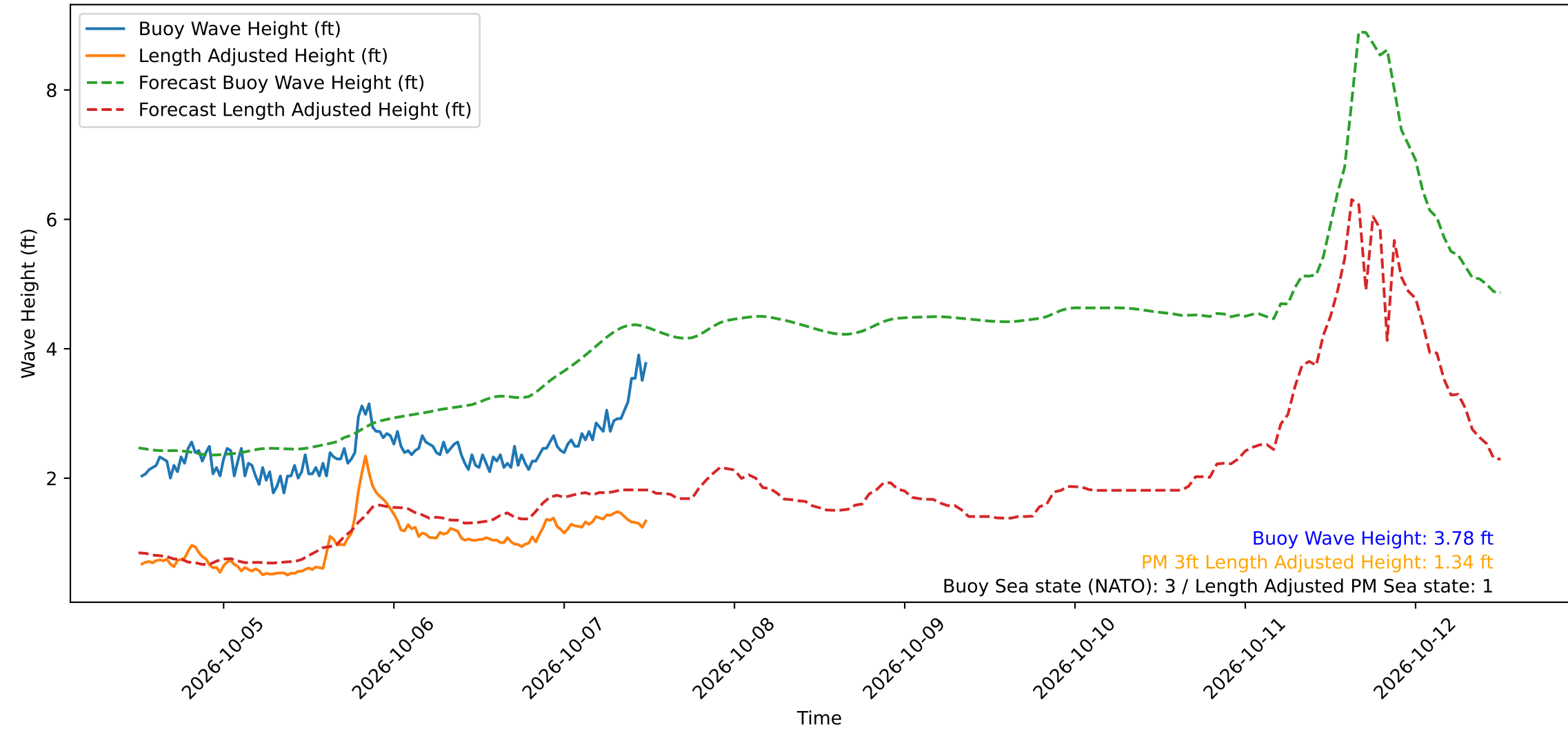
Wave Heights over Time for Green Beach at 2026-10-07 12:11:12
