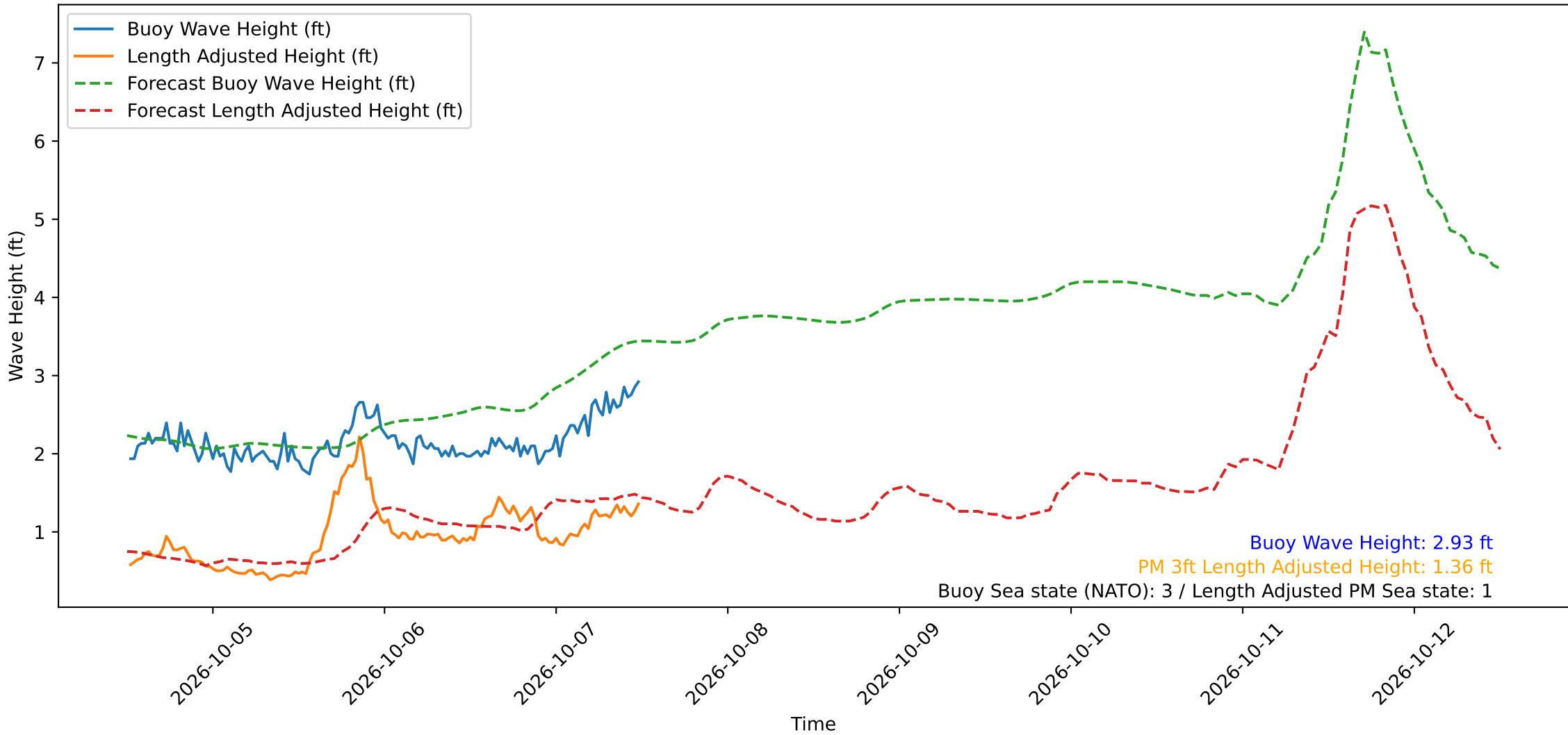
Wave Heights over Time for Red Beach at 2026-10-07 12:10:50
