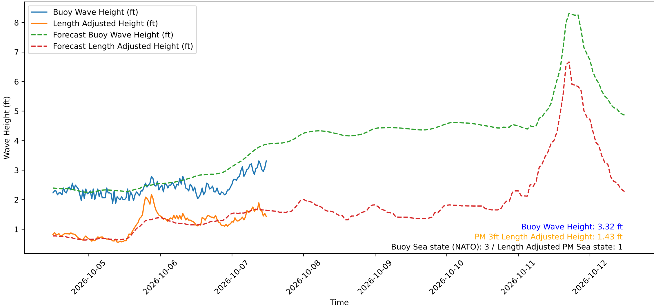
Wave Heights over Time for Oceanside Harbor at 2026-10-07 12:10:30
