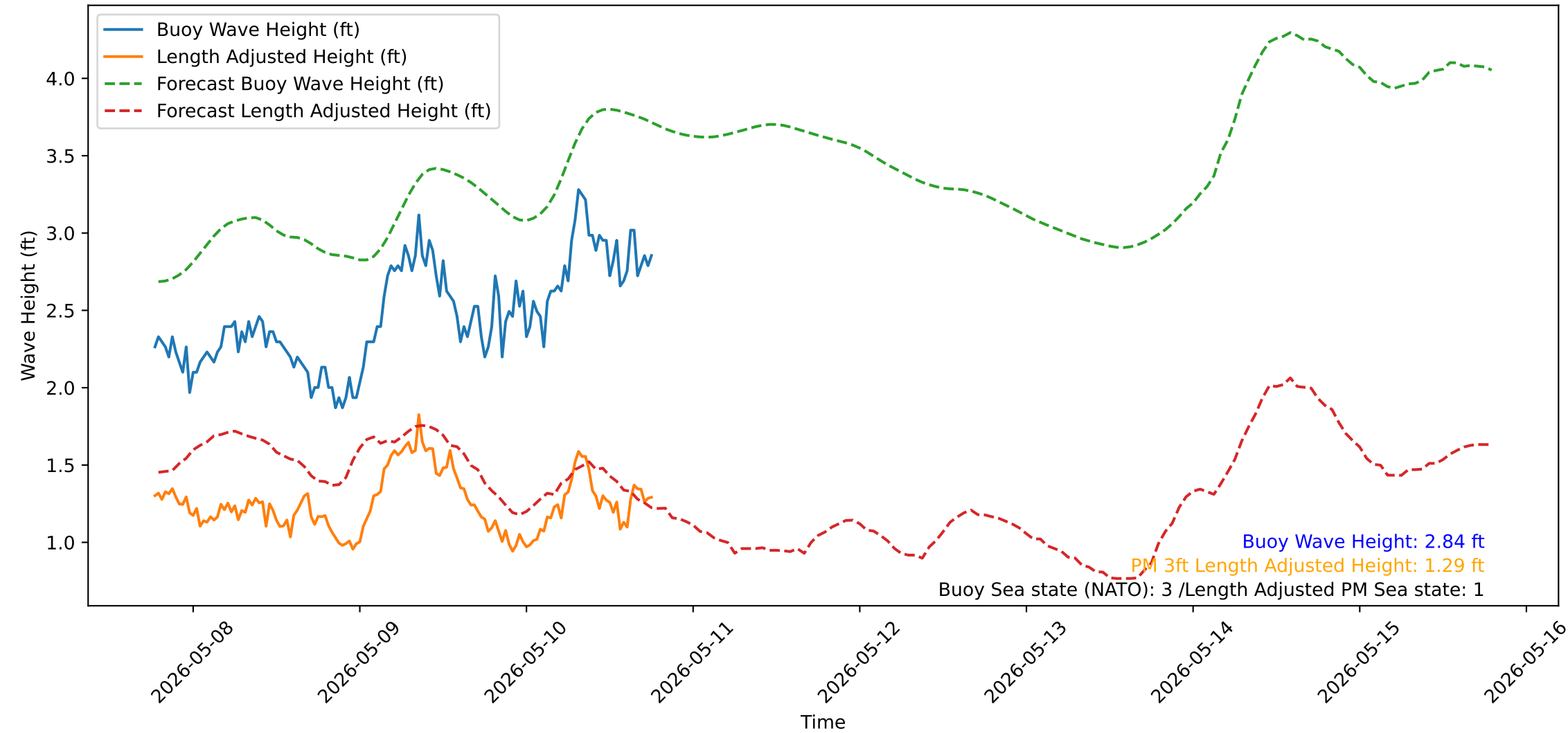
Wave Heights over Time for Oceanside Harbor at 2026-05-10 18:30:31
