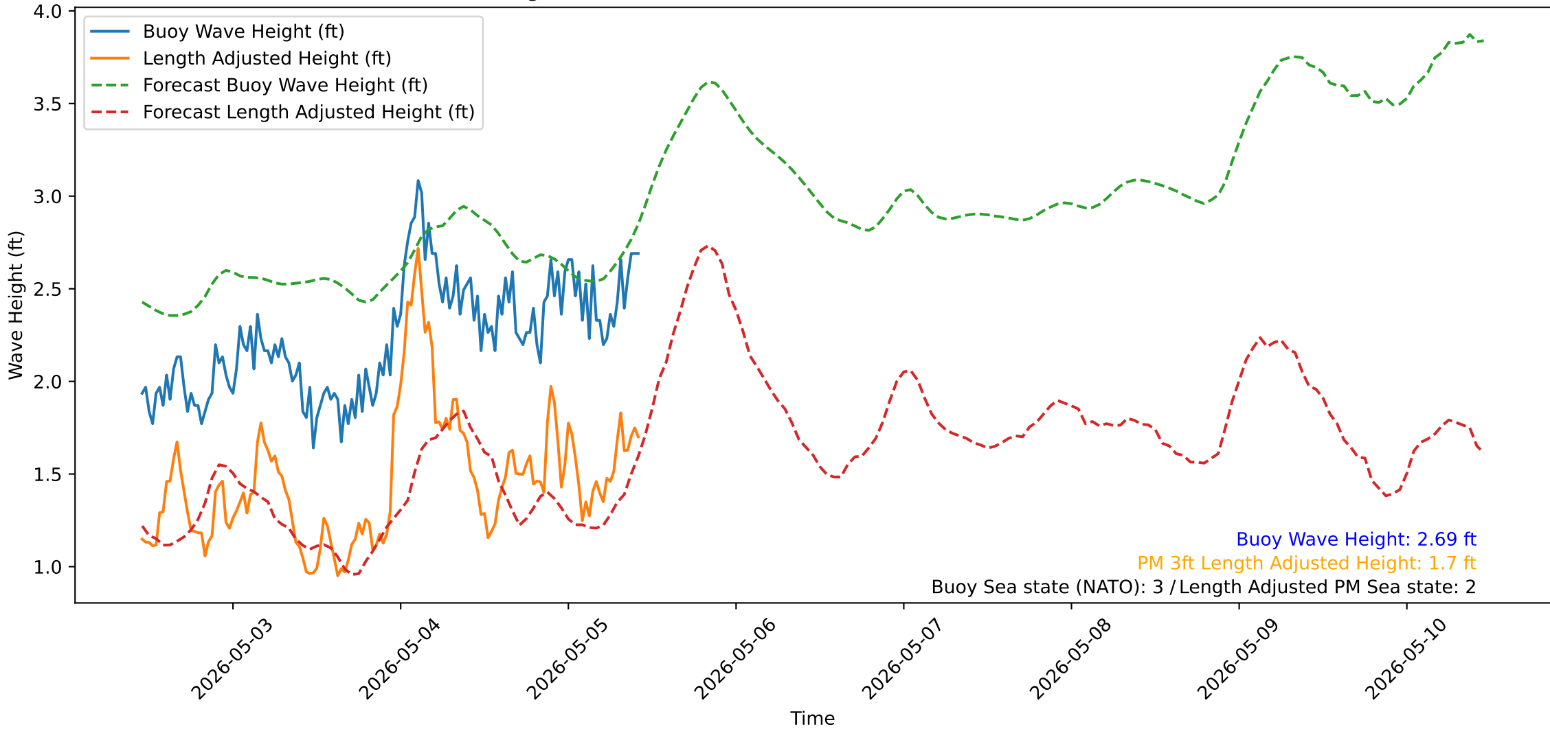
Wave Heights over Time for Oceanside Harbor at 2026-05-05 10:50:31
