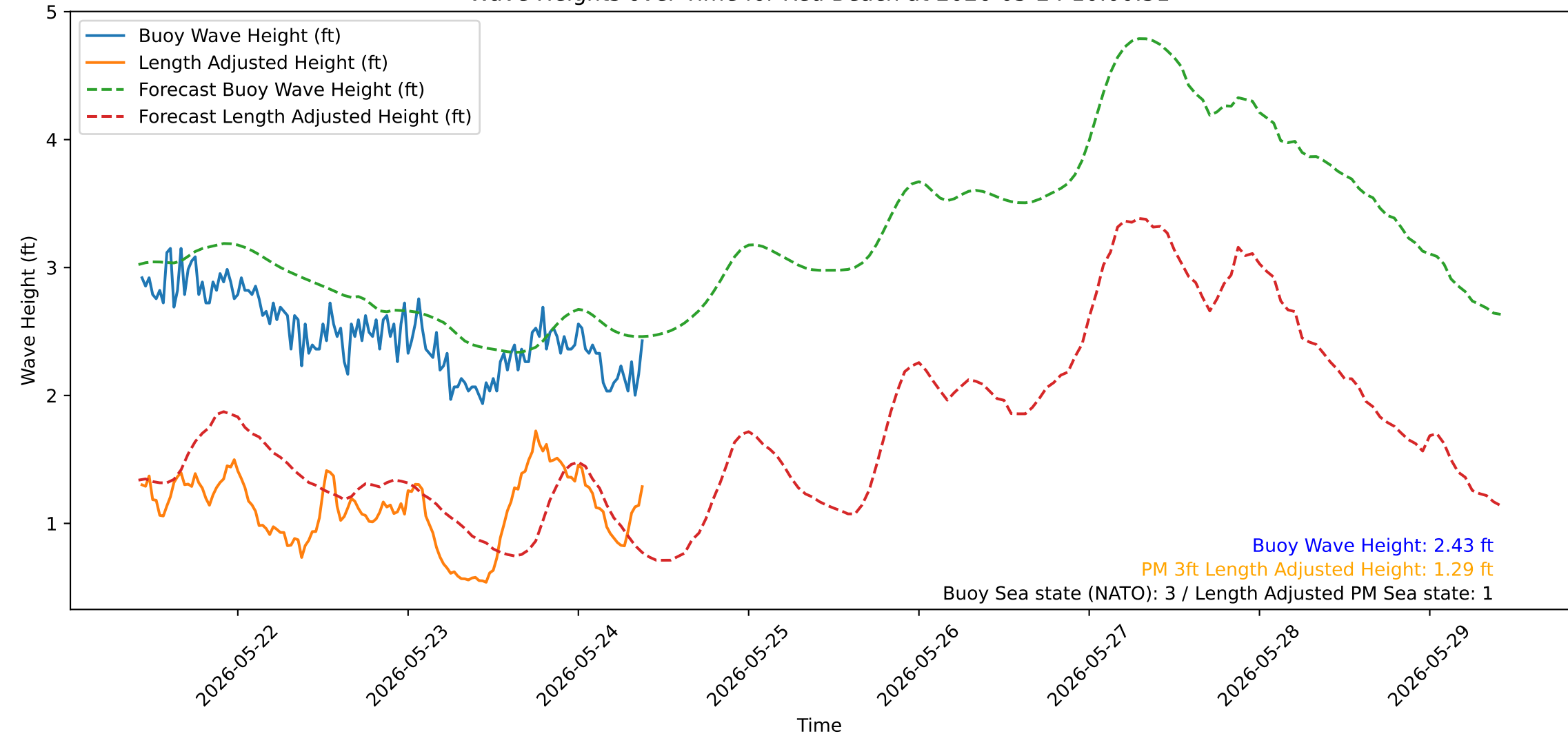
Wave Heights over Time for Red Beach at 2026-05-24 10:00:51
