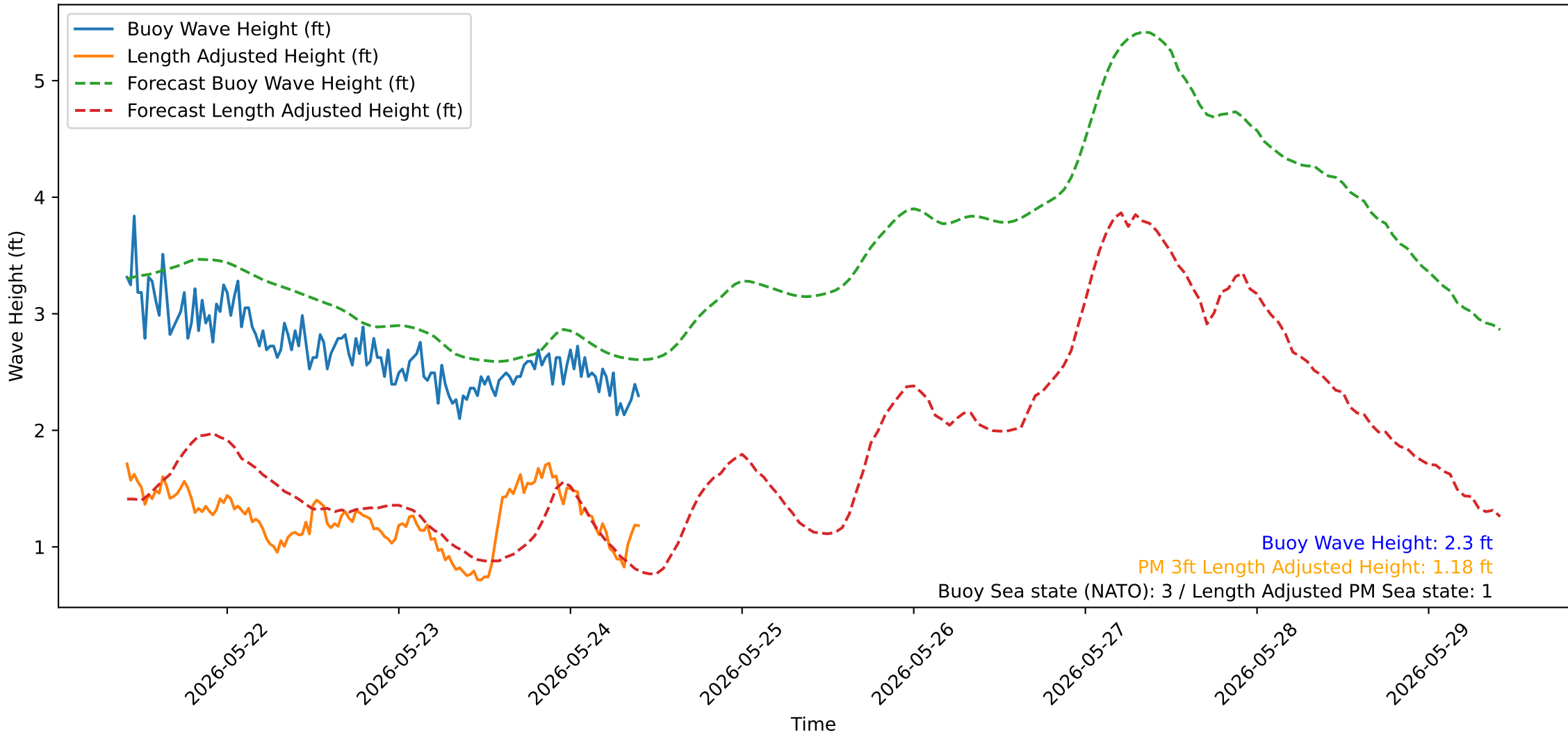
Wave Heights over Time for Oceanside Harbor at 2026-05-24 10:00:31
