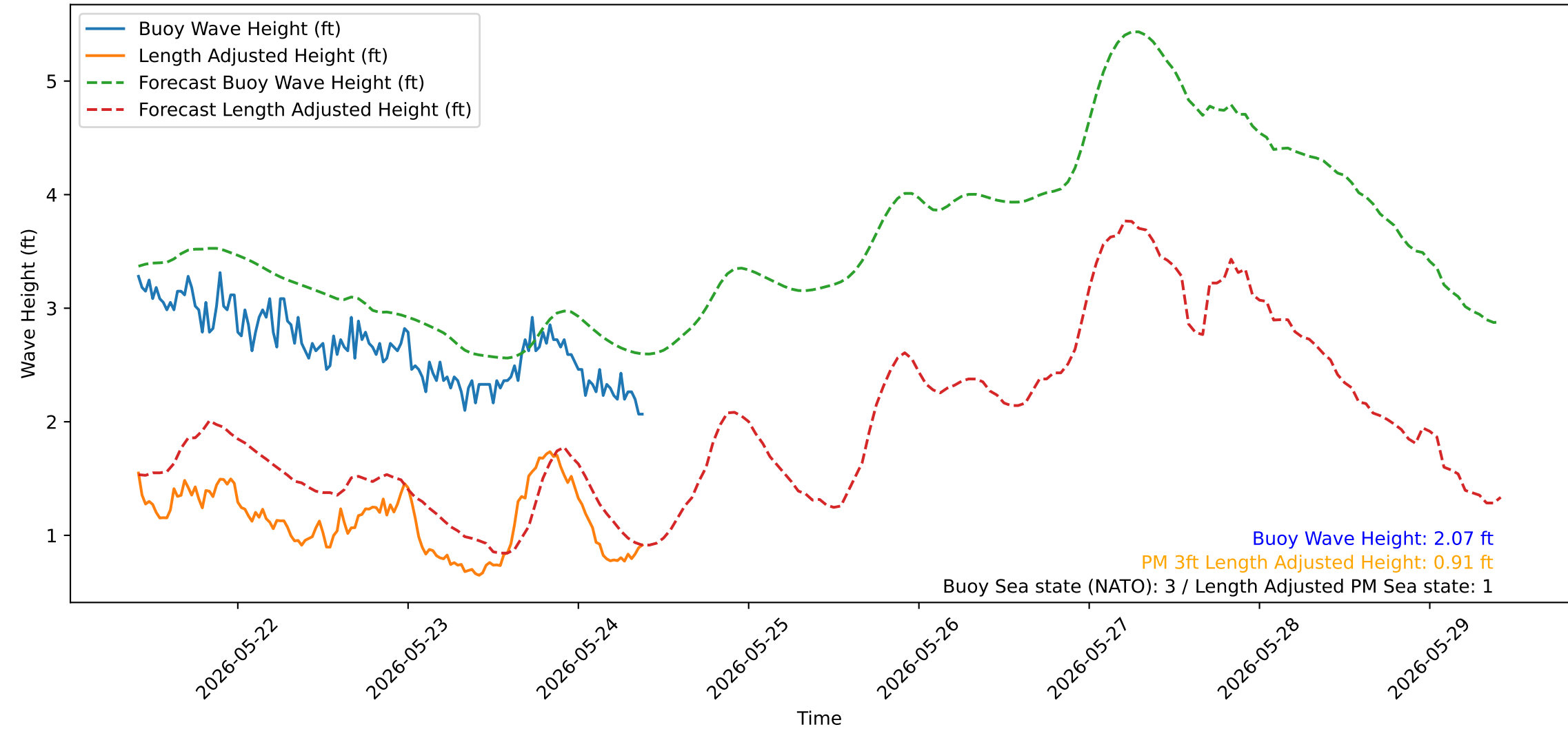
Wave Heights over Time for Green Beach at 2026-05-24 10:01:13
