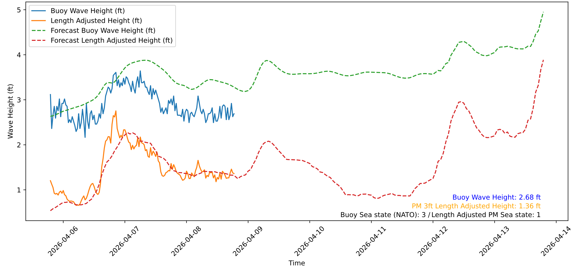
Wave Heights over Time for Oceanside Harbor at 2026-04-08 19:10:32
