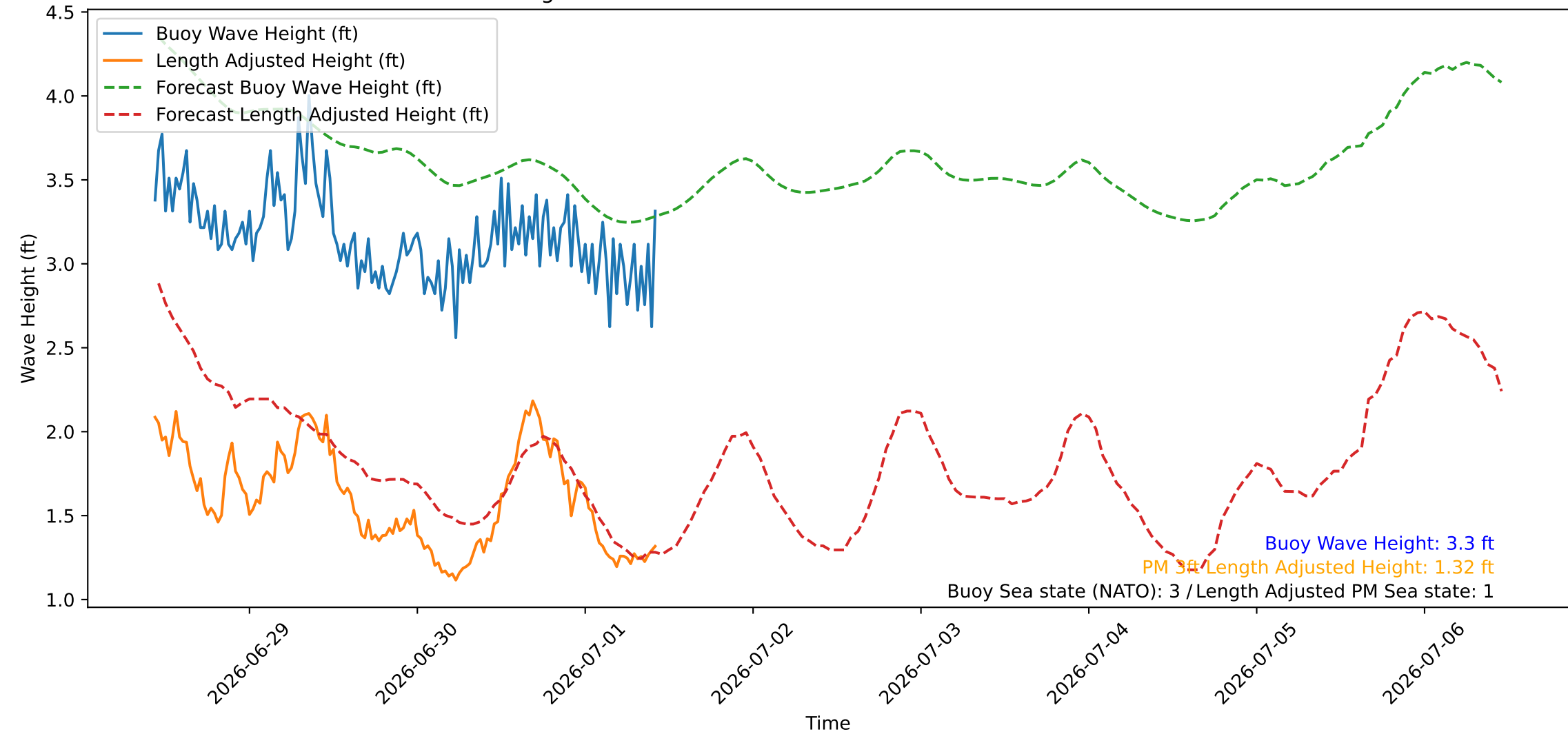
Wave Heights over Time for Oceanside Harbor at 2026-07-01 10:40:27
