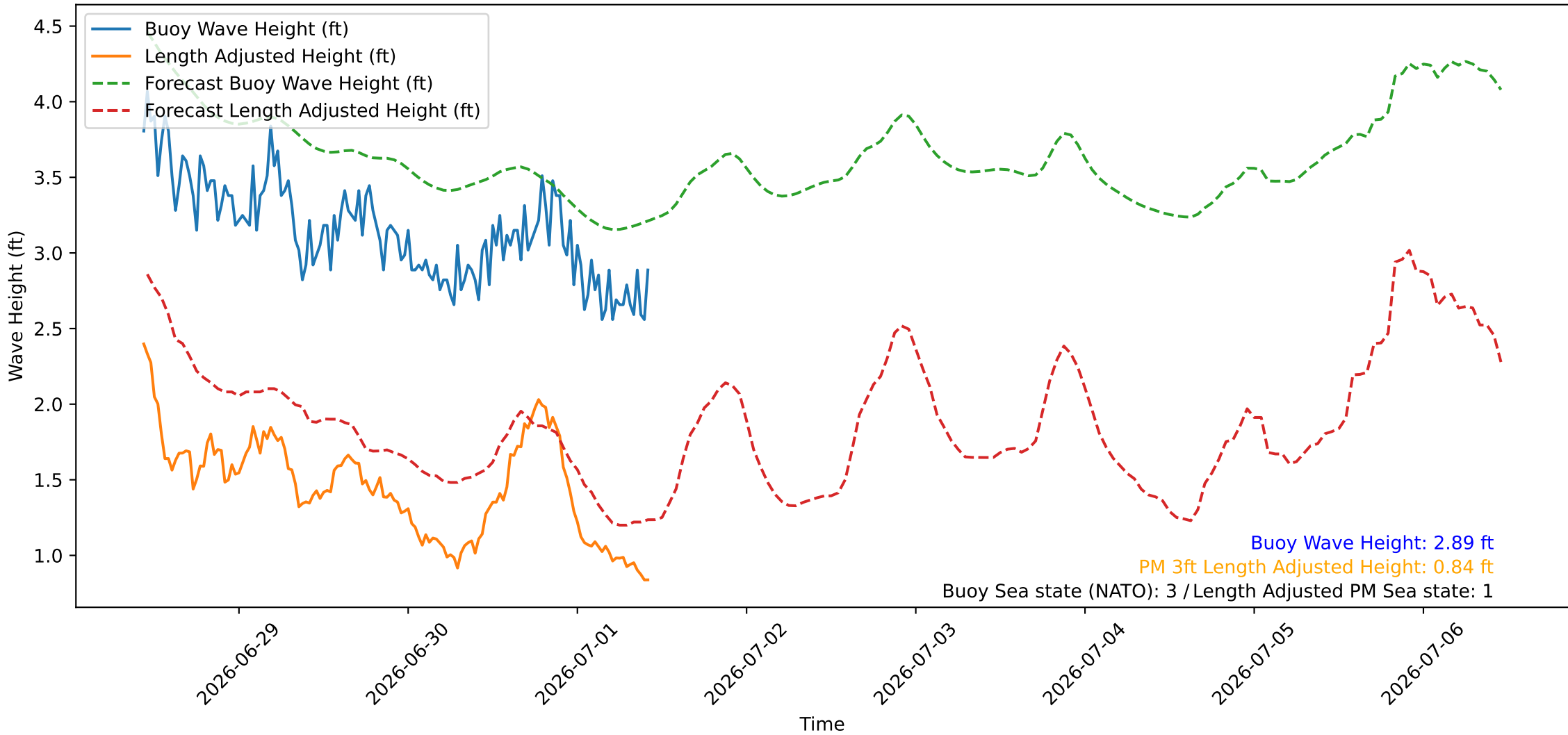
Wave Heights over Time for Green Beach at 2026-07-01 10:41:08
