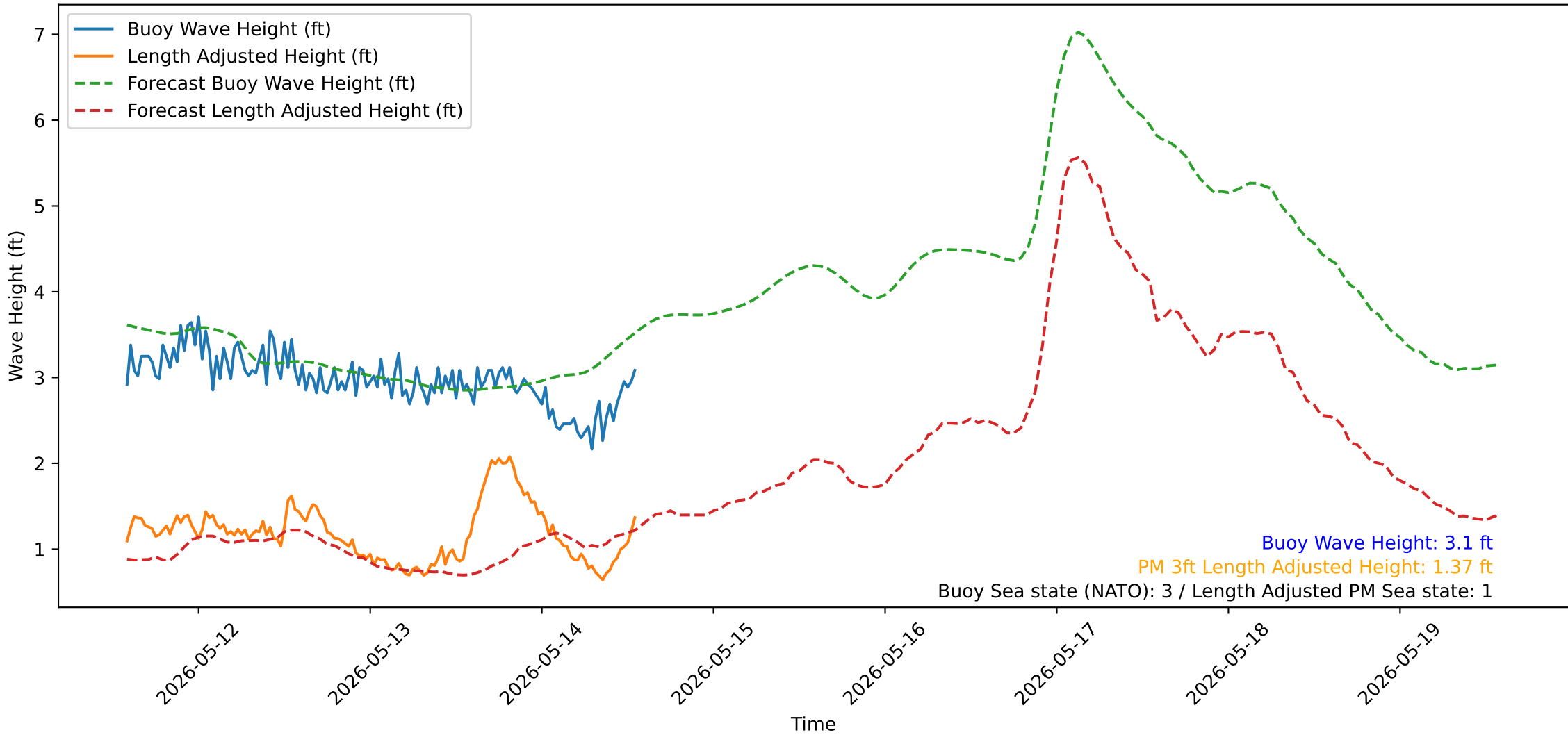
Wave Heights over Time for Oceanside Harbor at 2026-05-14 14:00:32
