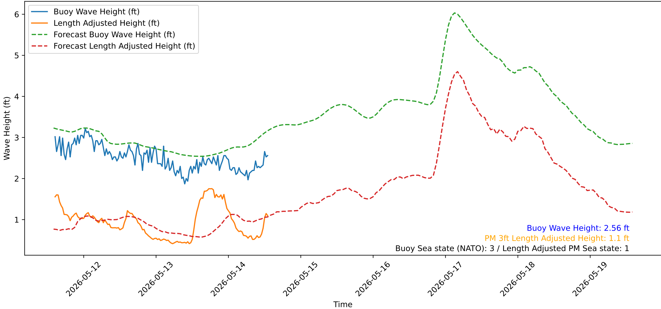
Wave Heights over Time for Red Beach at 2026-05-14 14:00:52
