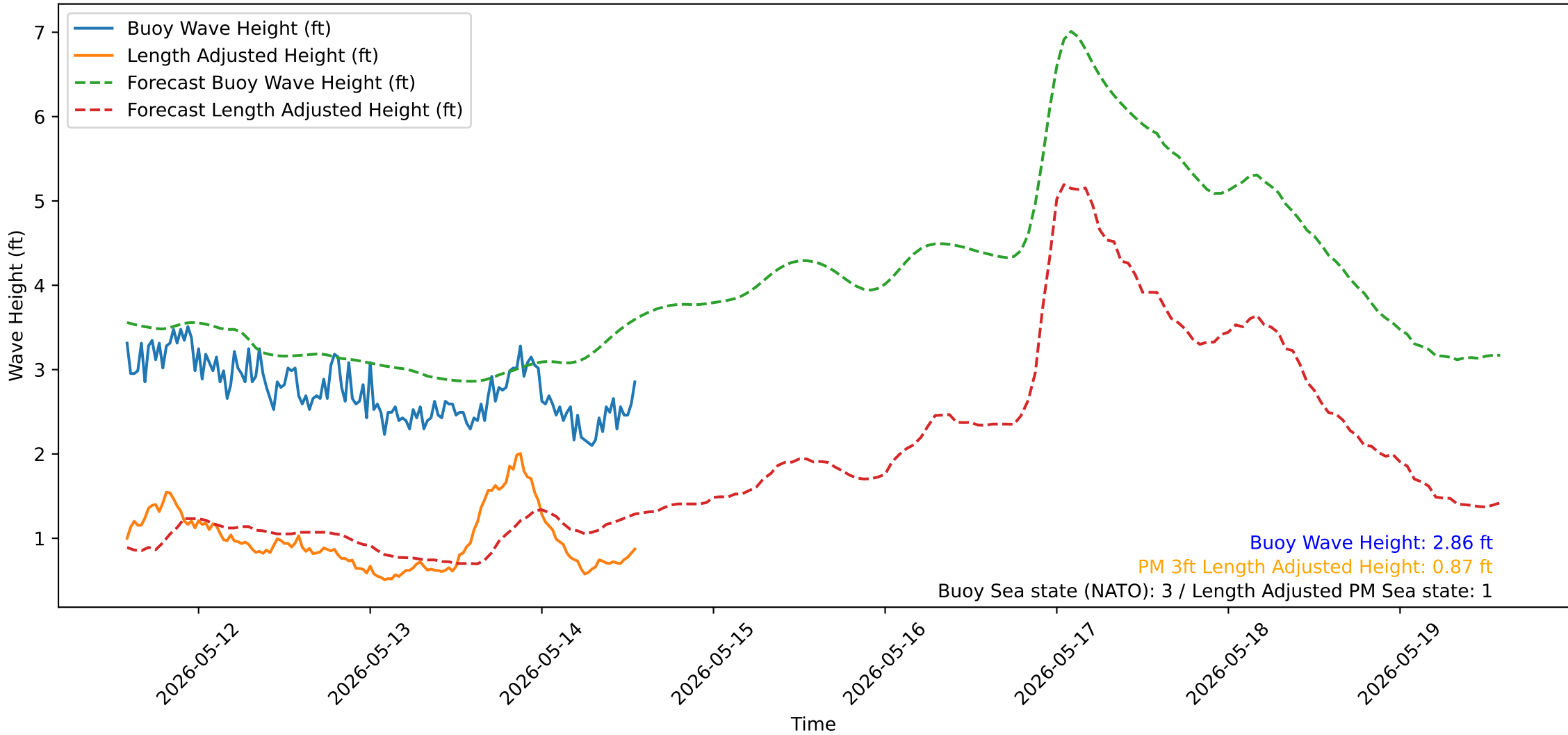
Wave Heights over Time for Green Beach at 2026-05-14 14:01:14
