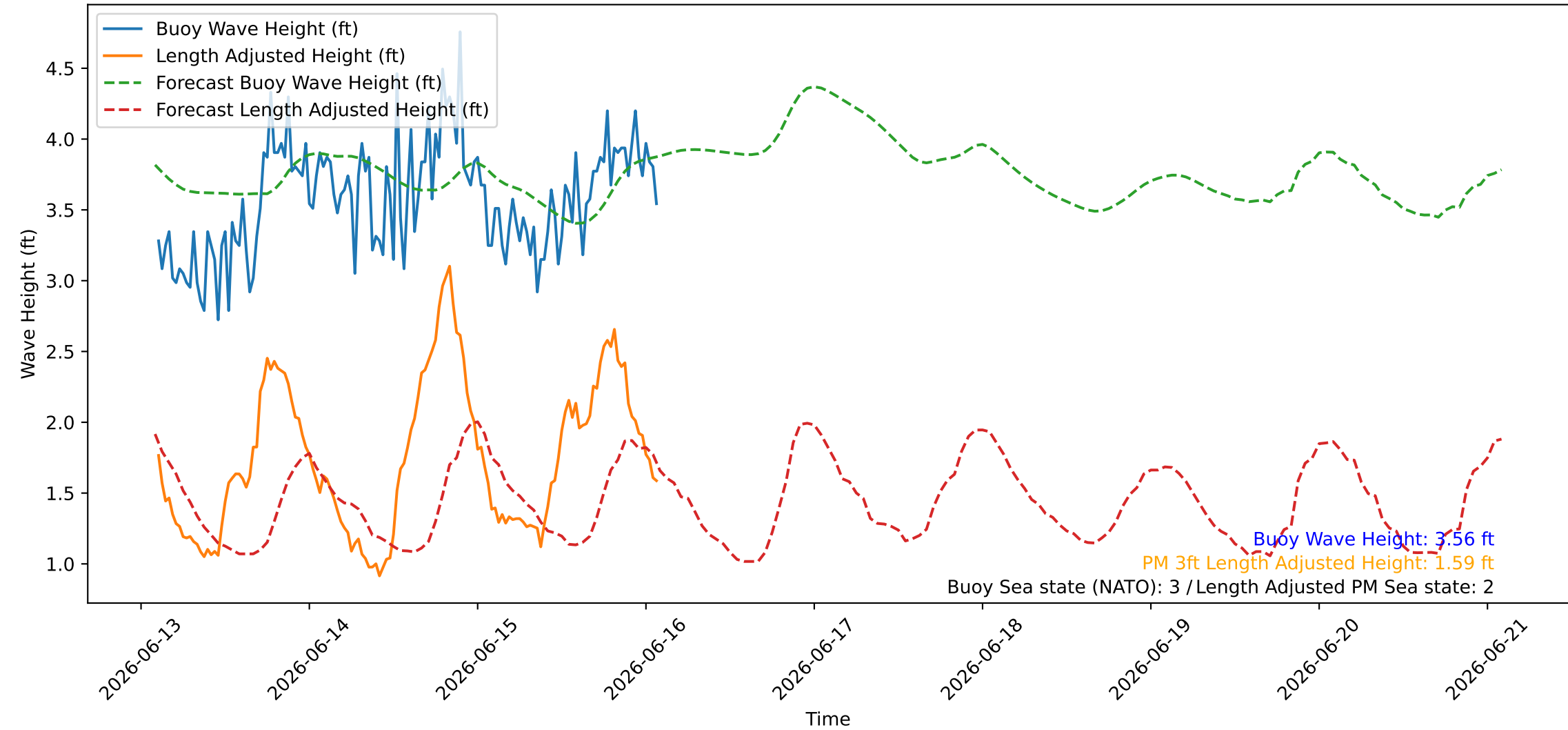
Wave Heights over Time for Red Beach at 2026-06-16 02:10:45
