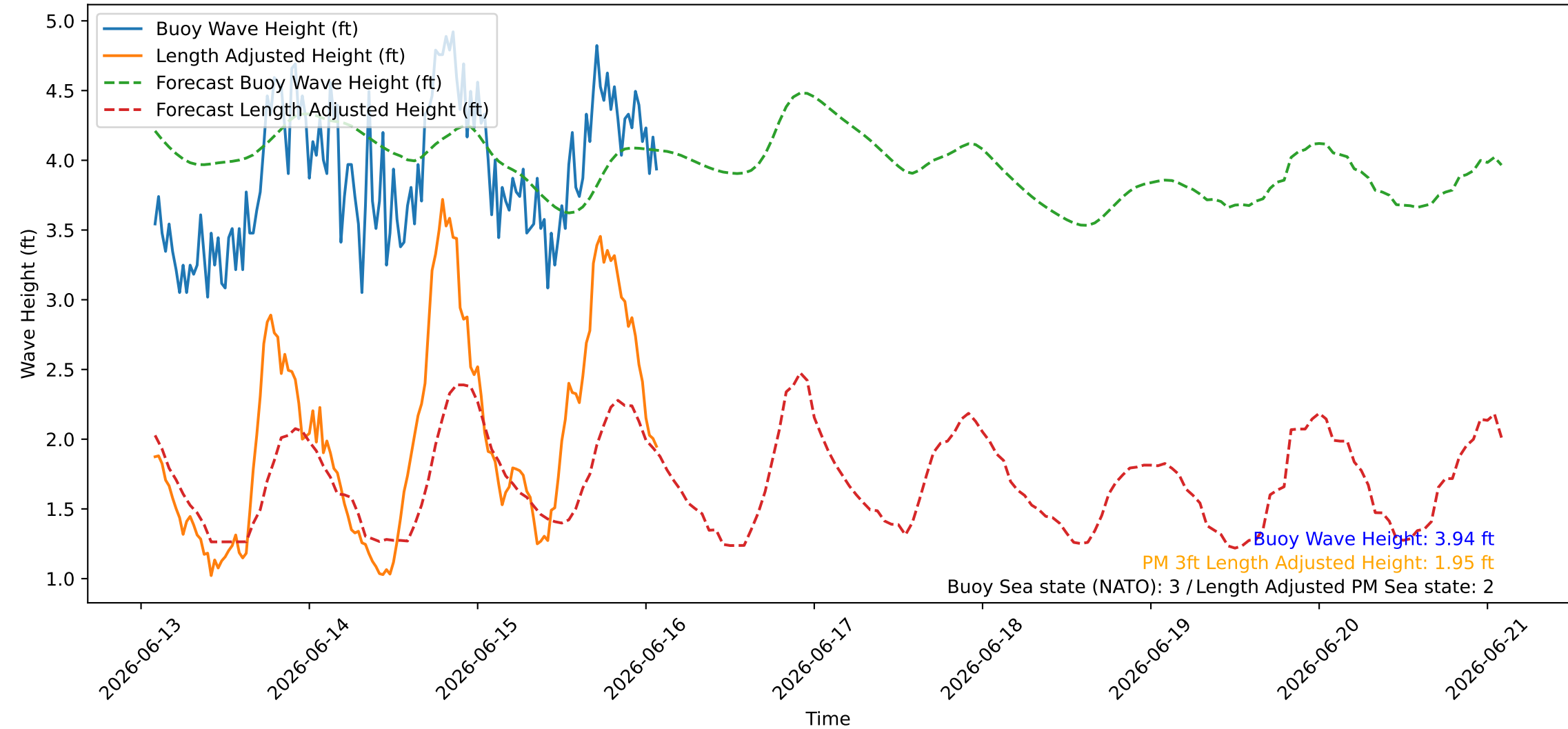
Wave Heights over Time for Green Beach at 2026-06-16 02:11:07
