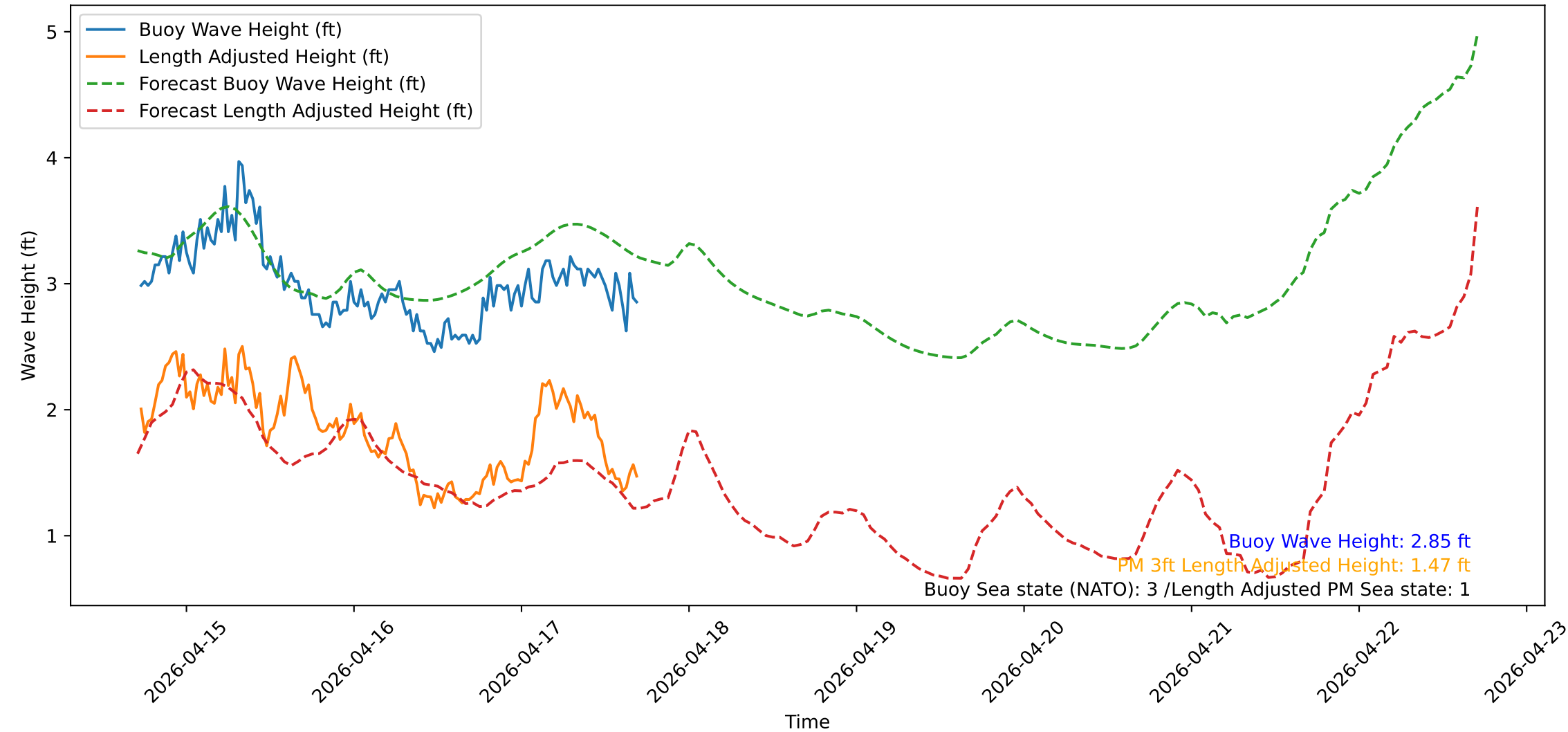
Wave Heights over Time for Green Beach at 2026-04-17 17:21:15
