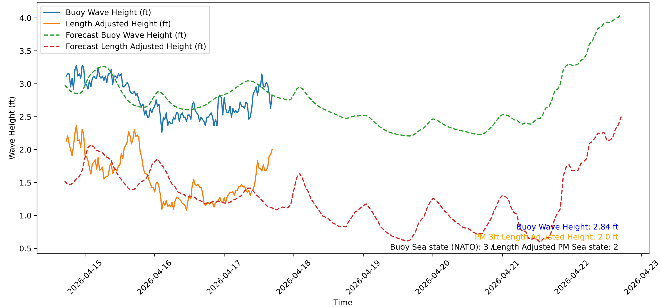
Wave Heights over Time for Red Beach at 2026-04-17 17:20:51
