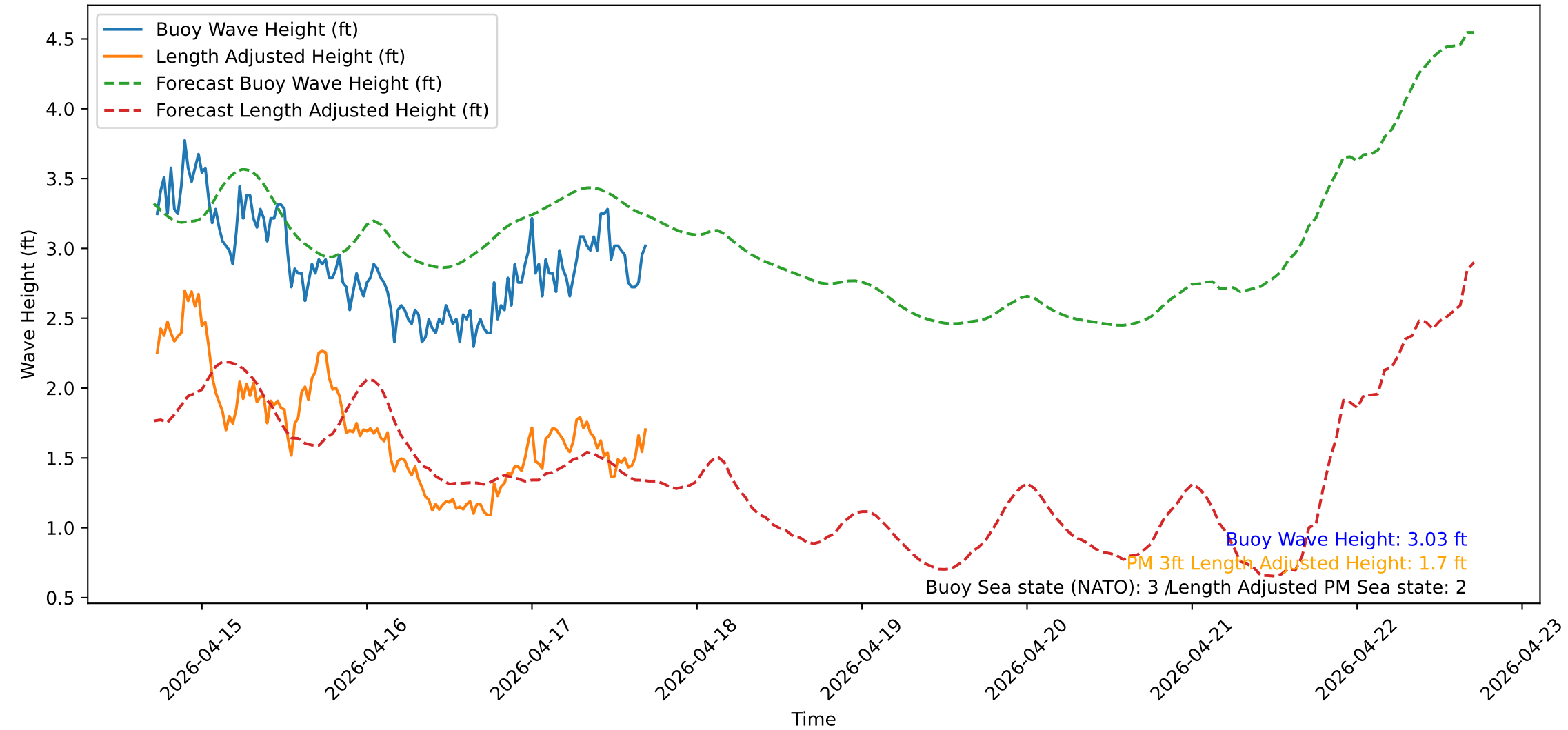
Wave Heights over Time for Oceanside Harbor at 2026-04-17 17:20:31
